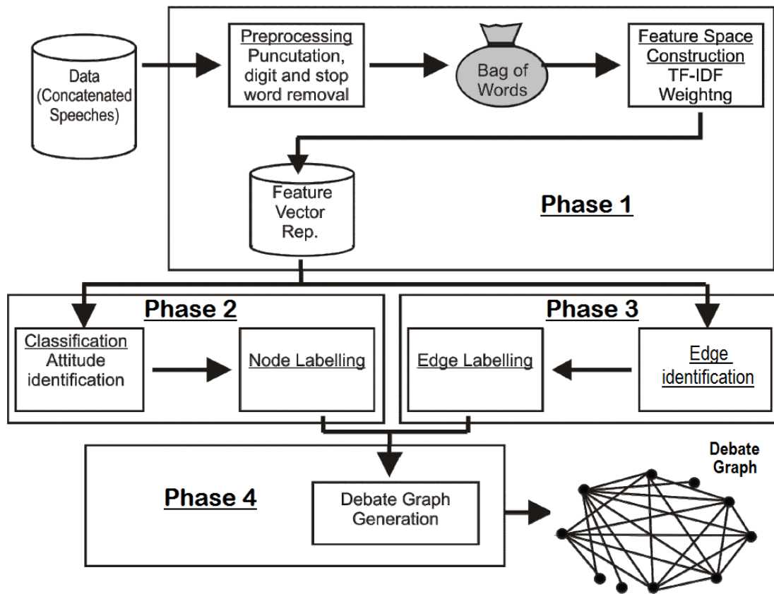
Figure 8.2: The Debate Graph Extraction (DGE) framework using the classification-based approach for attitude prediction.
