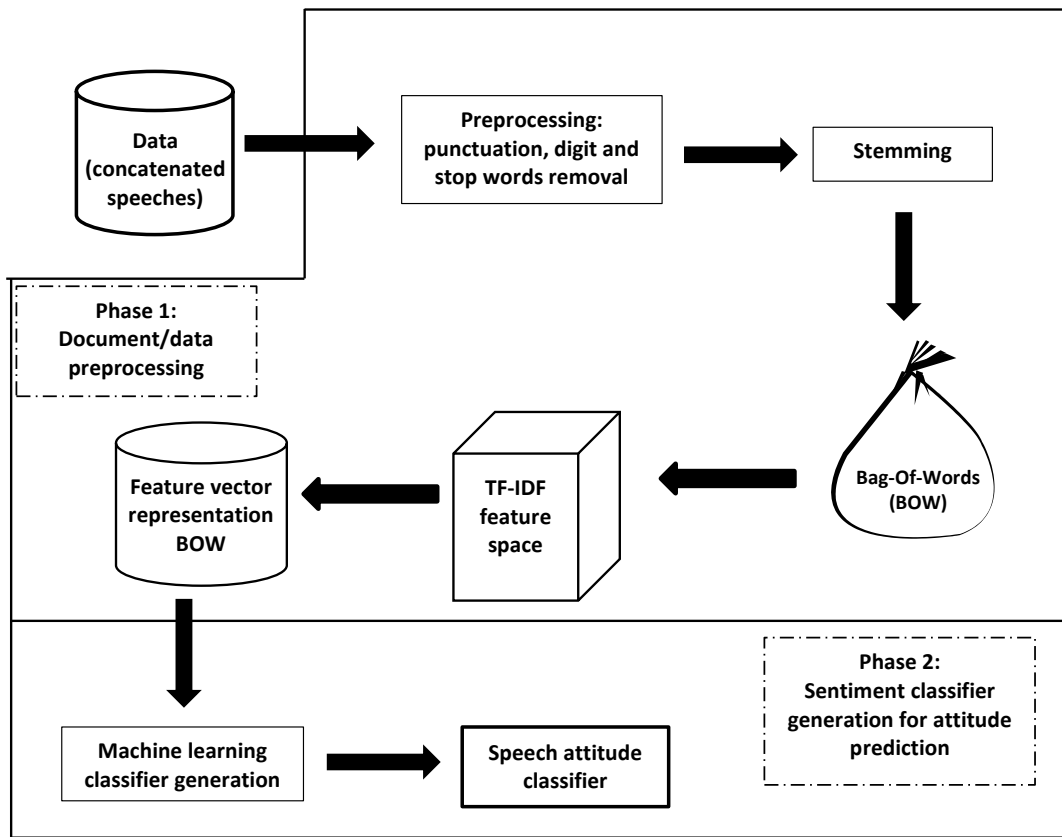
Figure 4.1: The classification-based approach to sentiment mining (classifier generation).
