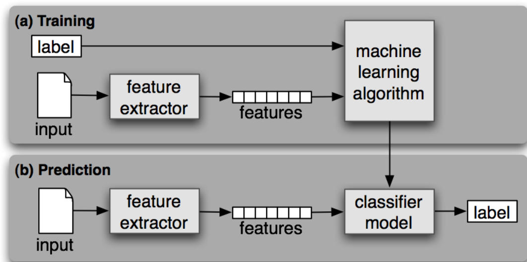
Figure 2.1: Training and testing a machine learning classifier.
