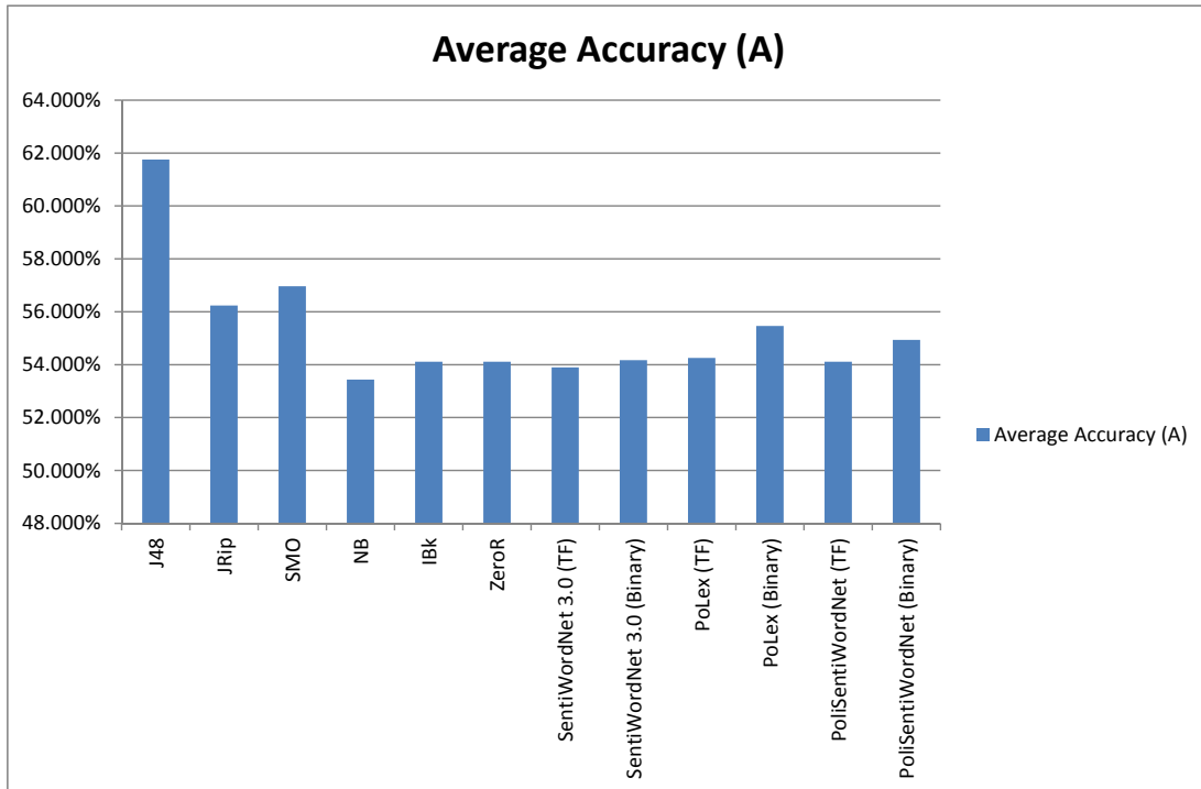
Figure 7.1: Bar chart representation for the recorded Average Accuracy (A) values presented in Table 7.1.
