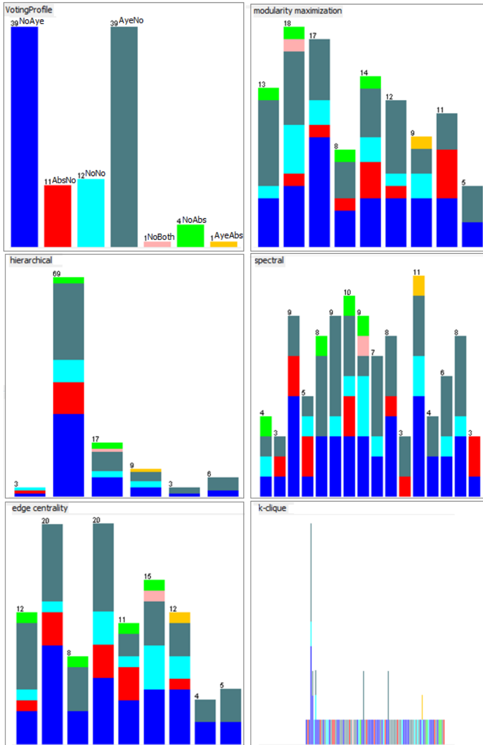
Figure 9.12: Communities in the interruption network for the Syria debate. The top left histogram presents the known communities, according to voting profile, while the rest of histograms present the predicted communities using modularity maximization, hierarchical and spectral clustering, edge centrality and k-Clique percolation algorithms. The colour coding is defined in the top left histogram.
