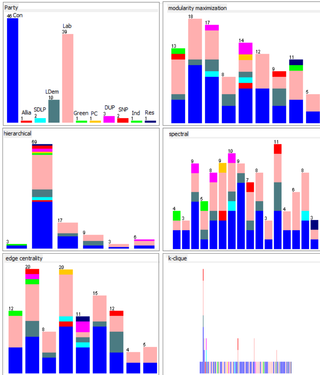
Figure 9.16: Communities in the interruption network for the Syria debate. The top left histogram presents the known communities (according to party affiliation) while the rest of histograms present the detected communities (clusters predicted using modularity maximization, hierarchical and spectral clustering, edge centrality and k-Clique percolation algorithms). The colour coding is defined in the top left histogram.
