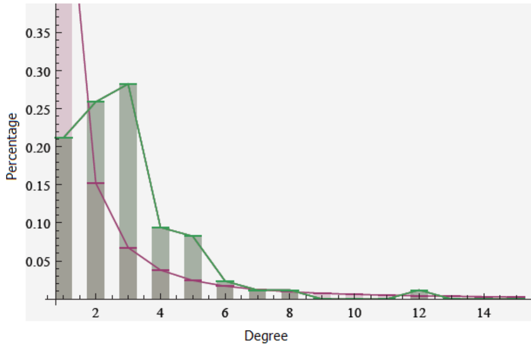
Figure 9.8: The power-law degree distributions for the Syria debate interruption network (top) and relevant interruption network (bottom). Each bar indicates the fraction of nodes (vertical axis) with respect to a given degree (horizontal axis). The degree distributions of both networks follow approximate power-law form indicated by the green curves, while the magenta curves indicate Zipfian distributions with the same range.
