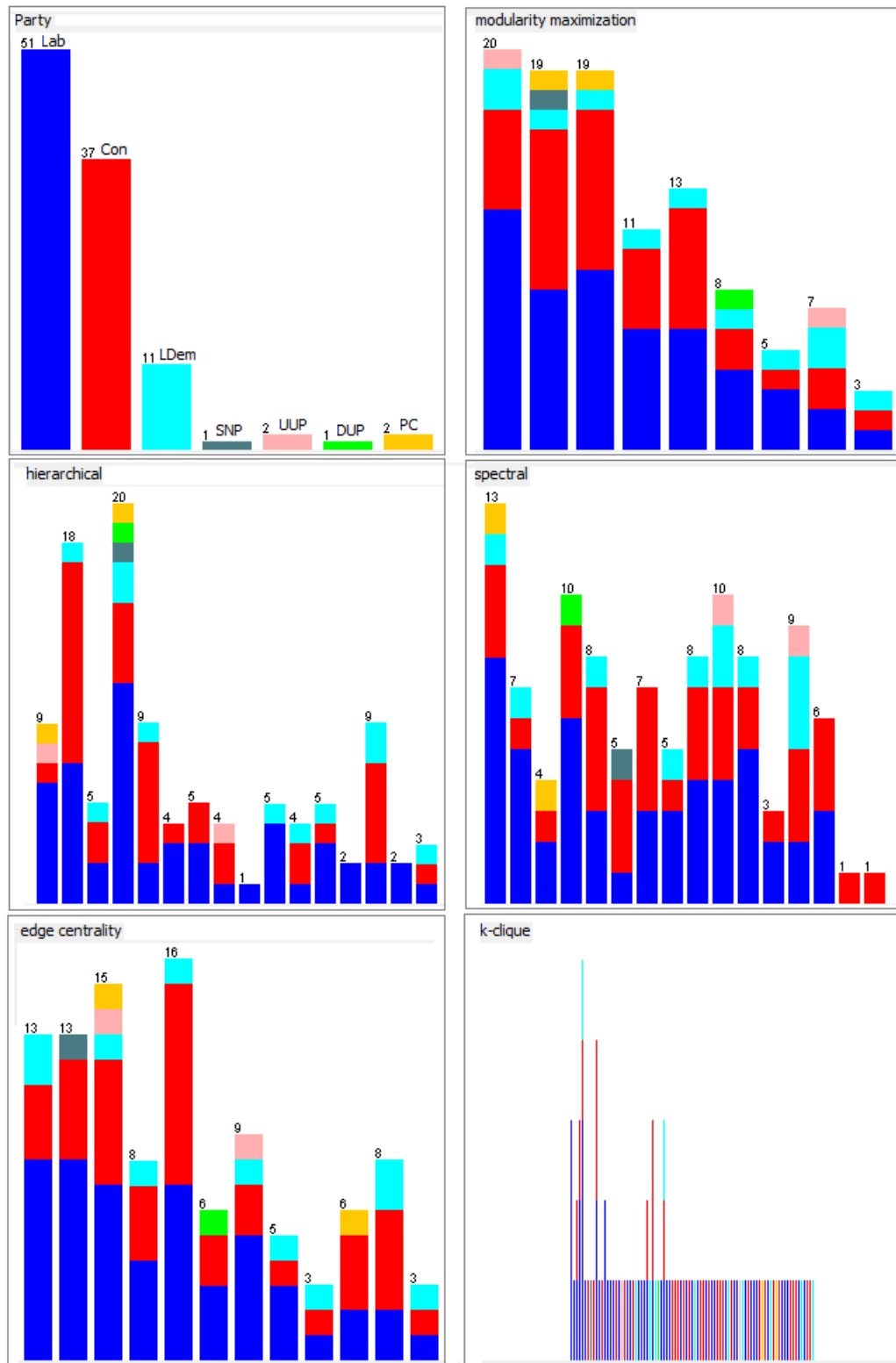
Figure 9.14: Communities in the interruption network for the Iraq debate. The top left histogram presents the known communities (according to party affiliation) while the rest of histograms present the detected communities (clusters predicted using modularity maximization, hierarchical and spectral clustering, edge centrality and k-Clique percolation algorithms). The colour coding is defined in the top left histogram.
