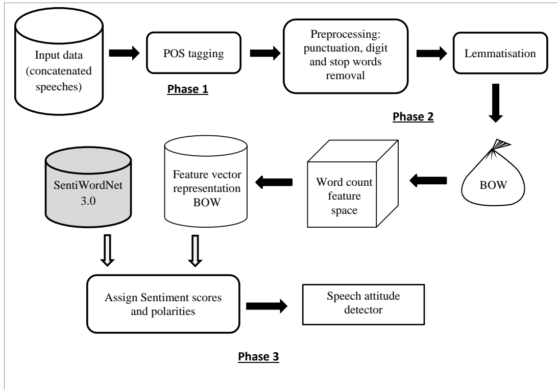
Figure 5.1: The generic sentiment lexicon-based approach to sentiment mining.
