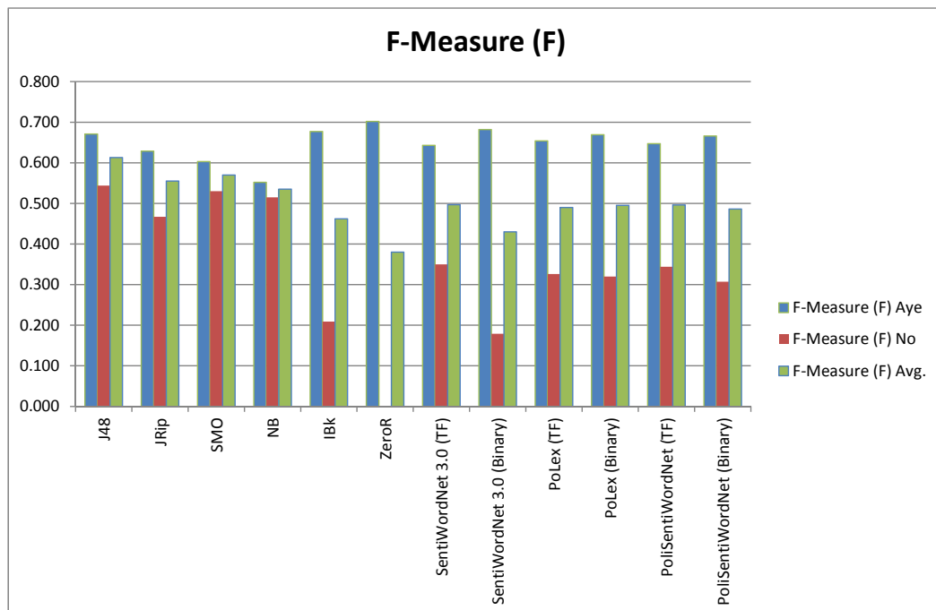
Figure 7.2: Bar chart representation for the recorded F-Measure (F) values presented in Table 7.1.
