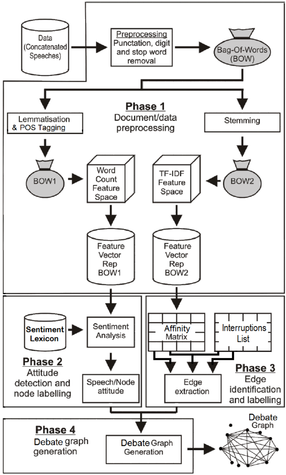
Figure 8.1: The Debate Graph Extraction (DGE) framework using the sentiment lexicon-based approach for attitude identification.
