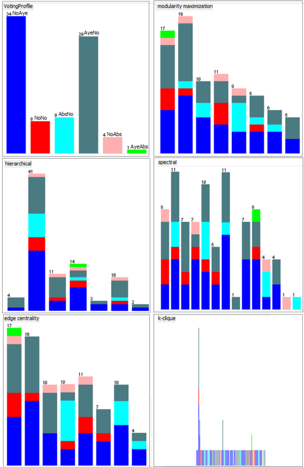
Figure 9.13: Communities in the relevant interruption network for the Syria debate. The top left histogram presents the known communities, according to voting profile, while the rest of histograms present the predicted communities using modularity maximization, hierarchical and spectral clustering, edge centrality and k-Clique percolation algorithms. The colour coding is defined in the top left histogram.
