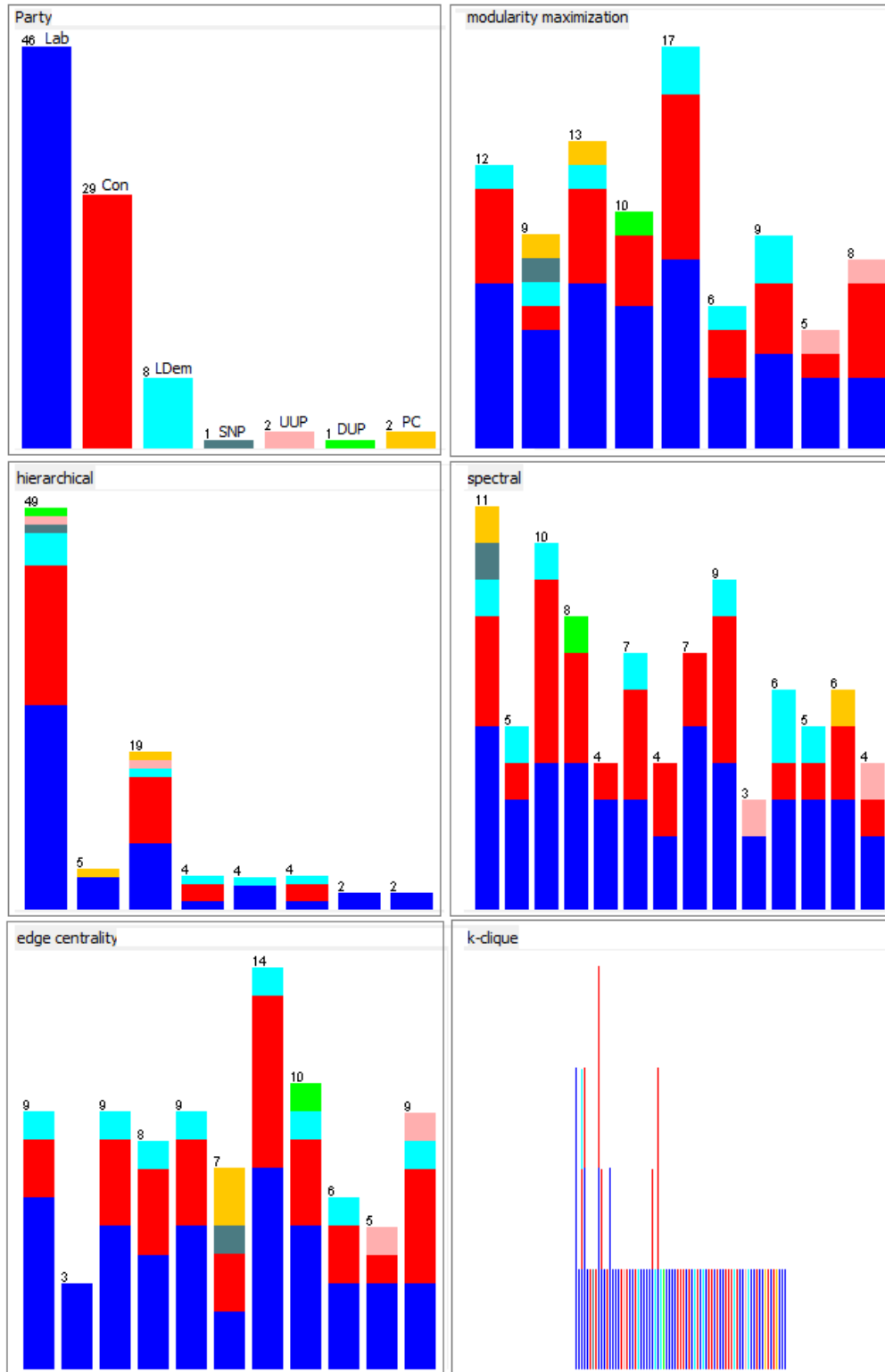
Figure 9.15: Communities in the relevant interruption network for the Iraq debate. The top left histogram presents the known communities (according to party affiliation) while the rest of histograms present the detected communities (clusters predicted using modularity maximization, hierarchical and spectral clustering, edge centrality and k-Clique percolation algorithms). The colour coding is defined in the top left histogram.
