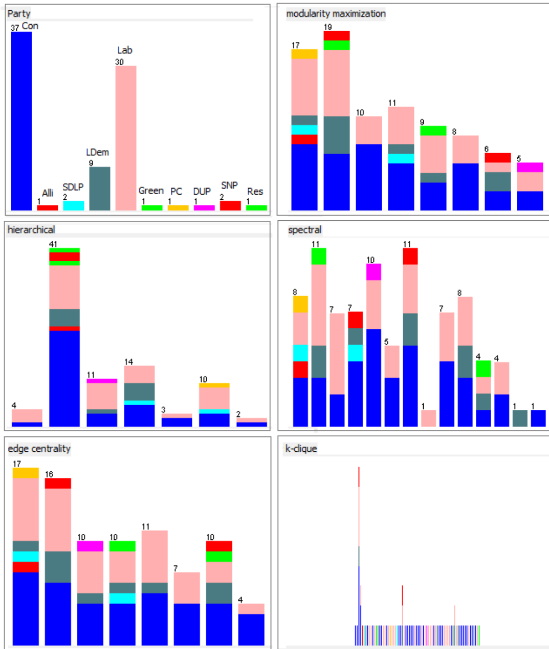
Figure 9.17: Communities in the relevant interruption network for the Syria debate. The top left histogram presents the known communities (according to party affiliation) while the rest of histograms present the detected communities (clusters predicted using modularity maximization, hierarchical and spectral clustering, edge centrality and k-Clique percolation algorithms). The colour coding is defined in the top left histogram.
