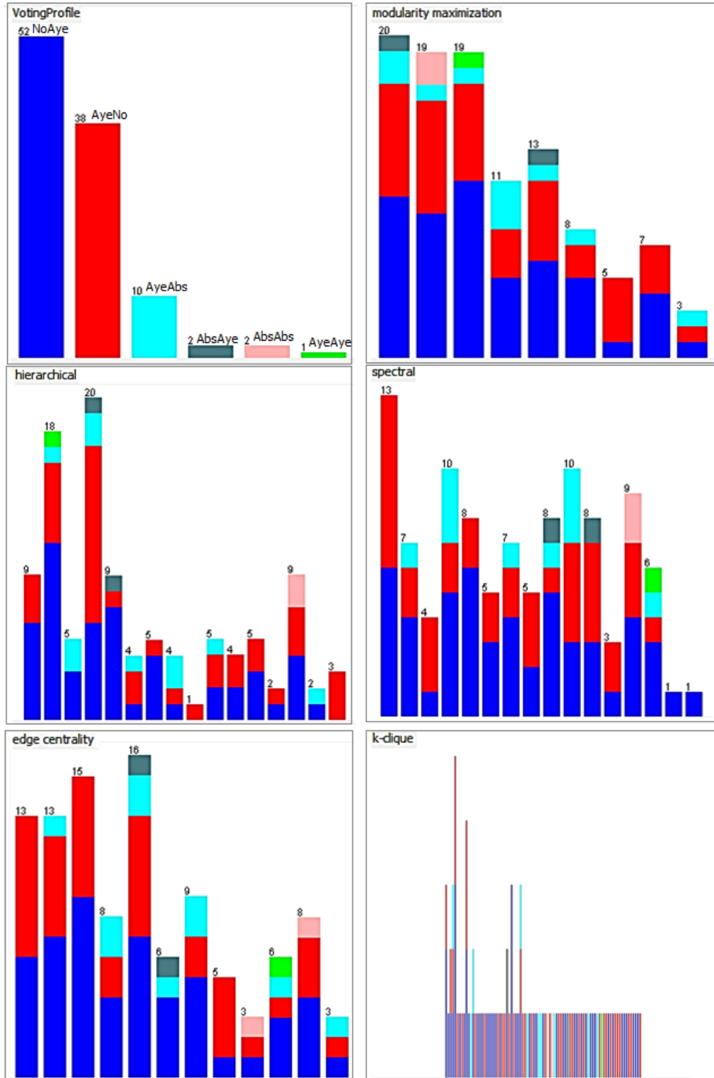
Figure 9.10: Communities in the interruption network for the Iraq debate. The top left histogram presents the known communities, according to voting profile, while the rest of histograms present the predicted communities using modularity maximization, hierarchical and spectral clustering, edge centrality and k-Clique percolation algorithms. The colour coding is defined in the top left histogram.
