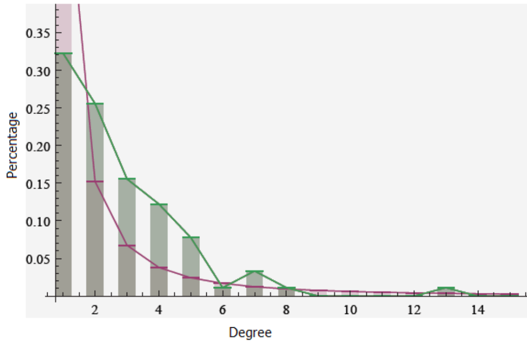
Figure 9.6: The power-law degree distributions for the Iraq debate interruption network (top) and the relevant interruption network (bottom). Each bar indicates the fraction of nodes (vertical axis) with respect to a given degree (horizontal axis). The degree distributions of both networks follow approximate power-law form indicated by the green curves, while the magenta curves indicate Zipfian distributions with the same range.
