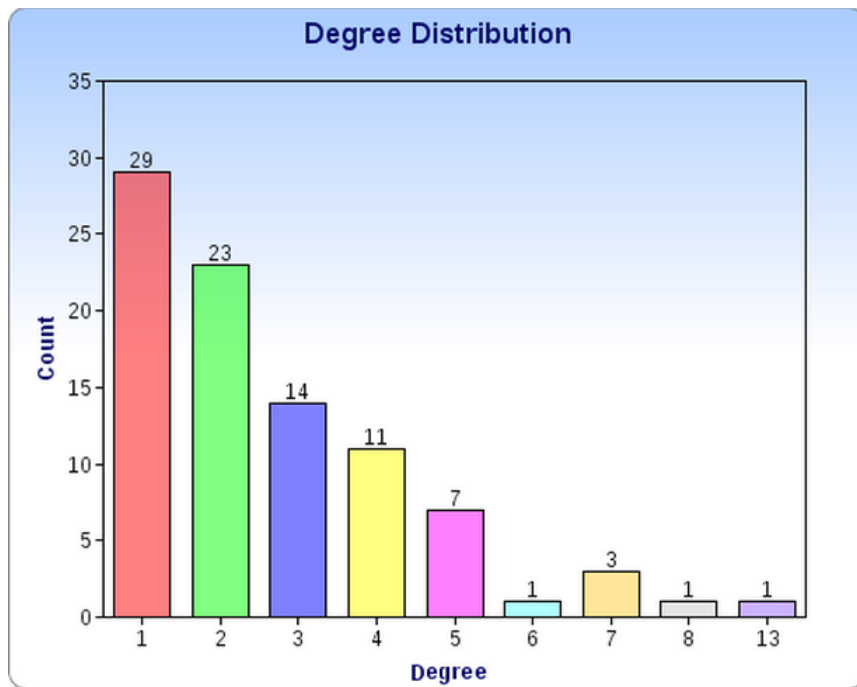
Figure 9.5: Degree distributions for the Iraq debate interruption network (top) and relevant interruption network (bottom). Each bar indicates the number of nodes (vertical axis) with respect to a given degree (horizontal axis).
