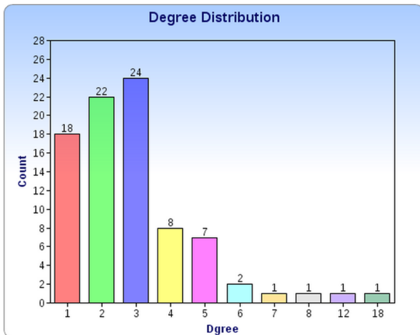
Figure 9.7: Degree distribution for the Syria debate interruption network (top) and relevant interruption network (bottom). Each bar indicates the number of nodes (vertical axis) with with respect to a given degree (horizontal axis).
