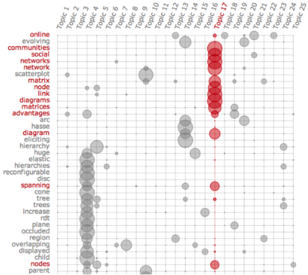
Figure 2.4: A tabular visualisation, produced using Termite, displaying the cooccurrences for a selected set of 30 terms.
