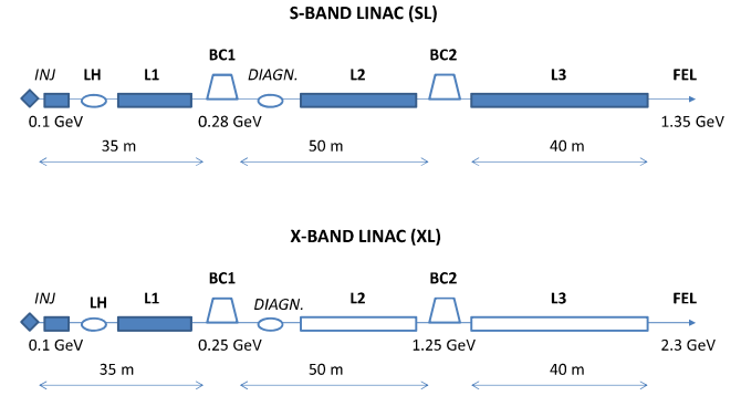
FIG. 5. Sketch of the linacs modeled for the brightness and the gain length study (not to scale). Filled rectangles are for S -band rf structures; empty rectangles are X -band. Labels in bold refer to elements modeled in this article.
