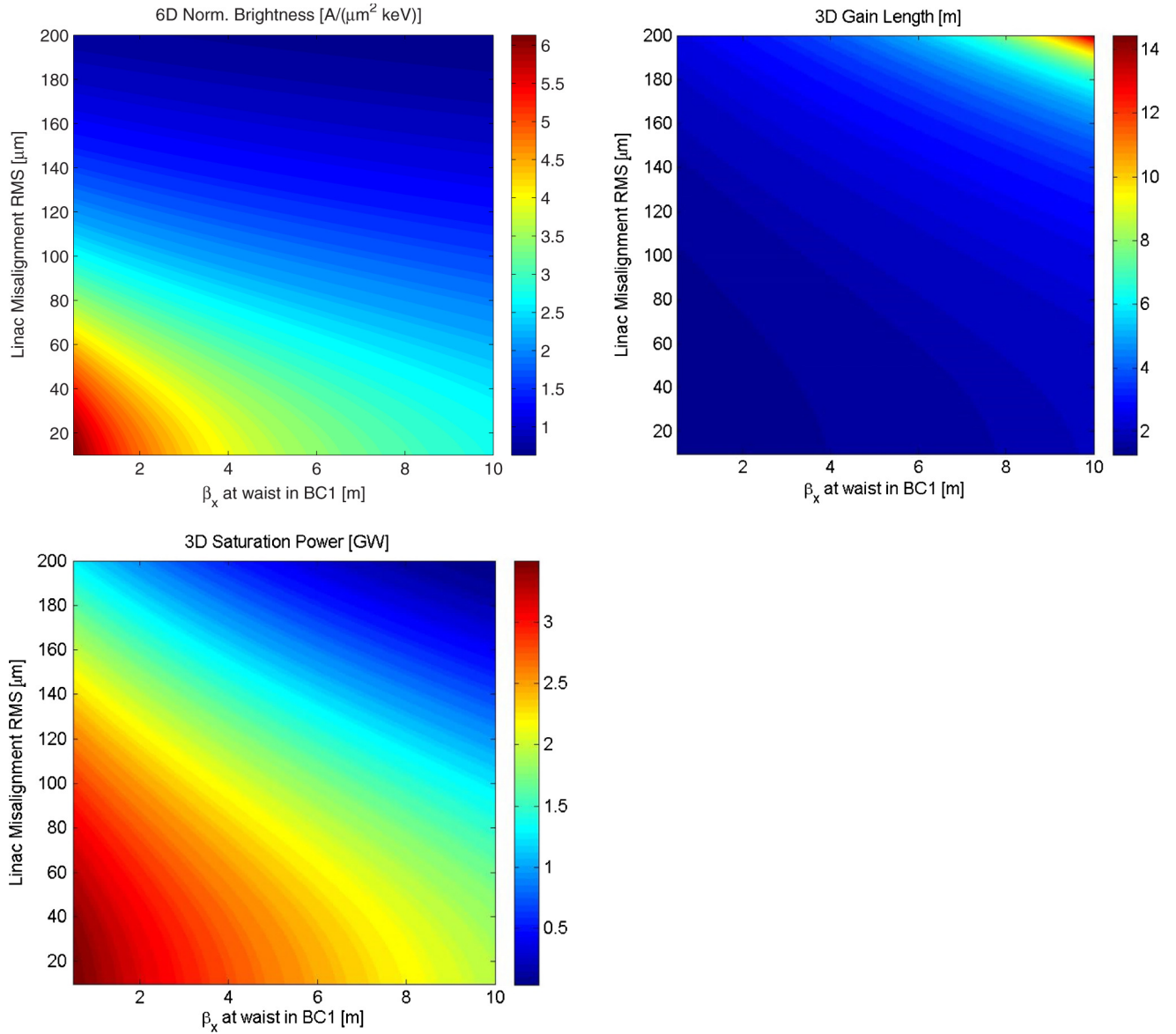
FIG. 9. Contour plot of B_{n,6D} (top left), L_{g,\text{coll}} (top right), and P_{\text{sat},\text{coll}} as a function of the rms linac-to-beam misalignment and of the minimum betatron function in BC1. A 500 pC bunch charge, compressed in one stage by a factor of 18 in the SL linac, was considered. The final peak current is 0.9 kA.
