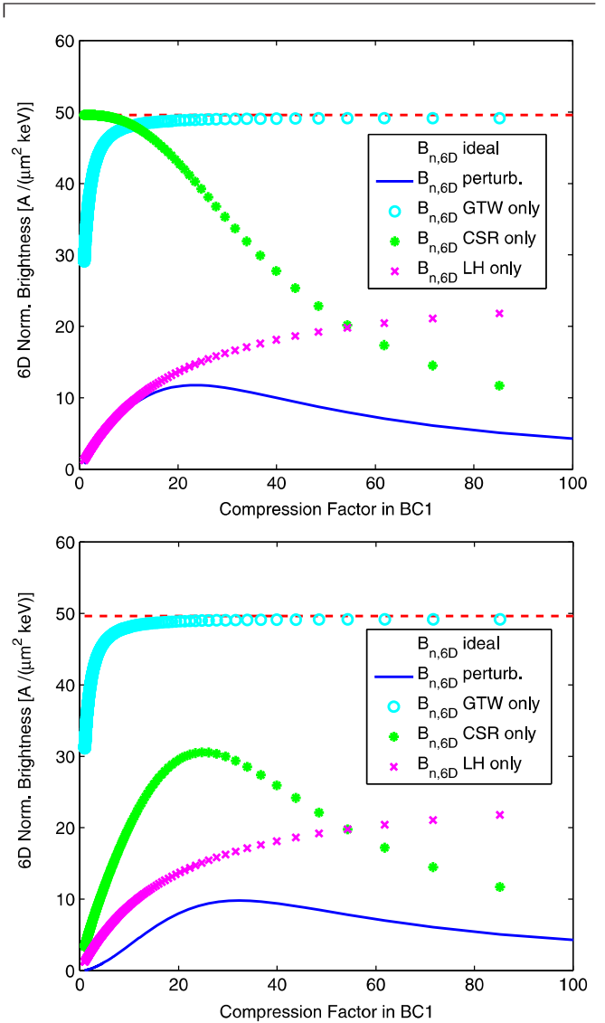
FIG. 7. Analytical estimate of B_{n,6D} at the end of XL (see Fig. 3) for the one-stage (left) and two-stage compression, as a function of the compression factor in BC1 . In the two-stage scheme, the total compression factor is fixed to 100.
