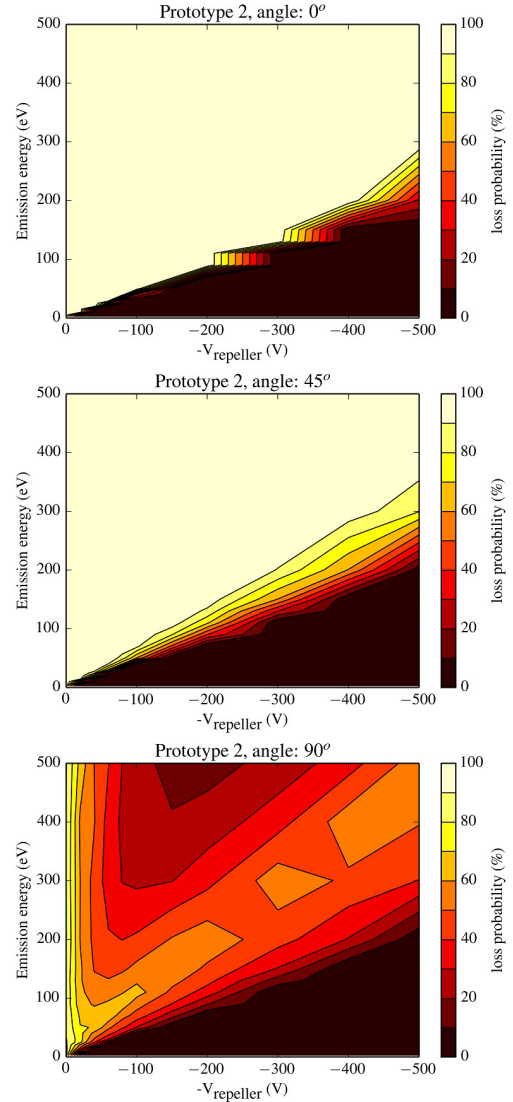
Figure 6: Loss probability of Prototype 2 at different emission energies, repeller ring voltages and maximum emission angles of 0°, 45° and 90°.
