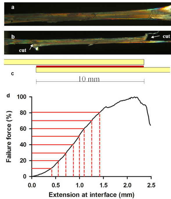
Fig. 1 – Images illustrating dissection for mechanical testing of the IFM. Two fascicles, bound by IFM, were dissected from the SDFT and CDET (a). The opposing end of each fascicle was cut transversely, leaving a 10 mm length of intact IFM connecting the fascicles (b and c). The fascicles were then pulled apart to failure, and the amount of extension at different percentages of failure force was calculated (d). Adapted with kind permission from eCM journal (Thorpe et al., 2013c).
