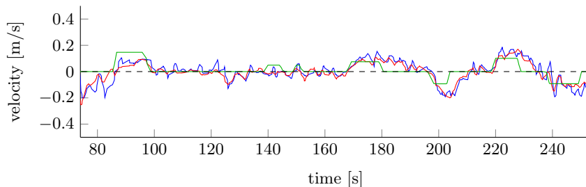
(b) Vertical velocity estimate (MSE: 0.0112, NMXM: 0.6068)
