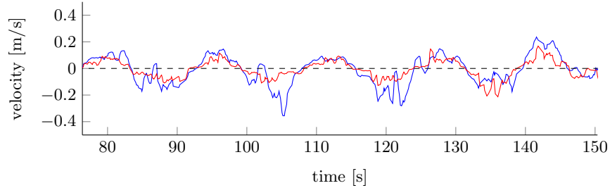
(b) Vertical velocity estimate (MSE: 0.0072 m, NMXM: 0.6066)
