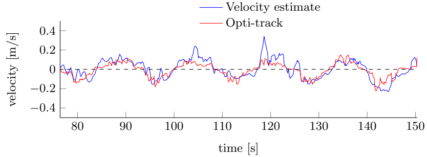
(a) Horizontal velocity estimate (MSE: 0.0064 m, NMXM: 0.5739)
