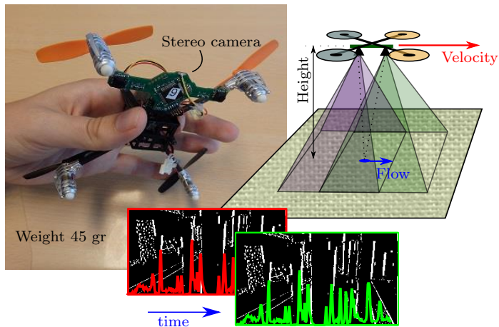
Figure 1: Pocket drone with velocity estimation using a downward looking stereo vision system. A novel efficient optical flow algorithm runs on-board an STM32F4 processor running at only 168 MHz and with only 192 kB of memory. The so-determining optical flow and height, with the stereo-camera, provide the velocity estimates necessary for the pocket drone’s low level control are obtained.
