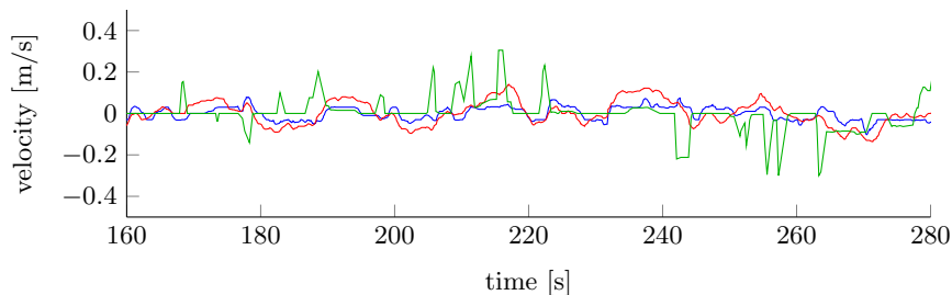
(b) Vertical velocity estimate (MSE: 0.0025 m, NMXM: 0.7494)
