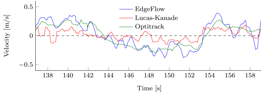
(b) Smoothed velocity estimates of EdgeFlow and Lucas-Kanade.
