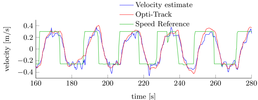
(a) Horizontal velocity estimate (MSE: 0.0041 m, NMXM: 0.9631)
