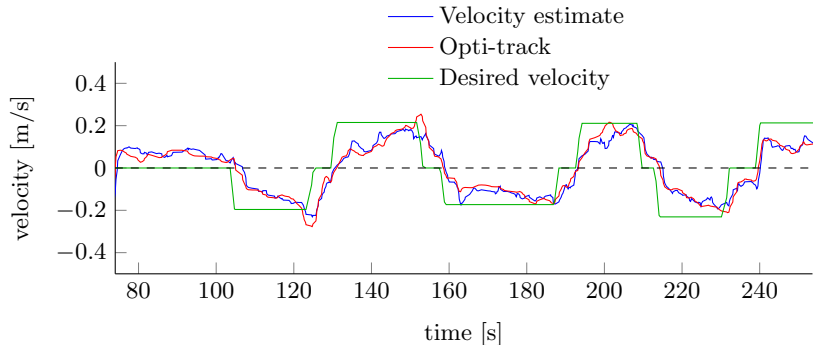
(a) Horizontal velocity estimate (MSE: 0.0224, NMXM: 0.6411)
