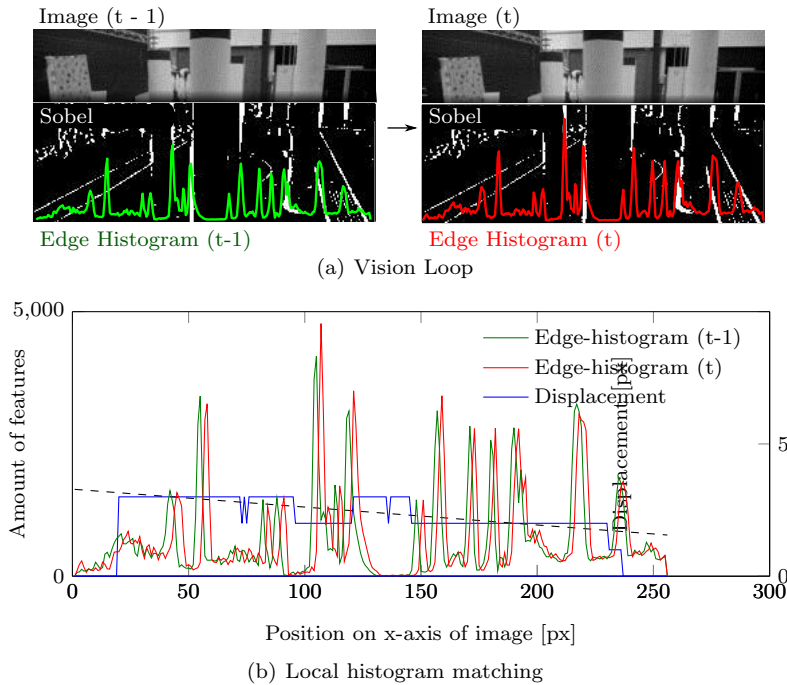
Figure 2: (a) The vision loop with for creating the edge feature histograms and (b) the matching of the two histograms (previous frame (green) and current frame (red)) with SAD. This results in a pixel displacement (blue) which can be fitted to a linear model (dashed black line) for a global estimation.
