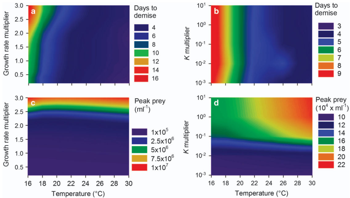
Figure 7 The effect of altering prey growth rate ( r_p ) and carrying capacity ( K ) on the time required for the predator to drive the prey to near extinction (that is, \sim 4 \times 10^5 cells \text{ml}^{-1} ) and the peak abundance of prey.
