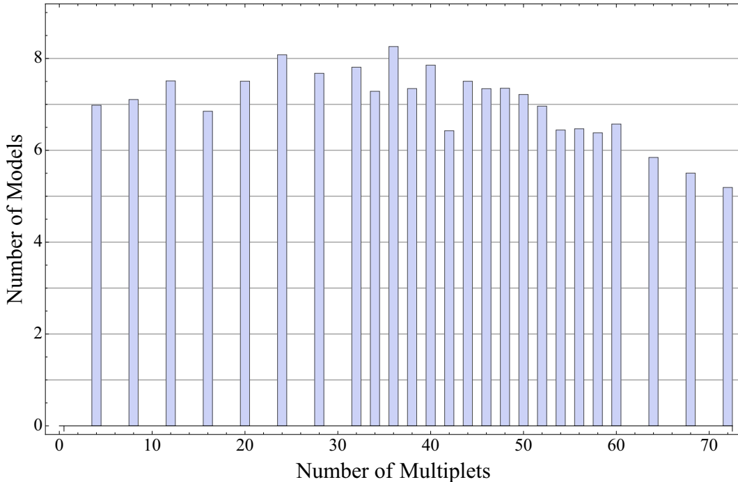
Figure 3: Logarithm of the number 3 generation models against the number of exotic multiplets ( n_e = n_{1e} + n_{\bar{1}e} + n_{5e} + n_{\bar{5}e} ) in a random sample of 10^{12} flipped SU(5) configurations.
