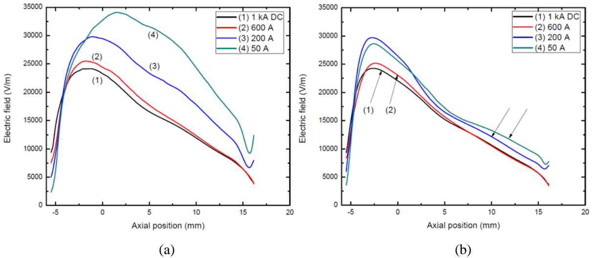
Figure 6. Variation of electric field with axial position at different instantaneous currents before current zero. P_0=21.4 atm and di/dt=13 A \mu s ^{-1} . (a) Standard k-epsilon model and (b) Chen-Kim model.
