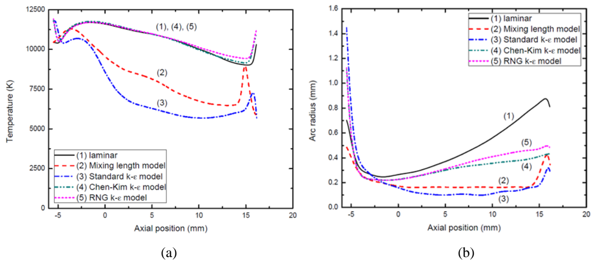
Figure 9. Variations of axis temperature and arc radius with axial position at current zero. (a) Axis temperature and (b) arc radius.
