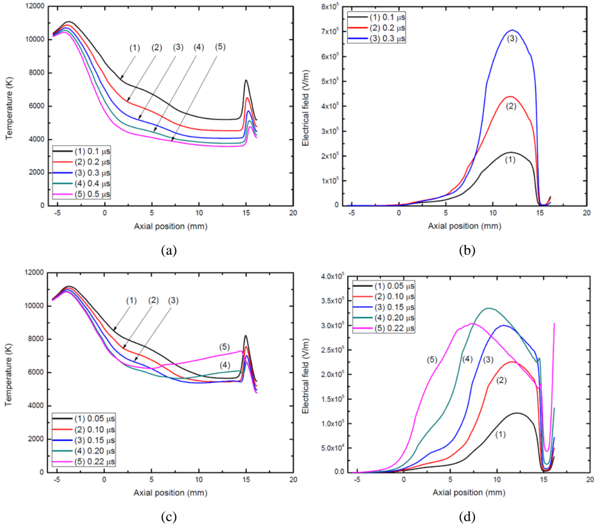
Figure 12. Axis temperature and electrical field distributions at various instants after current zero for the Prandtl mixing length model. (a) Axis temperature distribution and (b) electrical field distribution for dV/dt = 18 \text{ kV}\mu\text{s}^{-1} (thermal clearance); (c) Axis temperature distribution and (d) electrical field distribution for dV/dt = 19 \text{ kV}\mu\text{s}^{-1} (thermal reignition).
