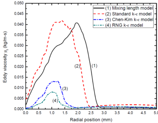
Figure 10. Radial profiles of the eddy viscosity at Z = 7.9 mm computed by different turbulence models at current zero. P_0=21.4 atm and di/dt=13 \text{A}\mu\text{s}^{-1} .
