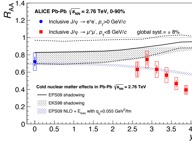
Fig. 10: Inclusive J/\psi R_{AA} as a function of the J/\psi rapidity measured in Pb–Pb collisions at \sqrt{s_{NN}} = 2.76 TeV [27], compared to theoretical calculations of CNM effects due to shadowing and/or coherent energy loss [65–67].
