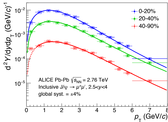
Fig. 5: Differential yields of inclusive J/\psi in Pb–Pb collisions at \sqrt{s_{\text{NN}}} = 2.76 TeV as a function of p_T for three centrality classes. Solid lines correspond to the results from the fit described in the text.
