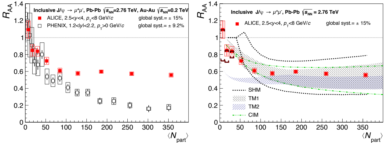
Fig. 7: Inclusive J/\psi R_{AA} as a function of the number of participant nucleons measured in Pb–Pb collisions at \sqrt{s_{NN}} = 2.76 TeV [27], compared to the PHENIX measurement in Au–Au collisions at \sqrt{s_{NN}} = 0.2 TeV [21] (left) and to theoretical models [13, 60, 62, 63], which all include a J/\psi regeneration component (right). The brackets shown in the three most peripheral centrality classes on the right figure quantify the possible range of variation of the hadronic J/\psi R_{AA} for two extreme hypotheses on the photo-production contamination in the inclusive measurement, see text for details.
