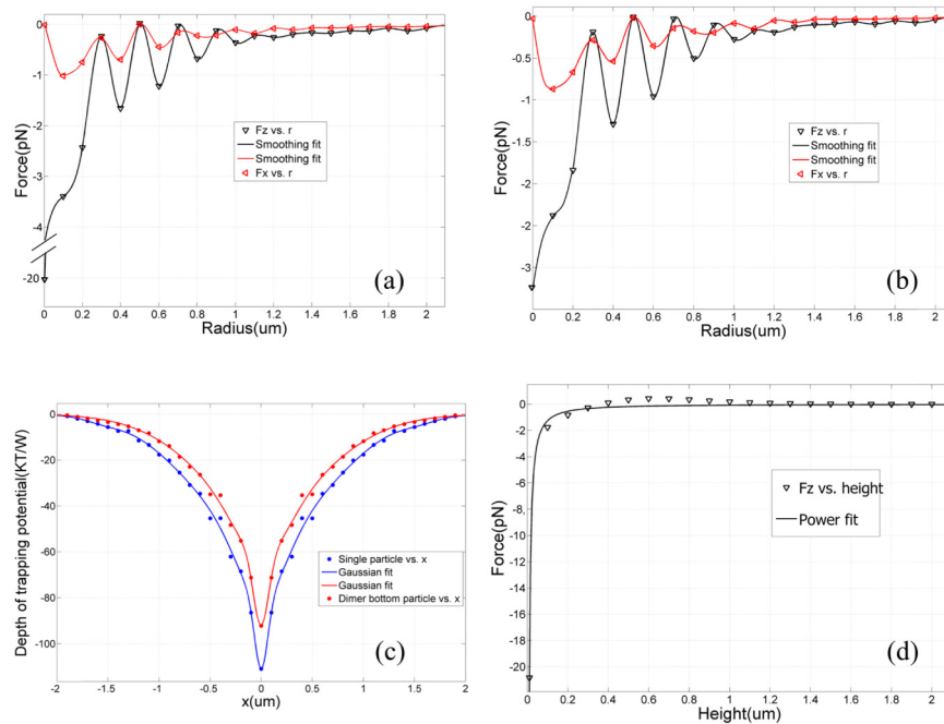
Fig. 4. The x- and z- direction total force distribution at the radial direction for (a) single particle above the Ag film and (b) vertically-oriented dimer above the Ag film, the bottom particle is studied. The parameters are same to Fig. 3. Radius is the particle offset length to the SP-VP center. The force was obtained every 100 nm. Both the particle-film and the particle-particle distances are 10 nm. The incident power is 1 W. (c) The calculated trapping potential well along x direction for single particle (blue curve) and the bottom particle of the dimer (red curve). (d) The z- direction force distribution with different height (particle bottom to surface) the single particle at the center and off the Ag film.
