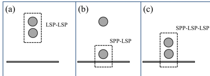
Fig. 7. Three plasmon hybridization modes: (a) dimer is far away from the film ( d_{pf} \gg d_{pp} ); (b) the dimer gap distance is large and the one sphere is close to the film ( d_{pp} \gg d_{pf} ); (c) dimer is close to the film ( d_{pp} \sim d_{pf} < R ).
