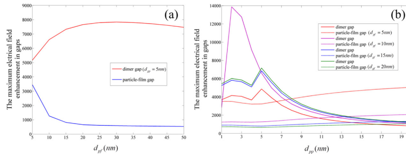
Fig. 6. The electrical field enhancement when changing d_{pf} (a) and d_{pp} (b) individually. The enhancement factor is obtained at the point next to the particle which will present the highest field value.
