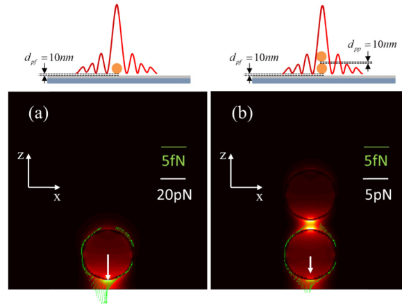
Fig. 3. The force analysis for: a single 50nm-diameter gold nanosphere: (a) placed on an Ag film; (b) a sphere is added to (a). The schematic diagrams show the locations of particles in the plasmonic field. d_{pp} and d_{pf} indicate the dimer gap distance and the particle-film gap dimer distance respectively. The green arrows show the forces at the points on the x-z section circle of the sphere. The white arrows indicate the total force as a result by the integral of the sphere surface. The background maps correspond to the electrical field.
