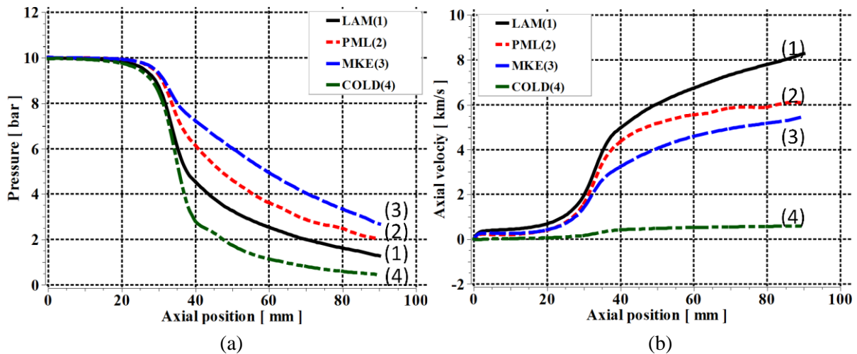
Figure 4. Variations of, (a) pressure and (b) axial velocity, along the nozzle axis for the 2 kA DC arc computed by three flow models. The pressure and axial velocity for the cold flow (Curve (4)) is also plotted to show the effects of the presence of the 2 kA DC arc.
