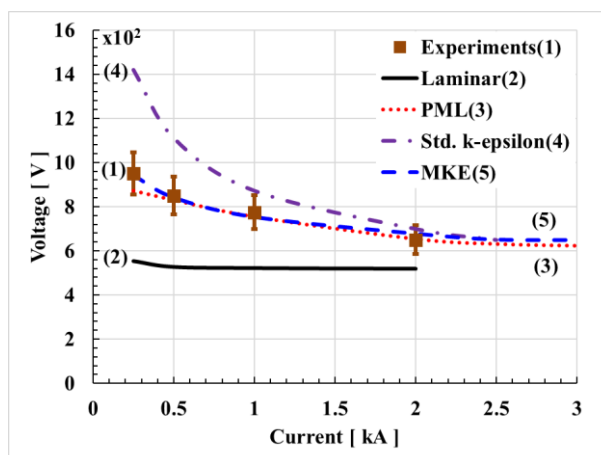
Figure 8. V-I characteristics for the DC air nozzle arcs at P_0=10 bar computed by the three flow models.
