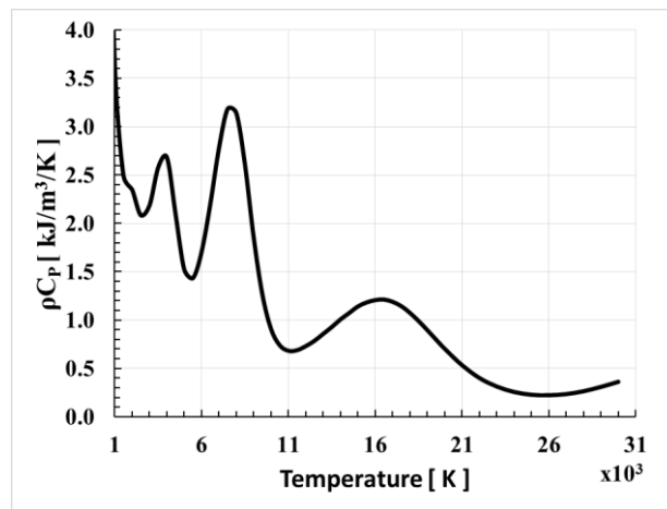
Figure 14. \rho C_p of air at the pressure of 10 bar.
