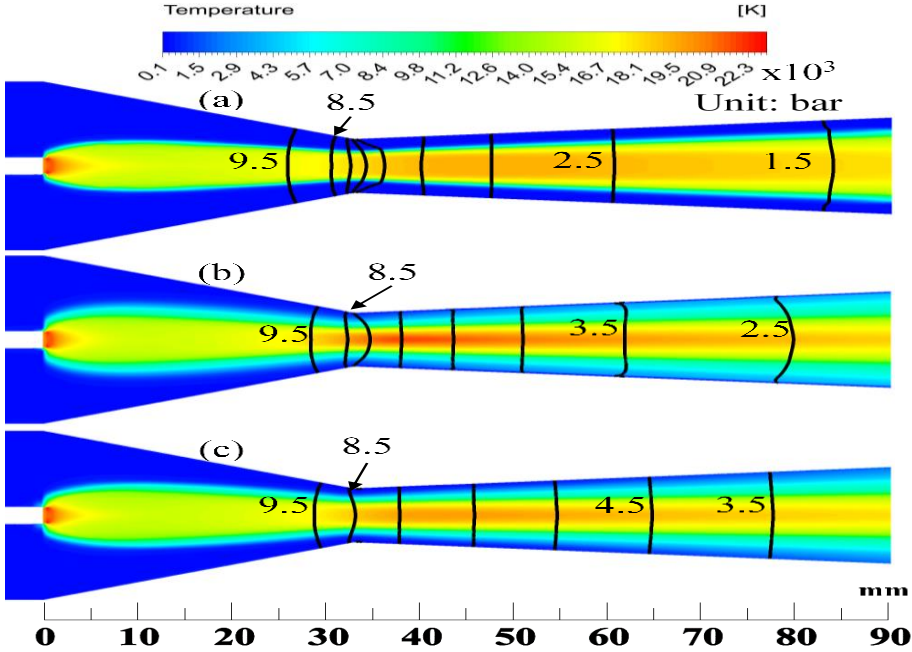
Figure 2. Temperature contour together with pressure isobars for a 2 kA DC arc at P_0 = 10 bar. The pressure difference between two adjacent isobars is 1bar. (a) Computed by laminar flow model; (b) Computed by PML; (c) Computed by MKE.
