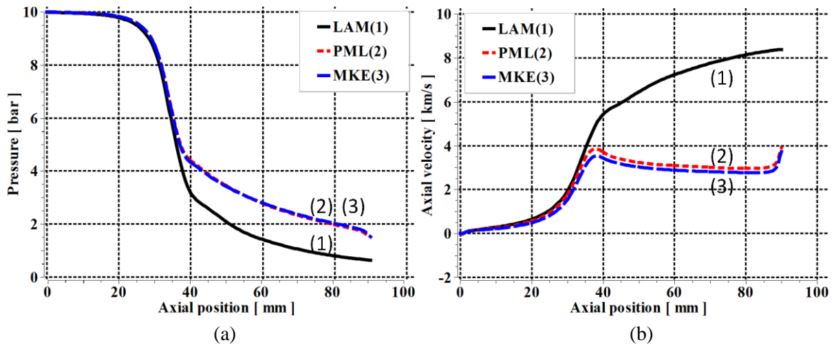
Figure 6. Variations of, (a) pressure and (b) axial velocity, along the nozzle axis for the 250 A DC arc computed by three flow models.
