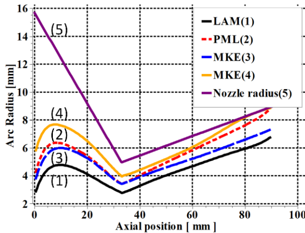
Figure 3. Variations of arc radius (radial position of 4,000 K isotherm) for 2 kA case computed by (1) laminar flow model; (2) PML and (3) MKE. Curve (4) is the arc radius for 3 kA computed by MKE, which shows that near the nozzle exit hot gas occupies the whole nozzle. Nozzle radius (5) is plotted to show the arc size in relation to the nozzle.
