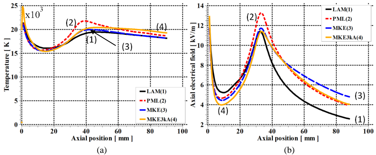
Figure 9. Variations of axis temperature of the 2 kA arc computed by laminar flow model, PML and MKE. The axis temperature of a 3 kA arc obtained by MKE is also plotted for comparison.
