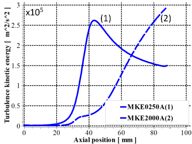
Figure 7. Axial distribution of axis turbulence kinetic energy per unit mass: (1) 250 A; (2) 2 kA calculated by MKE.
