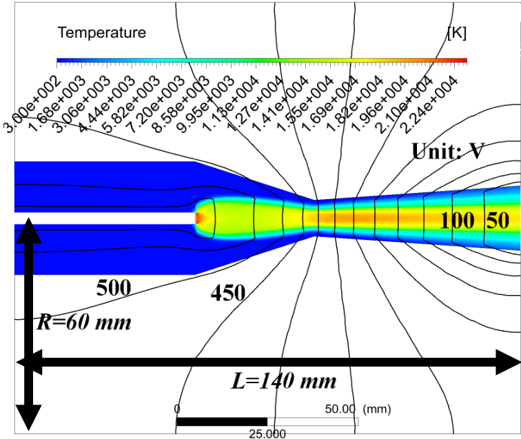
Figure 10. Temperature contour together with equipotential lines for the 2 kA DC arc at P_0 = 10 bar using MKE. Potential difference between two adjacent equipotential lines is 50 V. Computation domain has been extended to a radius of 60 mm from the axis to ensure that the potential distribution is no longer affected the size of the computation domain.
