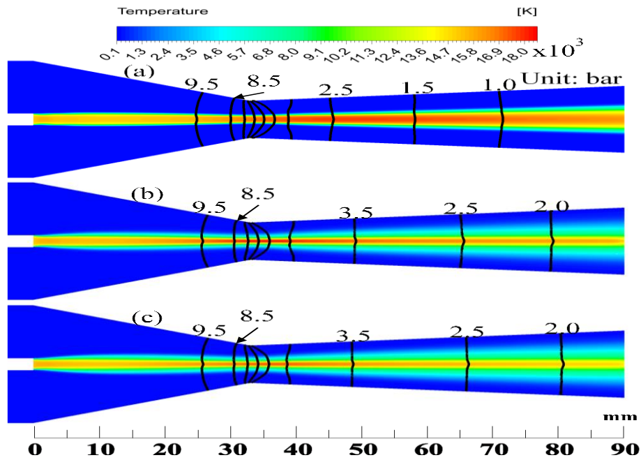
Figure 5. Temperature contour together with isobars for a 250 A DC arc at P_0 = 10 bar computed by (a) laminar; (b) PML; (c) MKE. The pressure difference between two adjacent unlabelled isobars after 8.5 bar is 1 bar.
