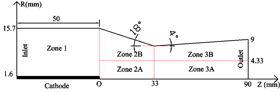
Figure 1. Nozzle geometry (not to scale) and grid system. The computation domain is divided into 5 zones: In Zone 1: a non-structured grids consisting of triangle cells with an average edge size of 0.5 mm is used. There are altogether 6872 grids. In Zone 2A uniform rectangular grids are used with a total number of grids of 66 (axial) x 130 (radial). There are 66x30 grids in Zone 2B. A total of 114 x 130 rectangular grids are placed in Zone 3A and 114 x 30 grids in Zone 3B. The radius of upstream electrode is 1.6mm. The radius of nozzle throat is 5mm. The origin of z-axis is at the upstream electrode tip.
