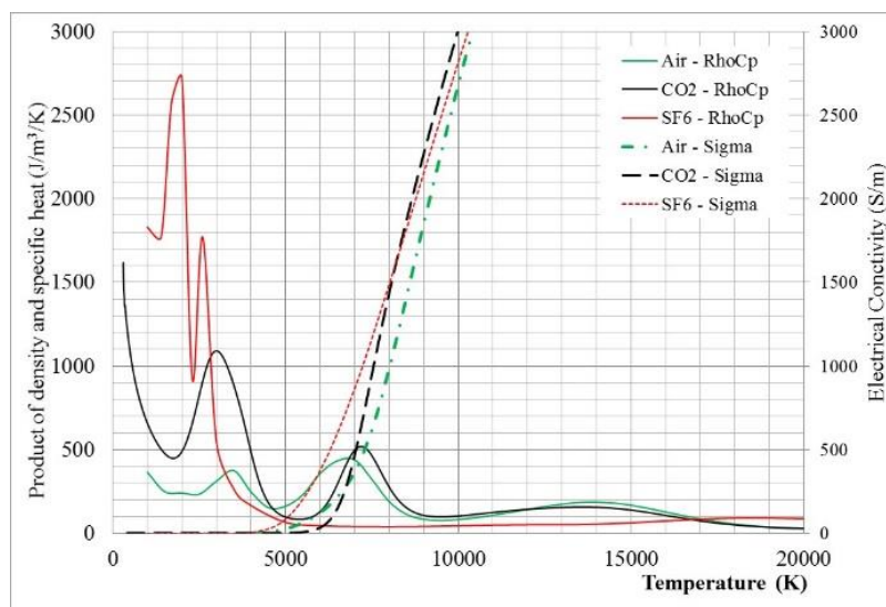
Figure 18. Electrical conductivity and \rho C_P of SF 6 [38], CO 2 [39] and air [13] at atmospheric pressure.
