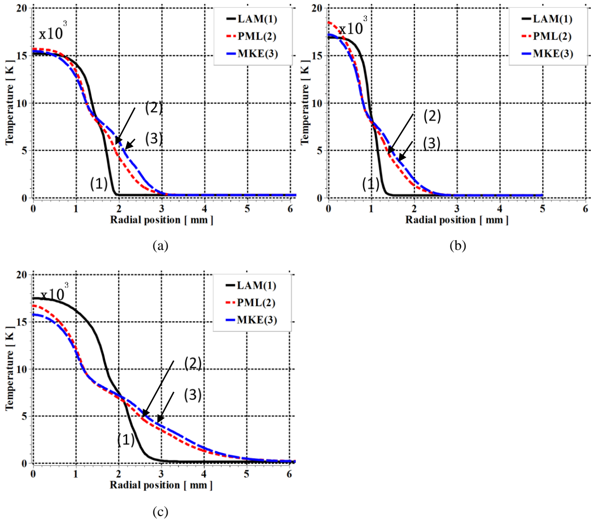
Figure 17. Radial temperature profiles computed by the three flow models for the 250 A DC arc at P_0 = 10 bar. (a) upstream midsection z= 15 mm; (b) nozzle throat, z= 33 mm; (c) downstream midsection z= 60 mm.
