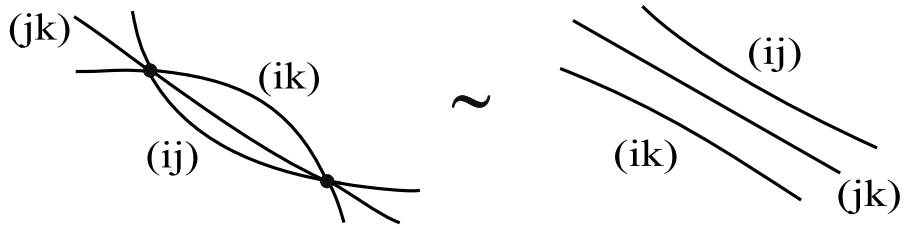
Fig. 5. Trihedral move on trace graphs.
