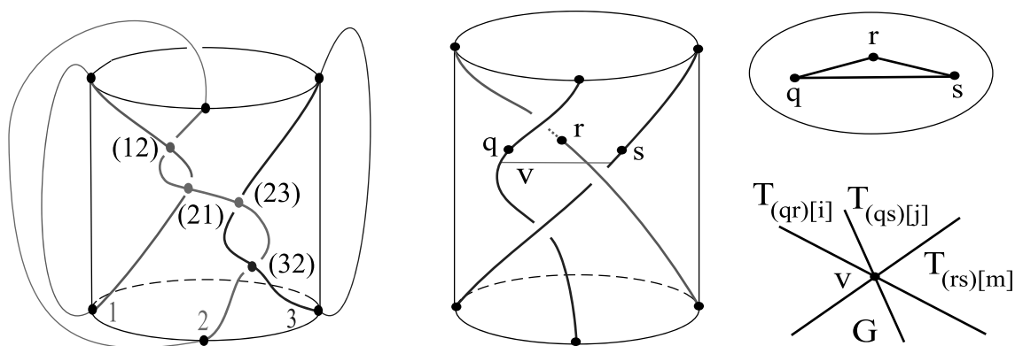
Fig. 10. Markings of crossings and trace circles.
