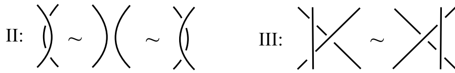
Fig. 2. Reidemeister moves on braids.
