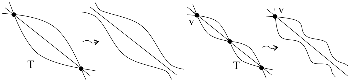
Fig. 14. Simulation of the appearance of a trihedron.
