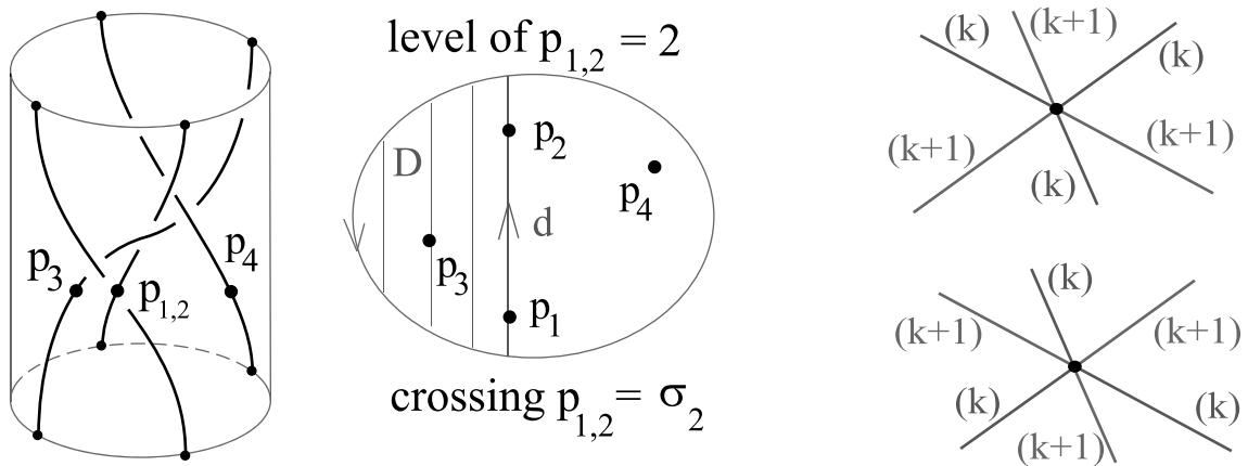
Fig. 12. Levels in trace graphs of closed braids.
