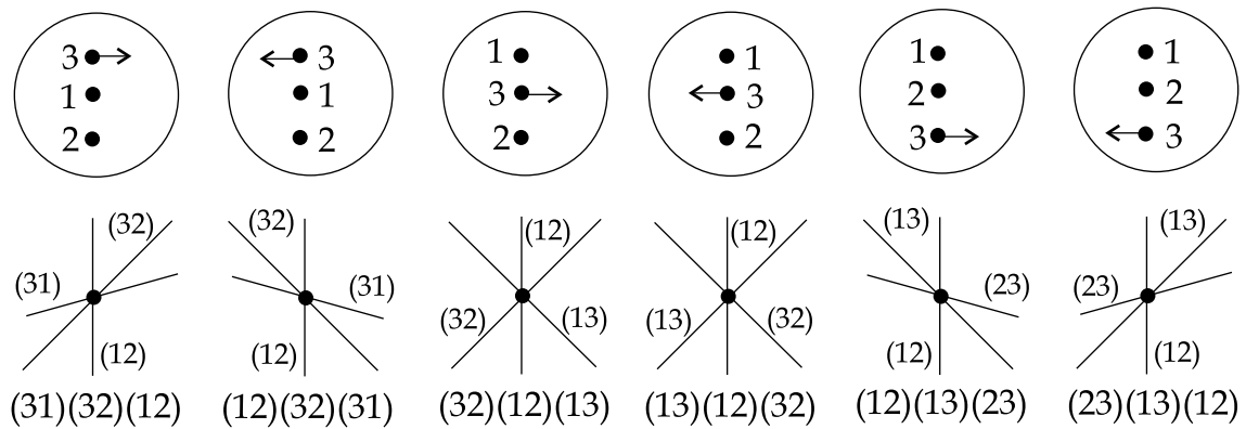
Fig. 16. Dynamic interpretation of triple vertices.
