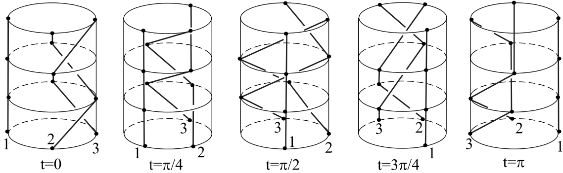
Fig. 3. Diagrams of rotated braids \text{rot}_t(\beta) for the braid \beta in Fig. 1.
