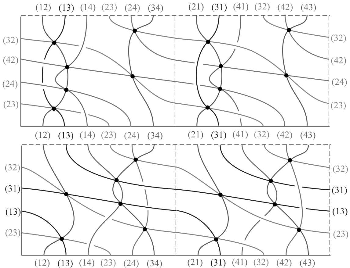
Fig. 11. Splittings of TG(\widehat{\sigma_2\sigma_3^2\sigma_2}) , TG(\widehat{\sigma_2\sigma_1^2\sigma_2}) into trace circles.
