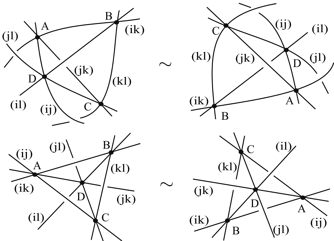
Fig. 6. Tetrahedral moves on trace graphs.
