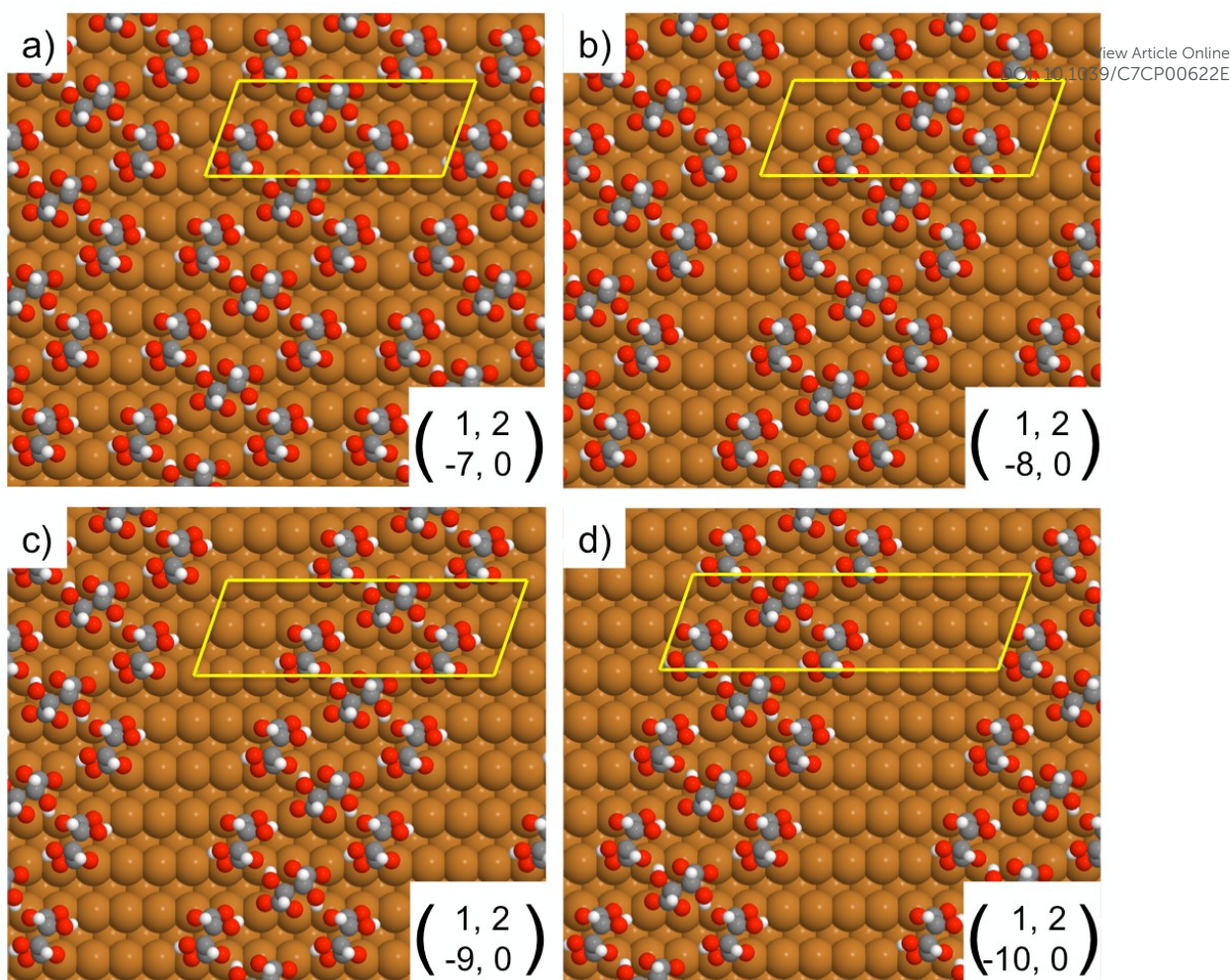
FIG. 4 Unit cells simulated by DFT for the R_{ec}O_aR_{ec} chain structure showing the width of the exposed Cu channel as the unit cell is progressively elongated from 7 to 10 Cu atoms along the \langle 1-10 \rangle direction. The local geometry of bitartrate in the trimer chains remains the same as in Figure 3b.
