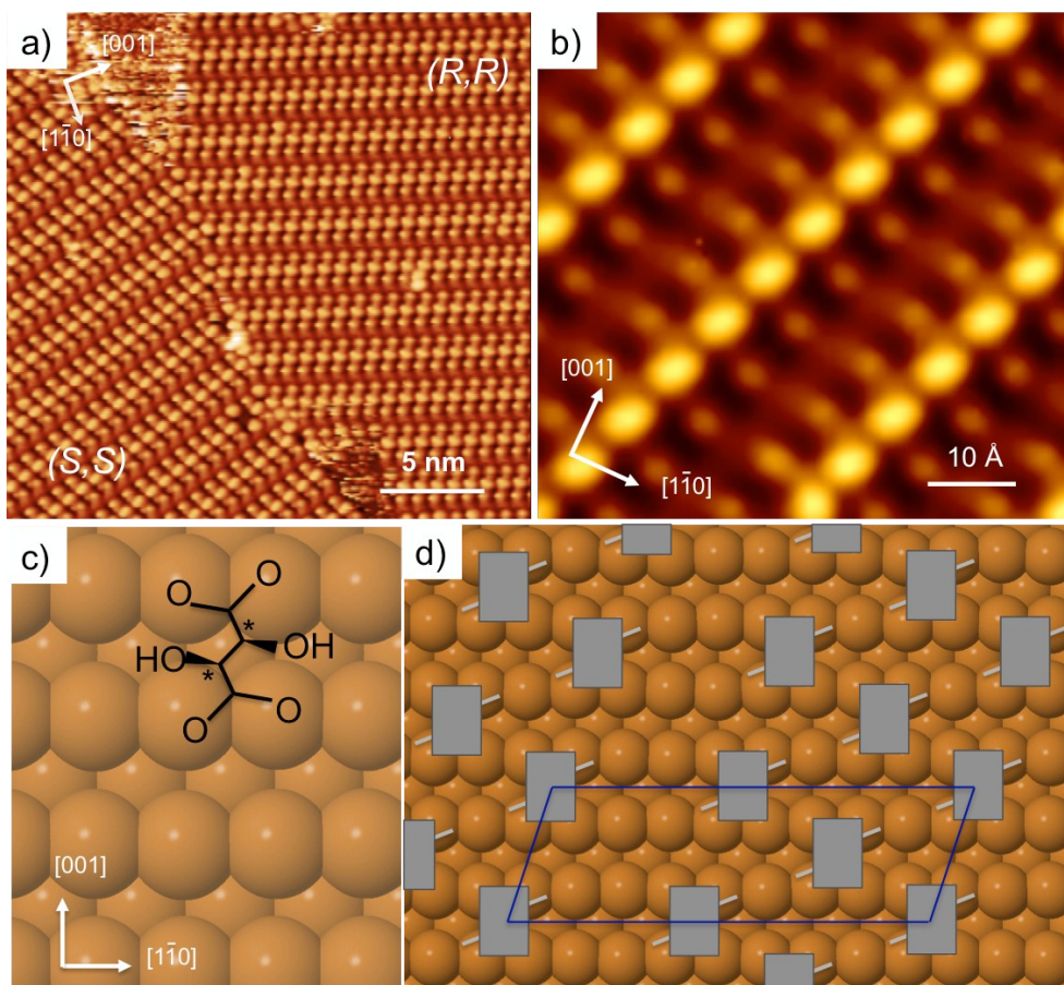
FIG. 1. STM images showing (a) domains of (9\ 0, -1\ 2) (S,S) and (1\ 2, -9\ 0) (R,R) bitartrate formed by dosing a racemic mixture of tartaric acid (300 K, -880 meV, 500 pA) and (b) a high resolution image of the (R,R) structure formed by dosing a single enantiomer (77 K, -510 meV, 280 pA). Schematics showing (c) the (R,R) bitartrate molecule (chiral centres marked *) and (d) the arrangement of (R,R) bitartrate in the (9\ 0, -1\ 2) unit cell proposed previously 22 .
