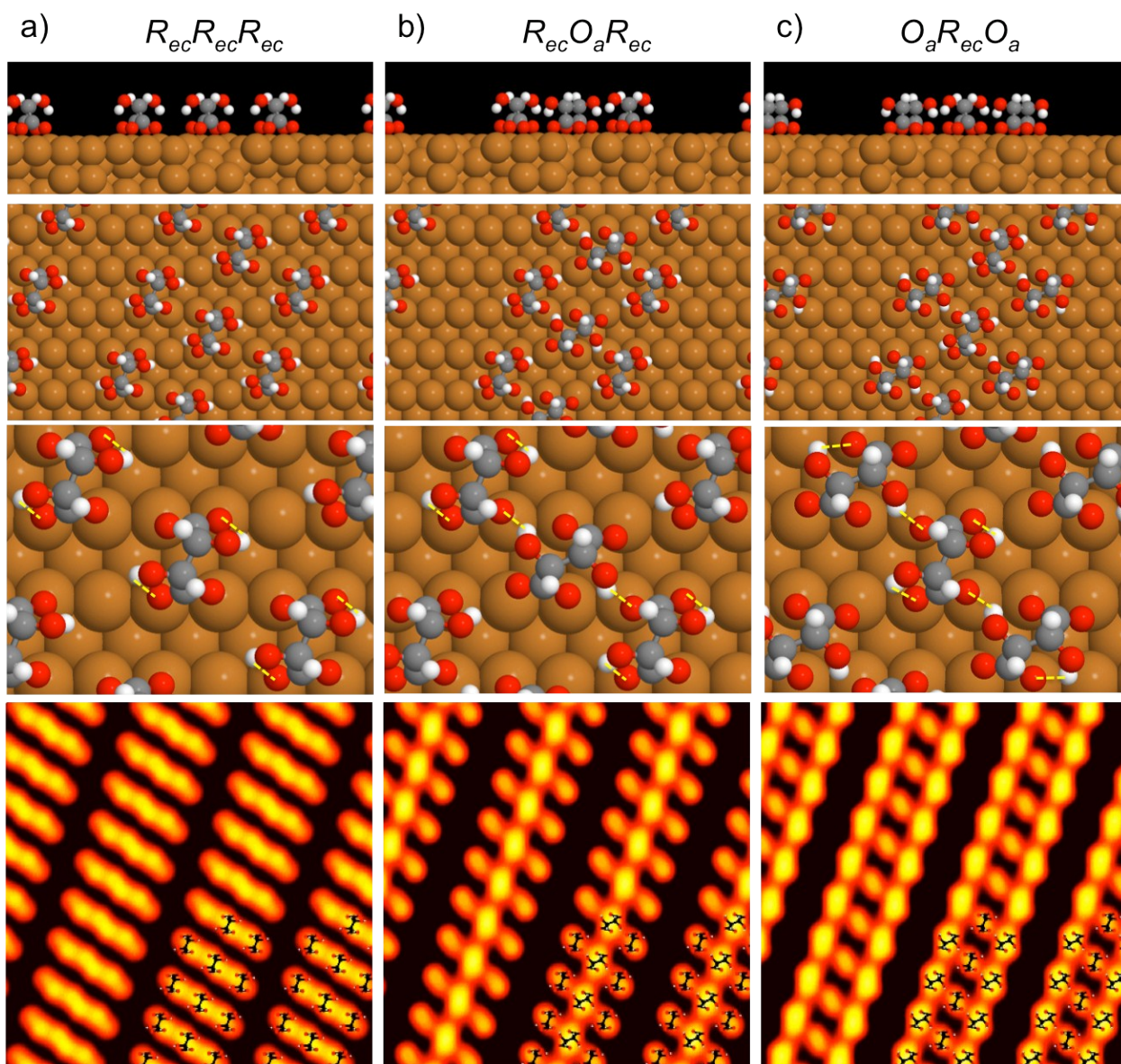
FIG. 3. Calculated structures for (R,R) bitartrate trimers in the (1 2, -9 0) unit cell, arranged with (a) the R_{ec}R_{ec}R_{ec} configuration, (b) an R_{ec}O_aR_{ec} arrangement and (c) an O_aR_{ec}O_a footprint. The top 2 rows show the end view of the chains and the overall arrangement of bitartrate trimers in the chains. The lower 2 rows show the inter- or intra-molecular hydrogen bonds within a trimer (marked as yellow lines) and, bottom row, simulated STM images for the different structures at the same bias voltage as Figure 1b, ( V=-500 meV).
