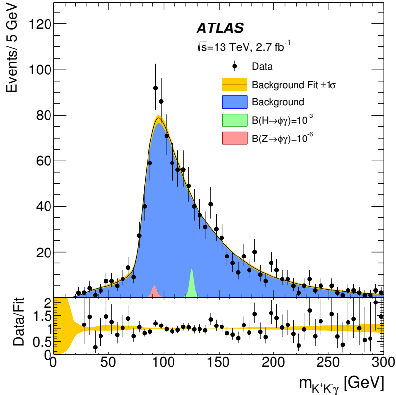
Figure 3: The m_{K^+K^- \gamma} distributions of the selected \phi\gamma candidates, along with the results of the maximum-likelihood fit with background-only model. The 1\sigma uncertainty band corresponds to the total uncertainty of the background model. The Higgs and Z boson contributions, expected for branching fraction values of 10^{-3} and 10^{-6} , respectively, are also shown.
