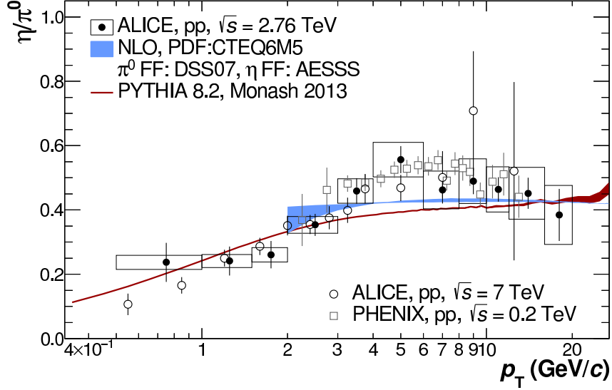
Fig. 10: Measured \eta/\pi^0 ratio in pp collisions at \sqrt{s} = 2.76 TeV compared to NLO pQCD calculations [6, 33] and PYTHIA 8.2 [14] generator-level simulations using the Monash 2013 tune. The horizontal error bars denote statistical, the boxes systematic uncertainties. The data at \sqrt{s} = 0.2 TeV [34] and \sqrt{s} = 7 TeV [4] are shown with statistical and systematic uncertainties added in quadrature.
