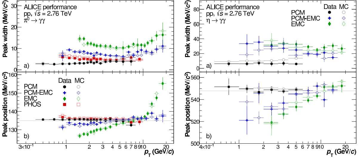
Fig. 5: Neutral pion (left panels) and \eta meson (right panels) mass position (bottom panels) and width (top panels) for the PCM, PCM-EMC and EMC methods. The performance of PHOS for \pi^0 is taken from Ref. [5]. Data are displayed as closed symbols, simulations as open symbols.
