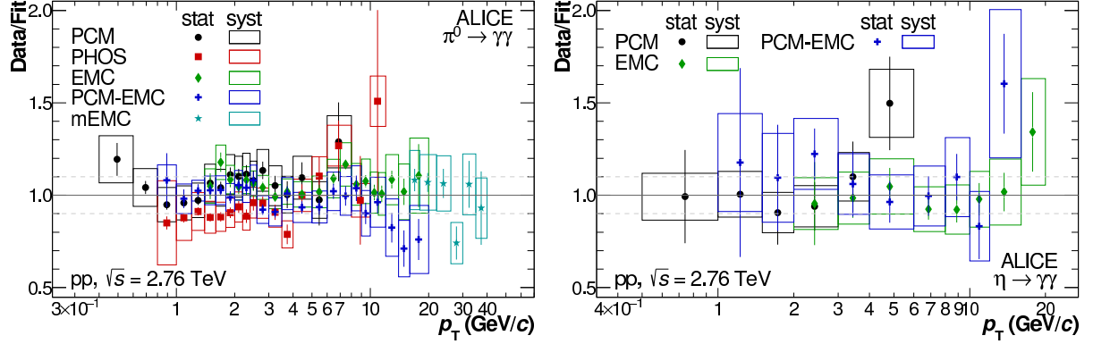
Fig. 8: Comparison of the individual measurements in their respective measured transverse momentum ranges relative to the two-component model fits [25, 26] of the final spectra. The final spectra are obtained by combining the individual measurements in the overlapping p_T regions with the highest granularity using the full correlation matrix as defined in the BLUE-algorithm [27–29].
