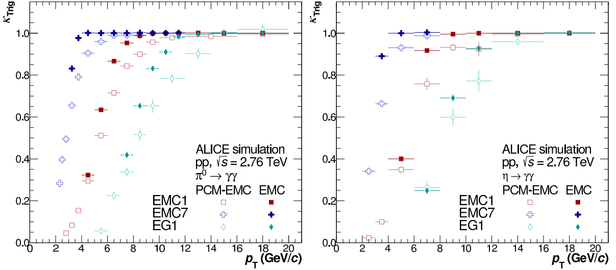
Fig. 2: Efficiency bias \kappa_{\text{Trig}} induced by different triggers (EMC1, EMC7 and EG1) for neutral pions (left panel) and \eta mesons (right panel) for PCM-EMC (open symbols) and EMC (closed symbols).
