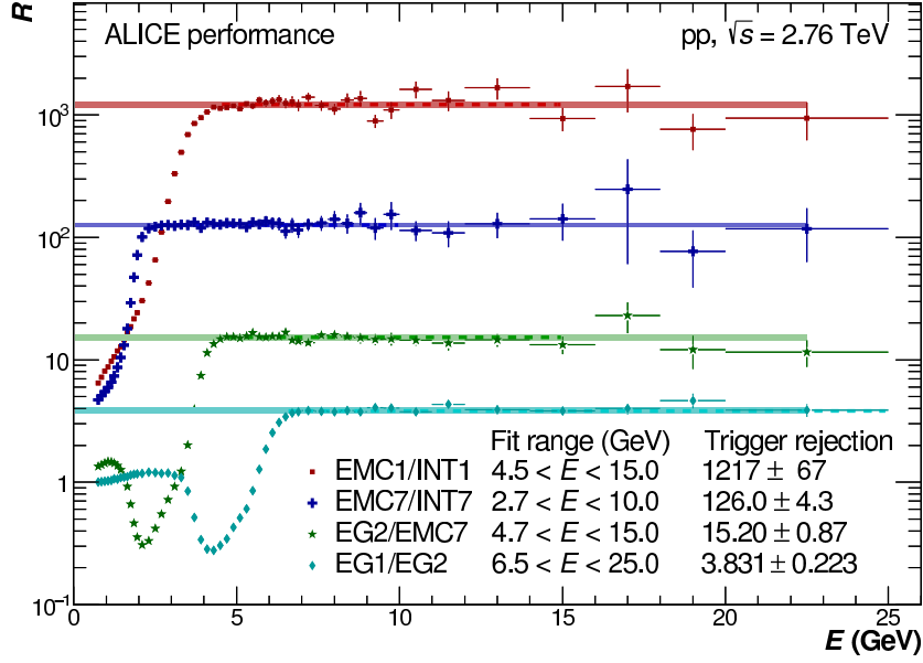
Fig. 1: Energy dependence of ratios between cluster spectra for EMC1/INT1, EMC7/INT7, EG2/EMC7 and EG1/EG2. The trigger names INT1 and INT7 denote the minimum bias triggers MB_{OR} and MB_{AND} respectively. The trigger names EMC1, EMC7, EG2 and EG1 denote the EMCal triggers at L0 in 2011 and 2013, and the EMCal triggers at L1 in 2013 with increasing threshold respectively. The individual trigger rejection factors and their respective fit ranges in the plateau region are indicated as well. The final rejection factors with respect to the minimum bias trigger are given in Tab. 1.
