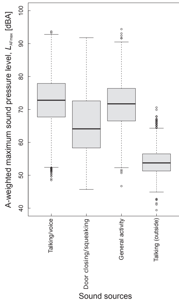
Fig. 4. Boxplots of A-weighted maximum sound pressure levels ( L_{AFmax} ) for dominant noise sources.
