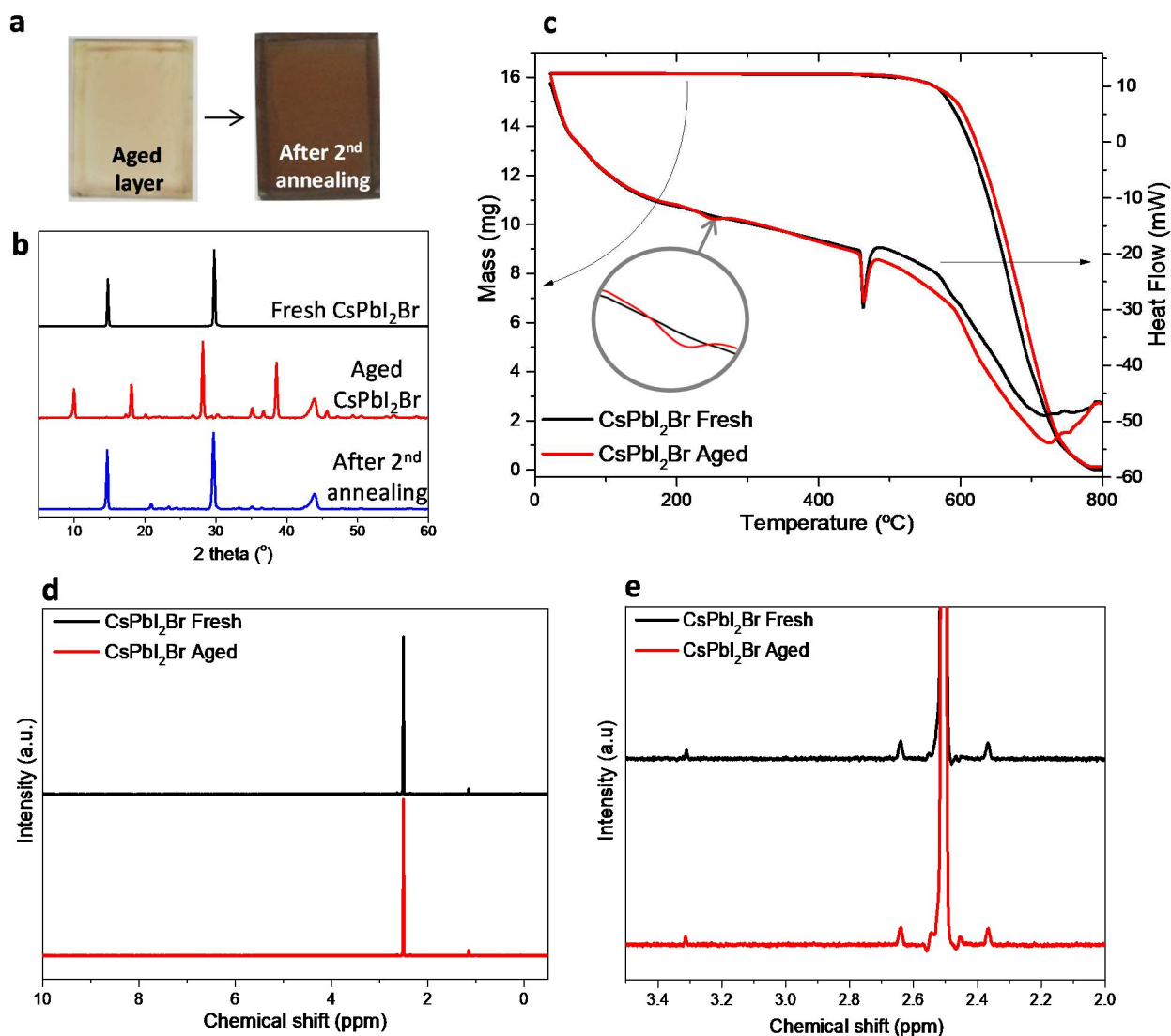
Figure 5. Physical investigation of the effects of water vapour on CsPbI 2 Br. (a) Photographs of an aged film before (yellow) and after (brown) recovery by heating at 350°C (2 nd anneal). (b) XRD pattern of films demonstrating that for aged films the original cubic crystal structure is re-established after annealing. (c) DSC-TGA of both fresh and aged powder samples. There is a melting peak at 463°C for both samples and a small exotherm at 255°C for the aged sample. (d,e) 1 H NMR of fresh and degraded samples in d 6 -DMSO. These show only peaks from the solvent. We conclude that the transformation from the brown to the yellow phase does not cause water to be included in the structure as a major component, and is reversible by heating.
