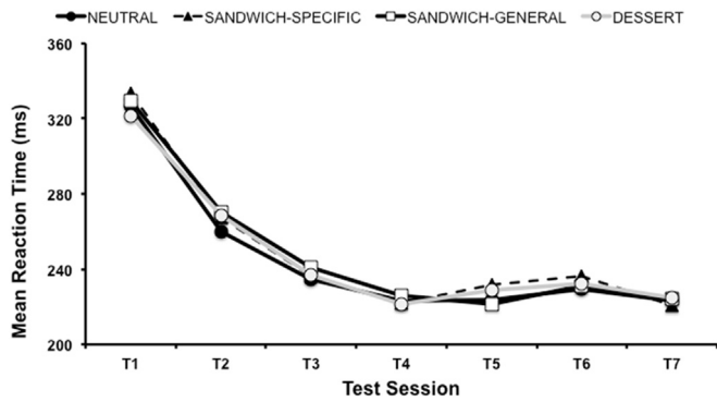
Fig. 5. Average reaction times for correct trials with streams containing the different distractor types at successive tests.
