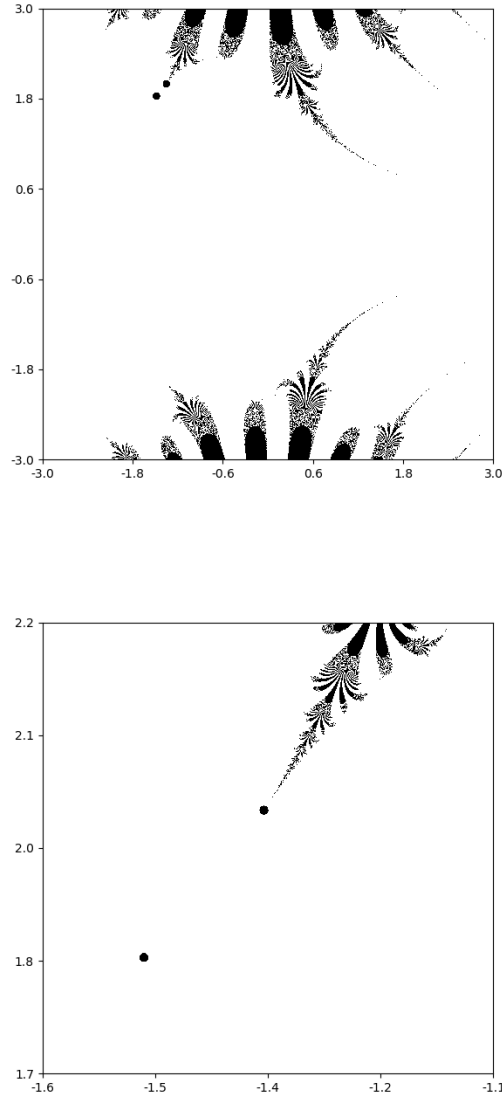
FIGURE 1. Two views of the Julia set (black) of f_{\alpha, \beta} . The asymptotic values \pm\alpha + \beta are denoted by black circles; in particular \alpha + \beta is the top right circle, and is a parabolic fixed point.
