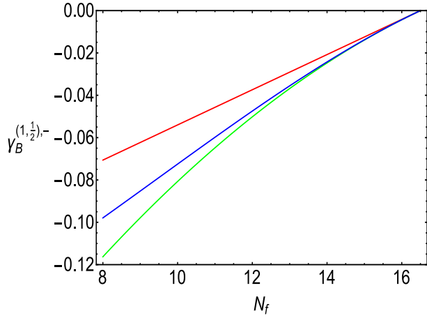
FIG. 4: Plot of \gamma_B^{(1,1/2),-} , as calculated in the scheme-independent series expansion to O(\Delta_f^p) with 1 \leq p \leq 3 , as a function of N_f . The curves refer to the calculation to (a) O(\Delta_f) (red) O(\Delta_f^2) (green), and O(\Delta_f^3) (blue), with colors online.
