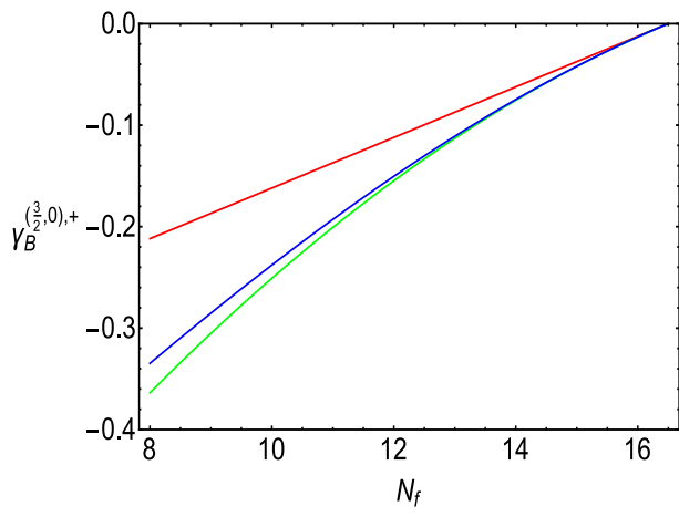
FIG. 3: Plot of \gamma_B^{(3/2,0),+} , as calculated in the scheme-independent series expansion to O(\Delta_f^p) with 1 \leq p \leq 3 , as a function of N_f . The curves refer to the calculation to (a) O(\Delta_f) (red) O(\Delta_f^2) (green), and O(\Delta_f^3) (blue), with colors online.
