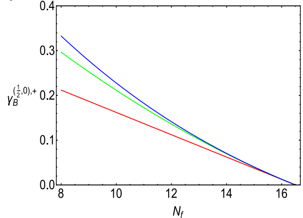
FIG. 1: Plot of \gamma_B^{(\frac{1}{2},0),+} , as calculated in the scheme-independent series expansion to O(\Delta_f^p) with 1 \leq p \leq 3 , as a function of N_f . The curves refer to the calculation to (a) O(\Delta_f) (red) O(\Delta_f^2) (green), and O(\Delta_f^3) (blue), with colors online.
