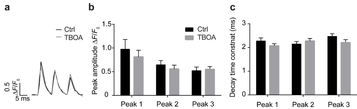
Fig. S4. Testing the effect of glutamate uptake blocker trifluoromethyl-benzoyl-aminophenyl-methoxy-L-aspartic acid (TBOA) on synaptic iGlu_u transients. (a) Average traces ( iGlu_u ) from single Schaffer collateral bouton stimulated at 100 Hz, before and after wash-in of TBOA (40 \mu M). (b) Peak amplitude was not affected by TBOA ( n = 10 boutons) (c) Decay kinetics was not affected by TBOA ( n = 10 experiments).
