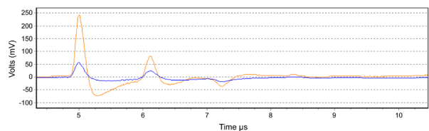
Figure 10: Partial Discharge pulse and the PD reflection (yellow phase) and the crosstalk on the blue phase.
