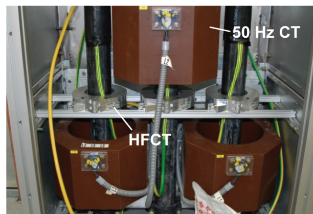
Figure 1: Permanent HFCT sensors installed above traditional CT for 50 Hz and power quality measurements.
