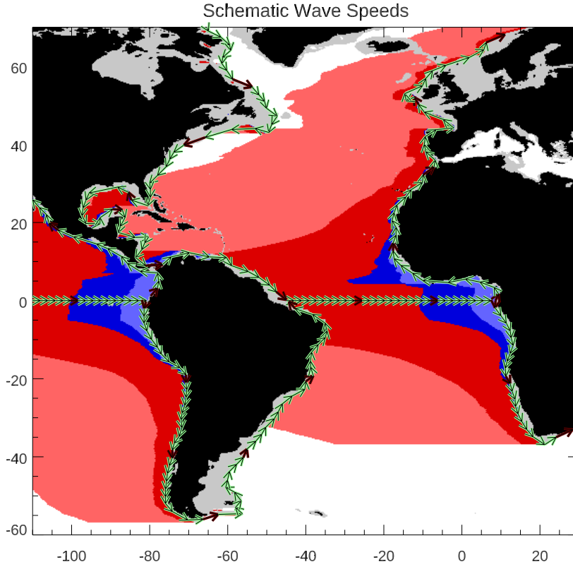
Fig. 1 Illustration of subinertial wave speeds in a flat-bottomed ocean, showing the fastest (long wavelength) mode-1 waves, and assuming a spatially uniform typical Kelvin wave speed of 2.5 \text{ ms}^{-1} . Arrows show the distance covered per day by Kelvin waves, with every tenth day highlighted. Colours show the westward distance covered by Rossby waves from the eastern boundary in ten days (pale blue), one month (dark blue), one year (red) and ten years (light red). For each, the boundary of the ocean is taken as the 500 m isobath (shallower regions are grey). In a more realistic ocean with variable stratification and bathymetry, the Rossby wave speeds would be reduced, and the boundary wave speeds increased, at high latitudes.
