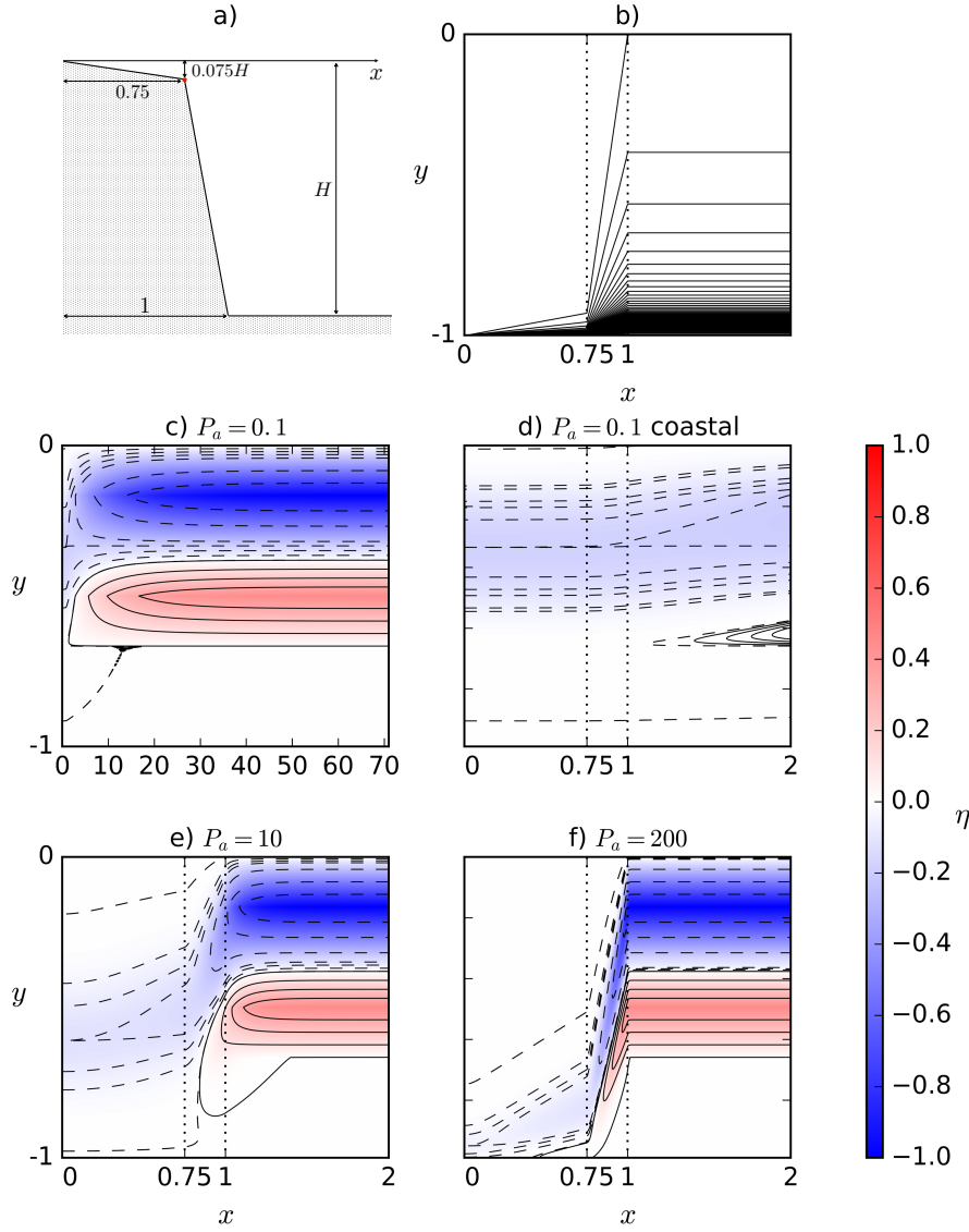
Fig. 4 Western ocean sea level in a barotropic model with topography, adapted from figures 3,4 and 5 of [50]. a) Geometry of the western boundary topography, with x measured in units such that the foot of the continental slope is at x = 1 . b) Corresponding contours of the string function gh/f , with equal spacing (values increase to the south). The y axis represents a range of 6000 km from the equator at y = -1 to the northern boundary at y = 0 , on this constant-beta geometry. c) High friction solution, similar to the vertical sidewall case, resolving the full width of the Stommel boundary layer ( P_a is the width of the topography measured in units of Stommel boundary layer width). d) Blow-up of c), focusing on the region with topography. e) and f) similar to d), but with lower friction (narrower Stommel boundary layers).
