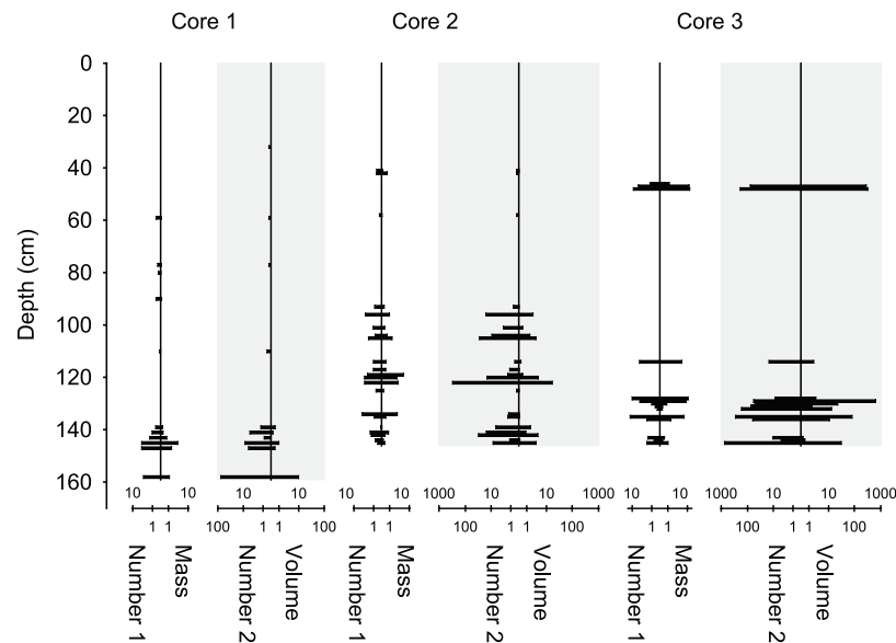
Figure 4. Charcoal records in three neighbouring peat cores collected at different distances from the margin of a small peat basin. Horizontal bars show the number (count), mass (g) and volume of charcoal particles ( \text{cm}^3 ) as estimated by two different methods, where number 1 and mass were estimated by a mass quantification method based on manual hand picking, and number 2 and volume (light grey shaded) were estimated by automated image analysis; see ‘Material and methods’ for further information. Core 1 was collected in the centre of the peat basin and core 3 was collected closest to the basin border. The distance between cores 1 and 2 was ca. 2 m, and the distance between cores 2 and 3 was ca. 3 m. Note logarithmic scale.
