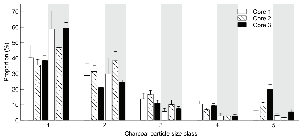
Figure 3. Proportion of charcoal particles in different size classes from three neighbouring peat cores as estimated by two different methods. Light-grey-shaded proportions were estimated by automated image analysis and the unshaded proportions were estimated by manual hand picking; see 'Material and methods' for further information.
