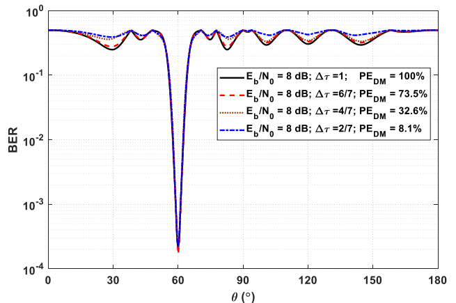
Fig. 4. Simulated BERs of the time-modulated OFDM arrays for various \Delta\tau when E_b/N_0 along \theta_0 of 60^\circ equals 8 dB. ‘ \Delta\tau=1 ’ refers to the conventional beam-steering array. It is assumed that each sub-carrier is QPSK modulated and N=7 , K=64 .
