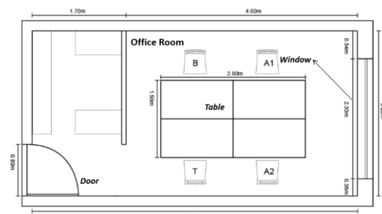
Figure 1: Room plan and dimension, window, and sitting positions.
