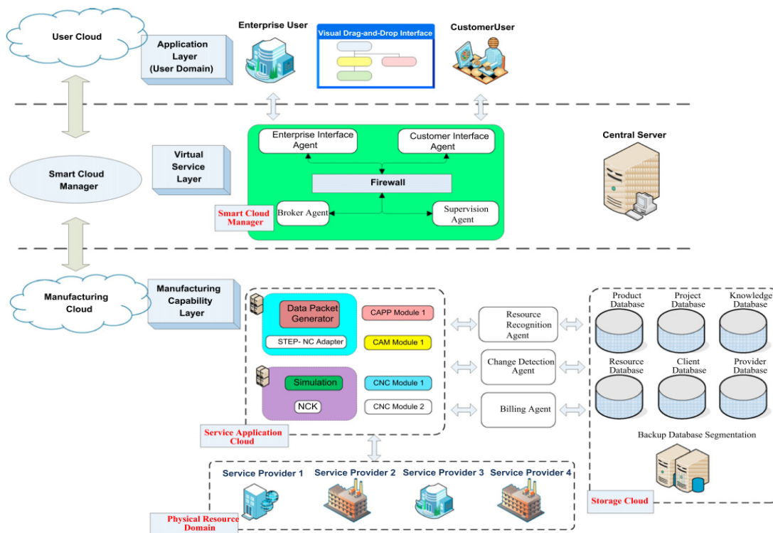
Figure 2: ICMS architecture [25]
