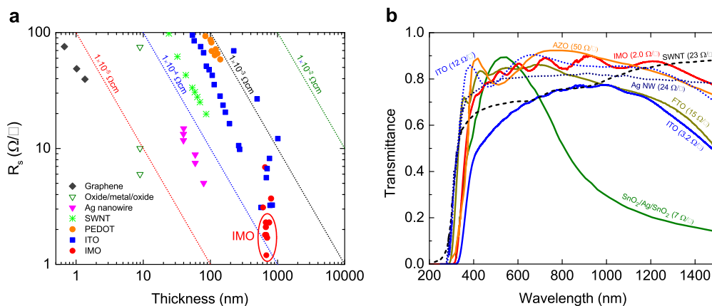
Fig. 1 Sheet resistances and optical transmittances of transparent conducting electrodes. a Sheet resistance R_s as a function of film thickness for different transparent conducting films 1 : PEDOT-PSS 2 ; ITO films 3,4 ; SWNTs 3 ; Ag nanowire 3 ; oxide/Ag/oxide films 5 ; and graphene 3 . This Figure is based on Ellmer's 1 with data points for IMO added and highlighted by the red ellipse. The IMO films have the lowest sheet resistances. The dotted diagonal lines denote constant resistivity values. b Spectral transmission of different transparent electrode films: single walled carbon nanotubes (SWNT) (23 Ω/□), Ag nanowires (24 Ω/□), aluminium-doped ZnO (AZO, 50 Ω/□), ITO (12 Ω/□), 5 SnO 2 /Ag/SnO 2 (7 Ω/□), 6 compared with our measurements of IMO (2 Ω/□), ITO (3.2 Ω/□), and fluorine-doped SnO 2 (FTO, 15 Ω/□). All materials which approach IMO's sheet resistance have much inferior infrared transparency.
