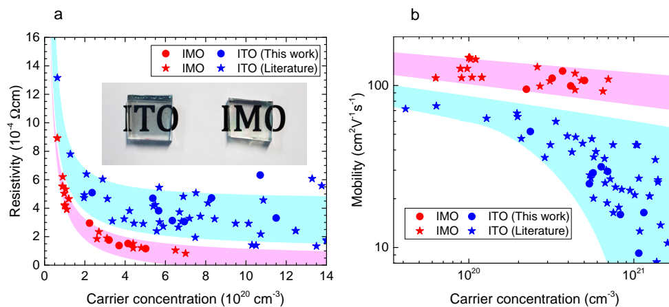
Fig. 2 Transport properties. a Resistivity versus free carrier concentration for polycrystalline ITO and IMO films. Inset shows a photograph of ITO and IMO films. b Hall mobility versus free carrier concentration. Data from this work are circles. Data plotted as stars are taken from the literature for IMO 11–16 and ITO 12,17–22 films. In this carrier concentration regime, the electron mobility is limited by ionized impurity scattering.
