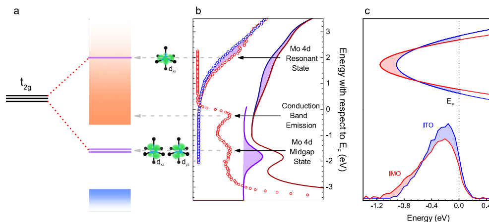
Fig. 5 Spectroscopy of electronic structure. a Schematic diagram of Mo 4d t_{2g} states and their corresponding orbitals (depicted in green), splitting into the upper state, d_{xy} , resonant with the conduction band (orange shading), the two lower states, d_{xz} and d_{yz} , in the band gap and the valence band (blue shading). The splitting resulting from tetrahedral elongation Jahn-Teller distortion of the \text{MoO}_6 octahedron is shown for comparison with the highly distorted \text{Mo}_{\text{In}}^{24\text{d}} depicted in Fig. 4. b Inverse photoemission data from ITO (blue) and IMO (red), showing extra intensity in the IMO data, corresponding to an unoccupied Mo 4d state resonant with the conduction band. Also shown is high energy photoemission data of the conduction band emission, Mo 4d midgap states and valence band onset of IMO. The features in part a of the figure are aligned to the corresponding peaks in the spectra. c Schematic band diagram, showing wavevector (vertical axis) versus energy (horizontal axis) representing the conduction bands of similarly doped IMO (red) and ITO (blue) aligned to the Fermi level. Below are background subtracted HAXPES spectra displaying conduction band emission from IMO (red, n = 5.0 \times 10^{20} \text{ cm}^{-3} ) and ITO (blue, n = 6.3 \times 10^{20} \text{ cm}^{-3} ). The spectra are normalised to the In 5s-dominated valence band peak at -9 eV. The shaded regions emphasise the additional intensity of the ITO peak and additional width of the IMO peak.
