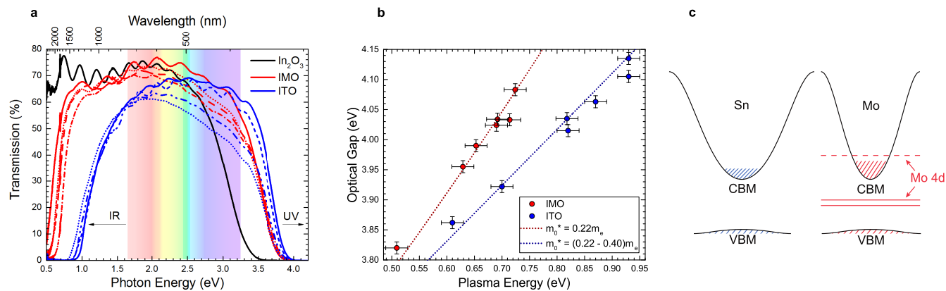
Fig. 3 Optical transmission and associated properties. a Optical transmission of IMO and ITO films (on 3.6 mm-thick soda lime glass) with a range of carrier concentrations, and a nominally undoped In 2 O 3 film, revealing greatly enhanced transparency in IMO due to plasma edges lying at lower energies. b Optical gap versus plasma edge energy of IMO and ITO films, the steeper gradient for IMO indicates a (highly desirable) reduced conduction band minimum effective mass with respect to that of ITO. Model curve lines are calculated using Fermi statistics with a density-of-states averaged effective mass. c Schematic representation of the band structure of ITO (left) and IMO (right) with the same carrier concentration. The IMO has a narrower conduction band dispersion with lower band edge effective mass than ITO and so a higher Fermi level is required to obtain the same number of states as in ITO. In IMO, the resonant and midgap Mo 4d bands are shown, respectively, by the dashed and solid red lines. No Sn state is shown in the ITO band structure schematic as the Sn 5s states mix with the states of the conduction band.
