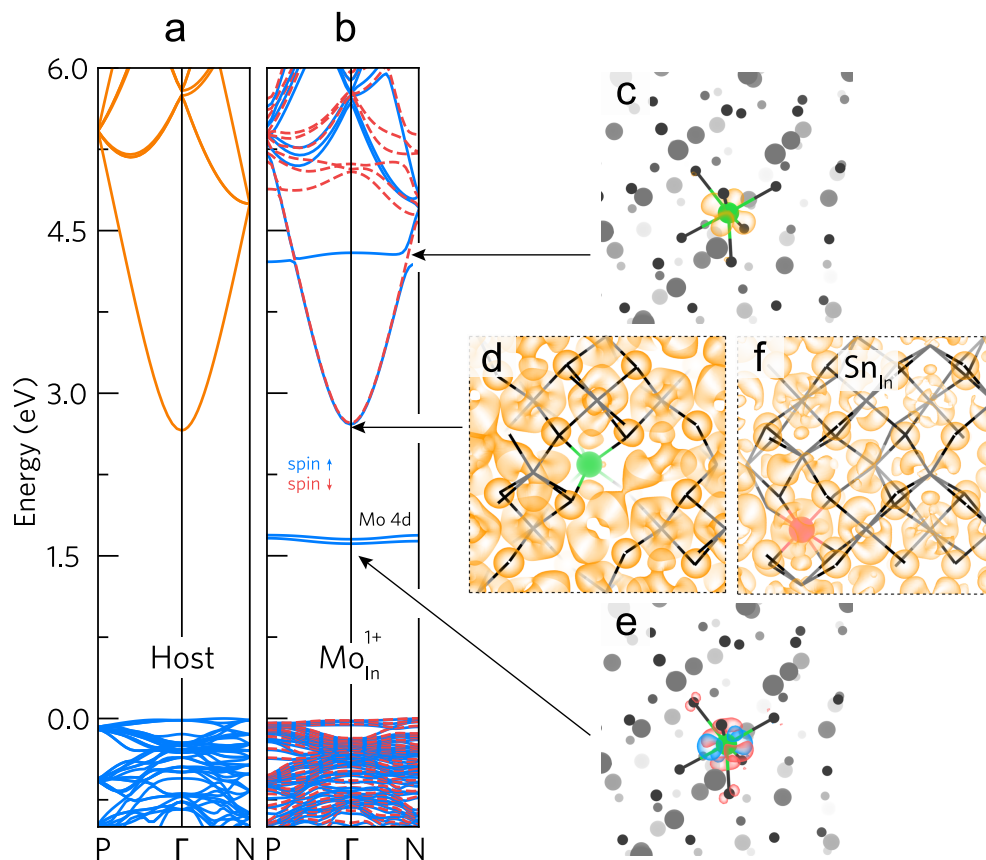
Fig. 4 Band structures and partial charge densities. a and b Band structures for undoped \text{In}_2\text{O}_3 and for IMO, including both spin components, with the Mo donor in the ionized 1+ charge state. The zero of the energy scale is the VBM. c , d and e show the partial charge densities for IMO corresponding to the resonant state in the conduction band, at the CBM and for the two states in the band gap respectively. f The partial charge density at the CBM is also shown for ITO. The \text{Mo}_{\text{In}}^{24\text{d}} atom is green, the \text{Sn}_{\text{In}}^{8\text{b}} atom is red and the \text{In}_2\text{O}_3 lattice is portrayed using a wireframe. For the resonant state and the midgap states, the O and In atoms are shown by black and grey spheres and the 'bonds' on the \text{In}_2\text{O}_3 lattice are removed in order to clearly visualise the \text{MoO}_6 distorted octahedra.
