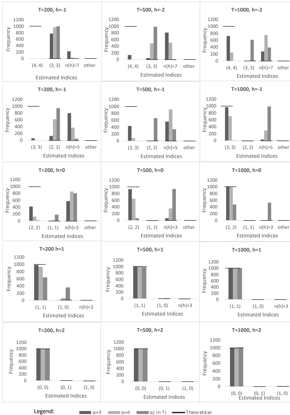
Fig. C: Histogram of the various estimated multistep Kronecker indices in 1000 realizations of Experiment 3
