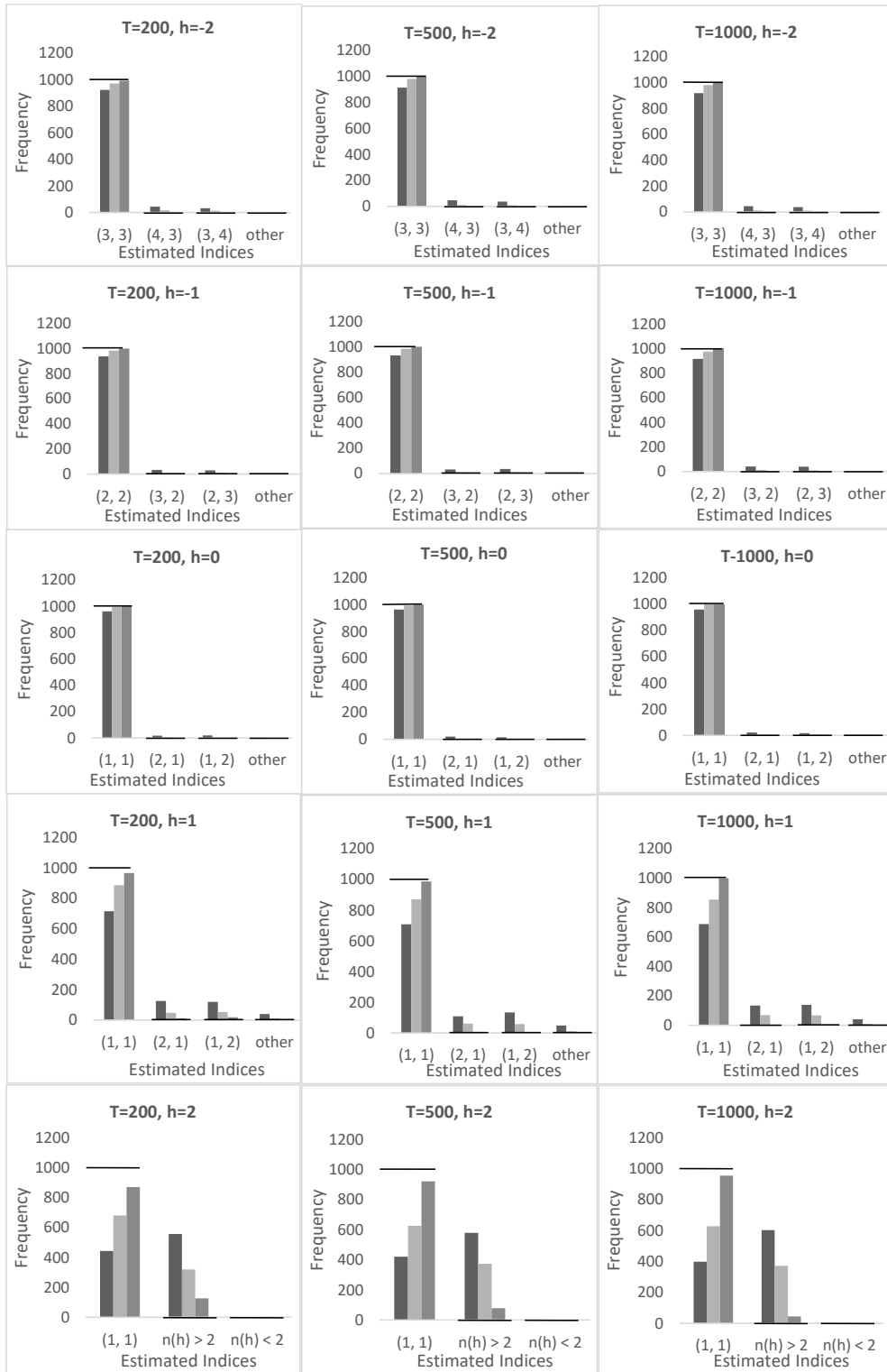
Fig. A: Histogram of the various estimated multistep Kronecker indices in 1000 realizations of Experiment 1
