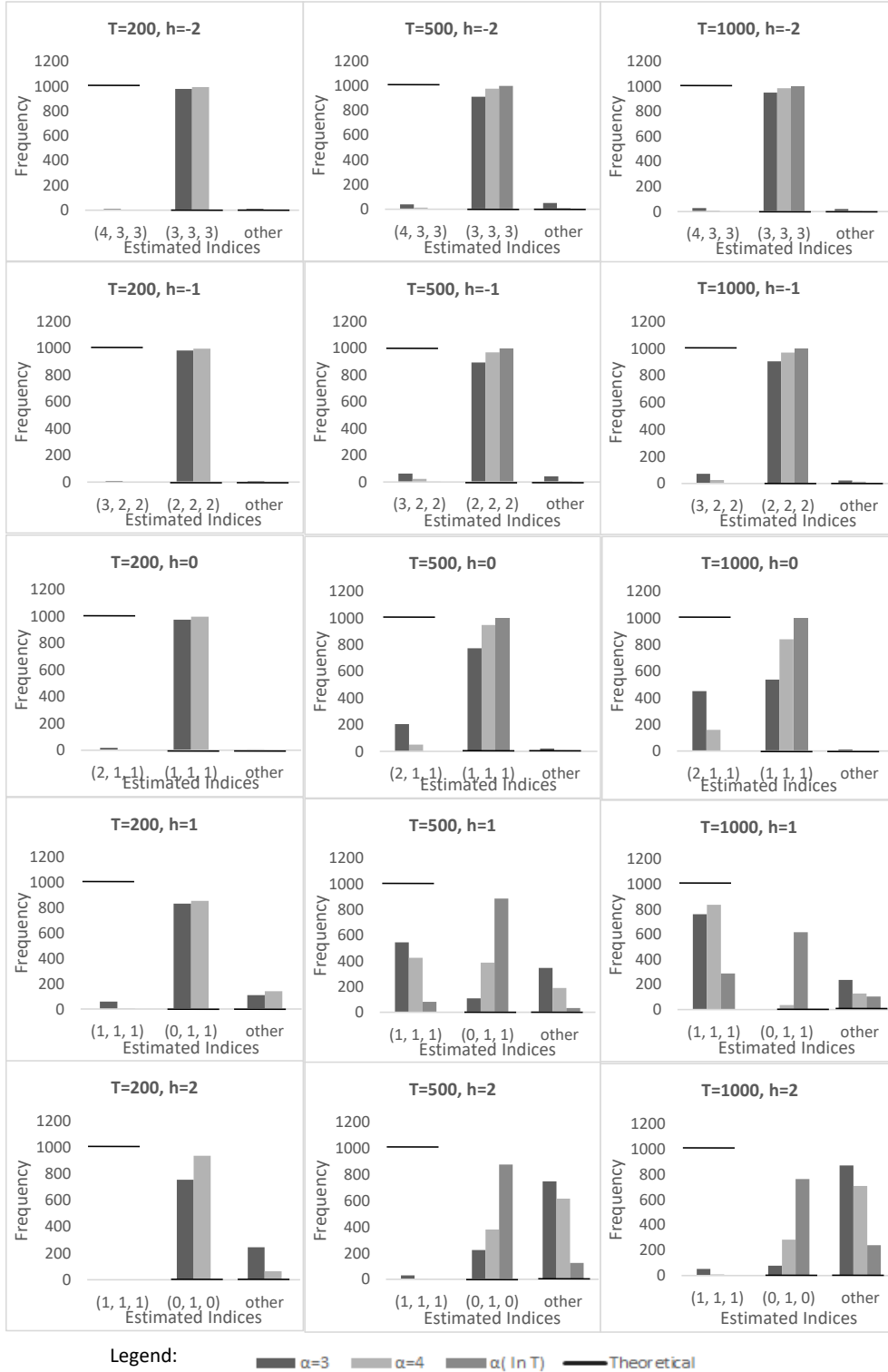
Fig. B: Histogram of the various estimated multistep Kronecker indices in 1000 realizations of Experiment 2
