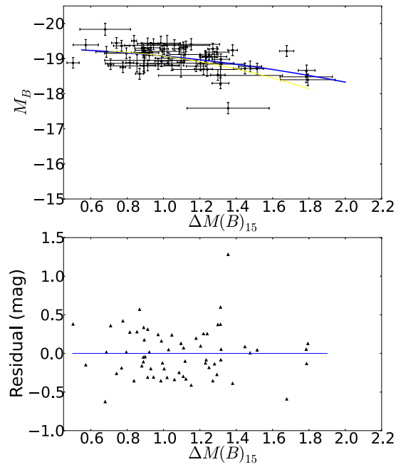
Figure 5. Top: the WLR before reddening correction including only SNe with (B - V)_{B_{\max}} < 0.01 . The blue line of best fit is a second-order polynomial. The yellow model is the line of best fit from Phillips et al. (1999). Bottom: the residuals of the WLR above as a function of \Delta m_{15}(B) .
