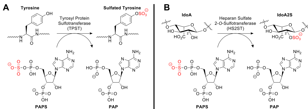
Fig. 1. (A) Tyrosylprotein sulfotransferase catalysed sulfation of a tyrosine residue. (B) Heparan sulfate 2- O -sulfotransferase catalysed sulfation of an iduronic acid (IdoA) subunit of heparan sulfate.
