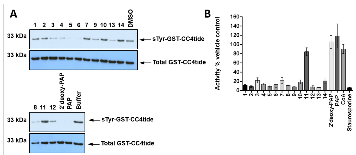
Fig. 5. Immunological evaluation of TPST1 inhibition towards substrate and a Ser/Thr protein kinase counter-screen. (A) Immunoblots evaluating TPST1 sulfotransferase activity in the presence of a panel of PAP- and PAPS-mimetic compounds. GST-CC4-tide (1 \mu g) was incubated in the presence of TPST1 (0.2 \mu g), PAPS (5 \mu M), and a fixed concentration of the indicated compound (400 \mu M) for 15 mins. After termination of the reaction using SDS-PAGE sample buffer, tyrosine sulfation was visualised by immunoblotting using a monoclonal sulfotyrosine antibody (top panel), with equal GST-CC4-tide and TPST1 loading confirmed using an antibody to detect 6xHis tagged proteins (bottom panel). (B) Enzymatic inhibition of PKA catalytic activity by a panel of PAP- and PAPS-mimetic compounds. PKA kinase (1 nM) was incubated with ATP (5 \mu M) in the presence of the appropriate nucleoside analogue (400 \mu M) for 30 min at 20 ^{\circ} C. PKA activity was calculated in real-time using fluorescently-labelled substrate peptide (2 \mu M) and normalised to DMSO (4% v/v) or buffer control (Please Add Byrne et al., PMID: 27444646). Data in B is mean and SD of 3 individual experiments. Staurosporine is included at 40 \mu M as a generic inhibitor of kinase activity. For A, similar results were seen in two independent experiments.
