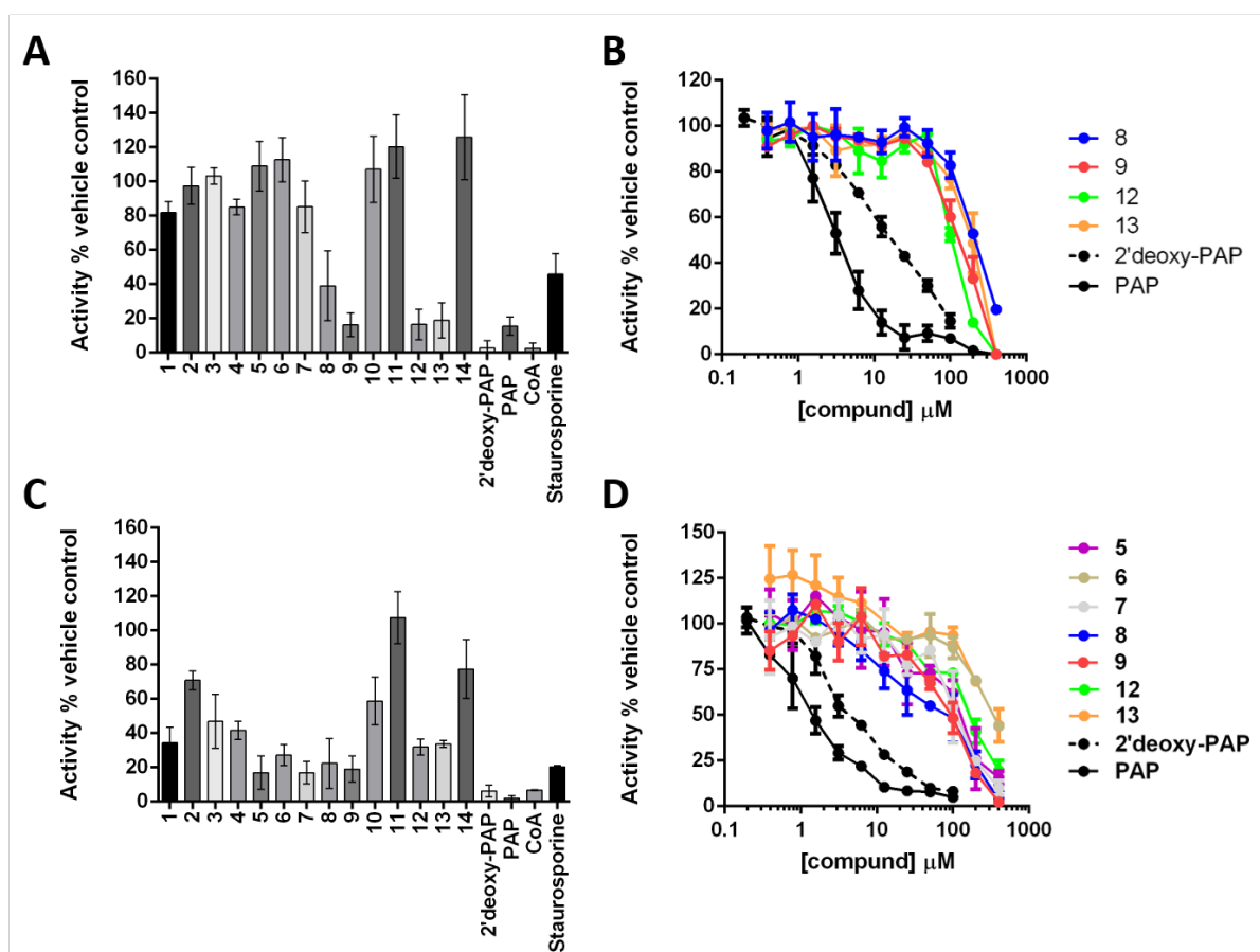
Fig. 4. Summary of enzymatic inhibition assays against HS2ST and TPST1. (A) Enzymatic analysis of HS2ST1 inhibition by a panel of PAP- and PAPS-mimetic compounds. MBP-tagged HS2ST (20 nM) was incubated with PAPS (5 \mu M) in the presence of the appropriate nucleoside analogue (400 \mu M). HS2ST sulfotransferase activity was assayed using a fluorescent hexasaccharide substrate (2 \mu M) and normalised to DMSO (4% v/v) or buffer control. Data shown is mean and SD of 4 repeat experiments. (B) Full dose–response curves for selected compounds. HS2ST (20 nM) was incubated with increasing concentration of the indicated compound in the presence of PAPS (5 \mu M) for 15 min at 20 ^{\circ} C. HS2ST activity calculated as previously described. Data from two independent experiments are combined. (C) Enzymatic analysis of TPST1 inhibition by a panel of PAP- and PAPS-mimetic compounds. TPST1 (0.1 \mu M) was incubated with PAPS (5 \mu M) in the presence of the appropriate nucleoside analogue (400 \mu M) for 30 min at 20 ^{\circ} C. TPST1 activity was measured using fluorescently-labelled CC4-tide (2 \mu M) and normalised to DMSO (4% v/v) or buffer control. (D) Full dose–response curves for selected compounds. TPST1 (0.1 \mu M) was incubated with increasing concentrations of the indicated compound in the presence of PAPS (5 \mu M) for 30 min at 20 ^{\circ} C. TPST1 activity was measured using CC4-tide and normalised to DMSO or buffer controls as previously described. The data shown is from duplicate experiments.
