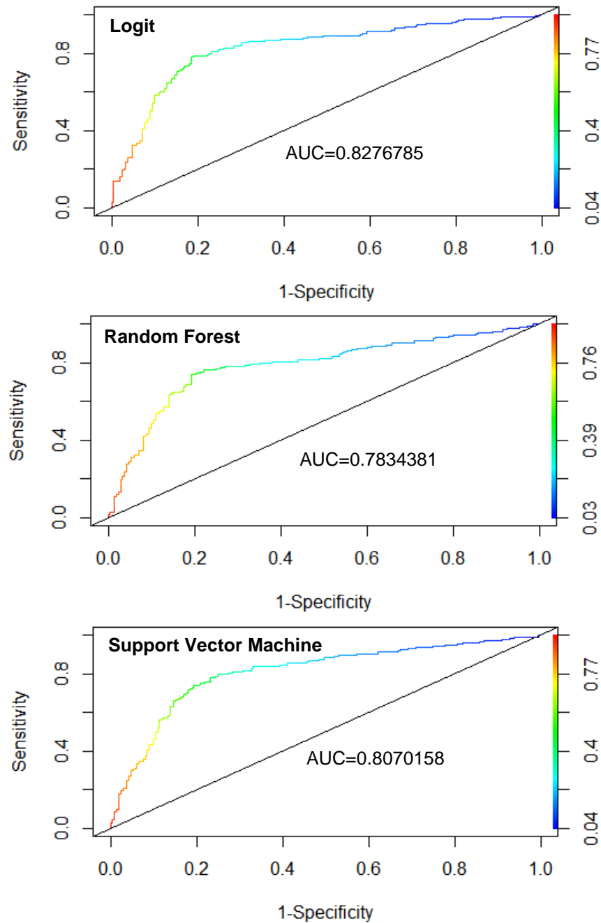
Graph 2. ROC Curves.
