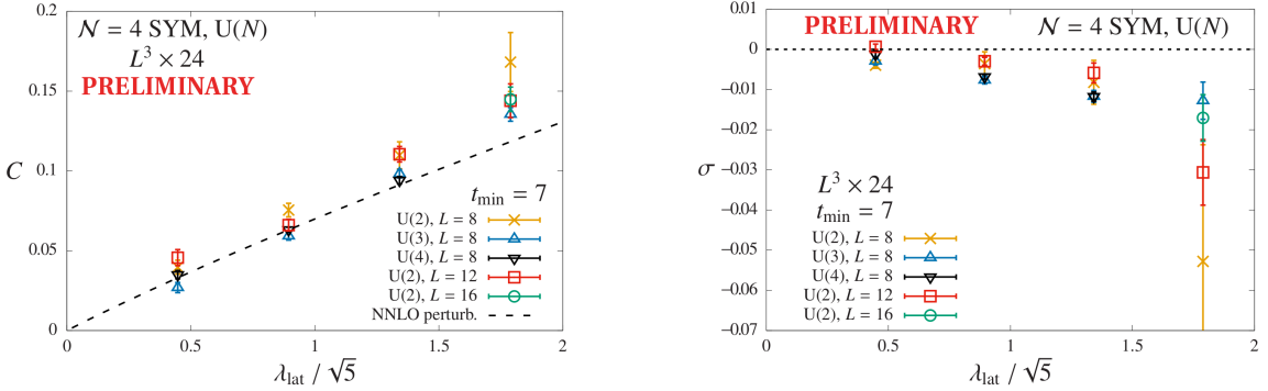
Figure 2: Preliminary lattice \mathcal{N} = 4 SYM results from tree-level improved static potential analyses. Left: The Coulomb coefficient C vs. the 't Hooft coupling \lambda = \lambda_{\text{lat}}/\sqrt{5} on 8^3 \times 24 lattices for U(N) gauge groups with N = 2 (gold \times s), 3 (blue triangles) and 4 (black \nabla s), along with N = 2 results from larger L^3 \times 24 volumes with L = 12 (red squares) and 16 (green circles). The results are consistent with perturbation theory, and the agreement improves with increasing N and L . Right: The string tension \sigma obtained from the same ensembles upon fitting V(r) = A - C/r + \sigma r . The small negative results move toward zero as L increases, confirming that the static potential remains coulombic.
