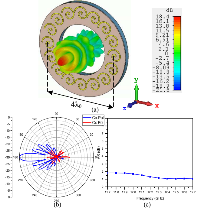
Fig. 6. 16-element circular sub-array (a) 3D radiation pattern (b) 2D radiation pattern (c) axial ratio (broadside radiation)
