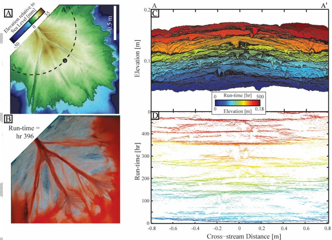
Fig. 8: Experimental data used to explore stratigraphic (in)completeness. The experimental deposit, referred to as TDB-13-S2 [Li and Straub, 2017], evolved in response to a constant supply of water and sediment and a constant rate of sea-level rise. Dynamics were monitored at high spatial and temporal scales relative to morphodynamics with a laser scanner that both captures elevations of the delta and co-registered images of the active surface with flow dyed for visualization. The total run time of the experiment was 500 h, and topography was measured every 1 h. (A) Digital elevation model (DEM) and (B) image of the of the experimental surface at run hour 396. Dashed line A-A' indicates location of transect extracted for analysis. (C) Cross section of synthetic stratigraphy generated from stacked DEMs, clipped for erosion. Deposits are colored by time of deposition. Solid black lines are contours of constant time. (D) Time–space map of preserved elevation for the cross section presented in panel C. White regions in the map represent time–space pairs where either stasis or erosion resulted in a lack of preserved time. A time-lapse movie of the evolution of the experimental surface and flow field can be found at: https://www.youtube.com/watch?v=E3CDyeBahYg&t=43s .
