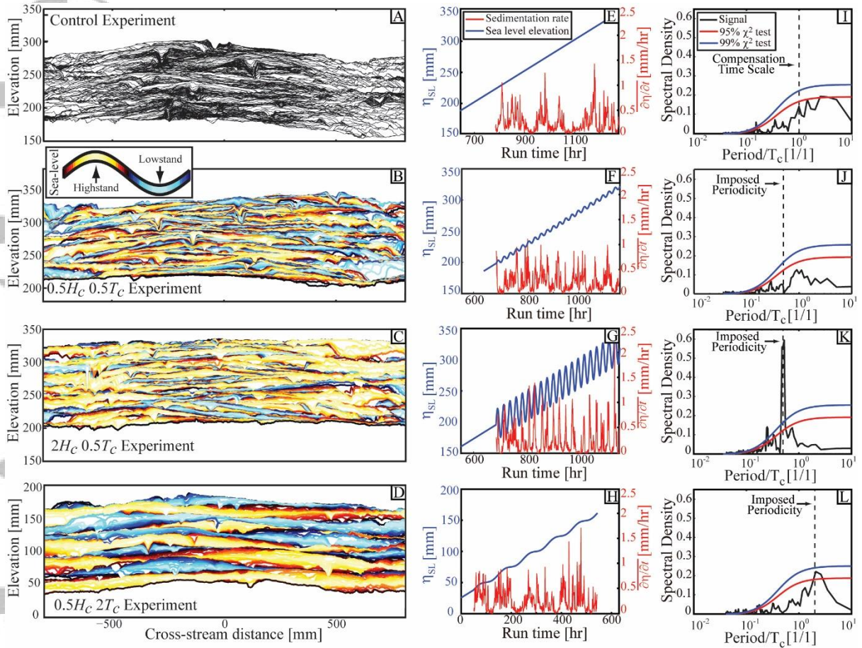
Fig. 15: Results illustrating stratigraphic storage/shredding thresholds for relative sea level (RSL) cycles from Li et al. [2016]. Analysis centers on time series of mean deposition rates measured from preserved experimental stratigraphy along a strike transect located approximately halfway between the basin entrance and mean shoreline. Data from four experiments are presented that share identical forcing conditions, with the exception of the period and magnitude of RSL cycles. The experiments include (A) a control experiment with no RSL cycles, (B) an experiment with cycles defined by a range ( R_{RSL} ) that is half of the largest channel H_c and a period ( T_{RSL} ) that is half of the compensation timescale T_c , (C) an experiment with cycles defined by a R_{RSL} that is twice H_c and a T_{RSL} that is half T_c , and (D) an experiment with cycles defined by a R_{RSL} that is half H_c and a T_{RSL} that is twice T_c . (A–D) Synthetic stratigraphy colored by time of deposition relative to location in RSL cycle. (E–H) Sea level ( \eta_{SL} ) and mean deposition rate ( \delta\eta/\delta t ) time series. (I–L) Power spectra of mean deposition rate time series and \chi^2 confidence limits. Figure modified from Hajek and Straub [2017].
