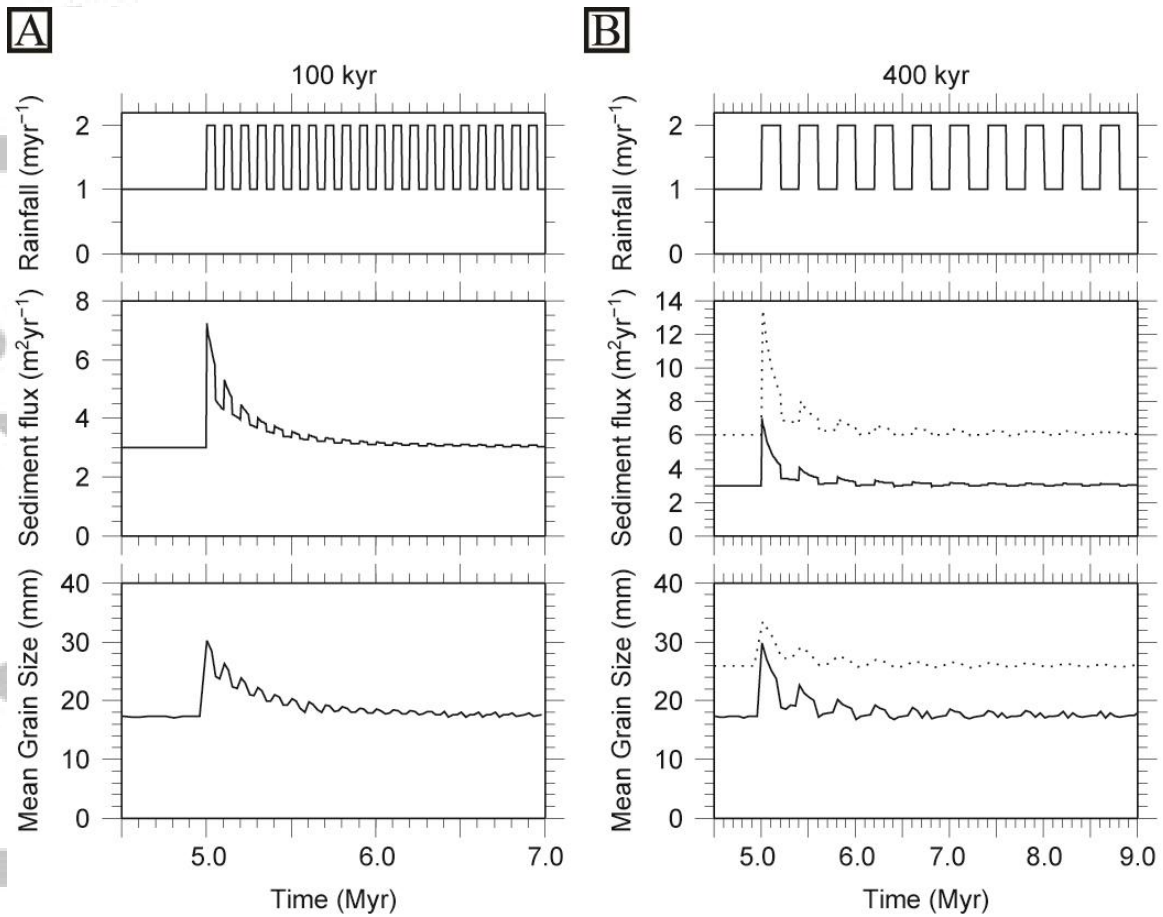
Fig. 5: Diffusional response of catchments. Response in terms of sediment flux and mean grain size to oscillations in precipitation rate with periods a) 100 kyr and b) 400 kyr (dotted lines show sediment flux and mean grain size for a catchment and basin twice as long). After Armitage et al. [2013].
