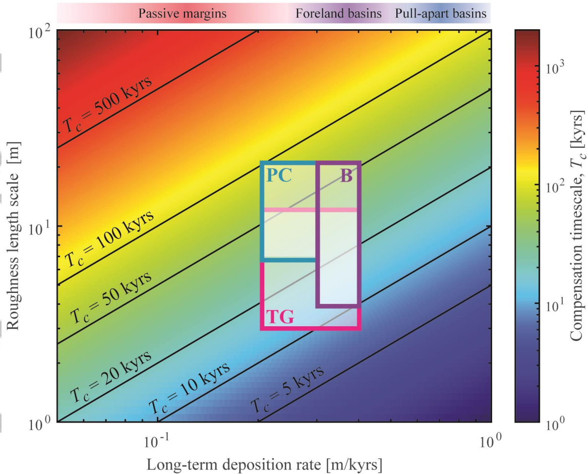
Fig 18: Contoured T_c values for reasonable ranges of landscape roughness and long-term sedimentation rates. Larger roughness length scales and slower sedimentation rates yield longer T_c values. Estimated T_c ranges for the Bighorn Basin, Wyoming, U.S.A. (B), Piceance Creek Basin, Colorado, U.S.A. (PC), and Trempealeau Basin, Spain (TG) (Table 2) indicated in transparent boxes. Approximate characteristic sedimentation-rate ranges for different basin types shown above plot [after subsidence rates of Xie and Heller, 2009 ]. Landscape roughness length scales range from relatively small rivers that might fill, for example, proximal basins (e.g., 1 m-deep flows) to large relief scales (100 m) that would be associated with very large terrestrial rivers, large aggradational deepwater channels, or potentially large-scale relief associated with fluvial or alluvial fans.
