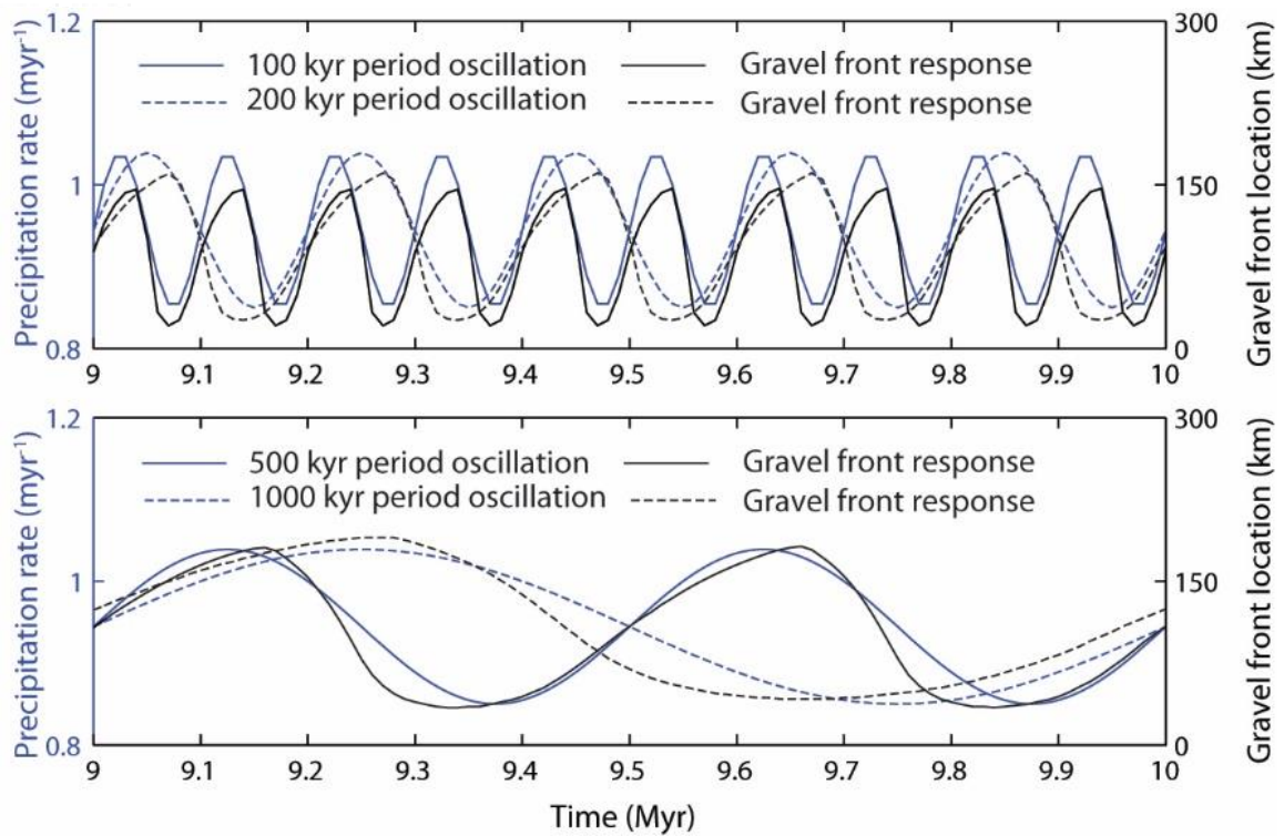
Fig. 4: Response of the gravel front (black lines) to oscillation in precipitation (blue lines) with periods of 100, 200, 500 and 1000 kyr. Note a phase shift between the period of forcing and the periodic gravel front response, which appears to be longer for shorter period oscillations in precipitation rate. After Armitage et al. [2018].
