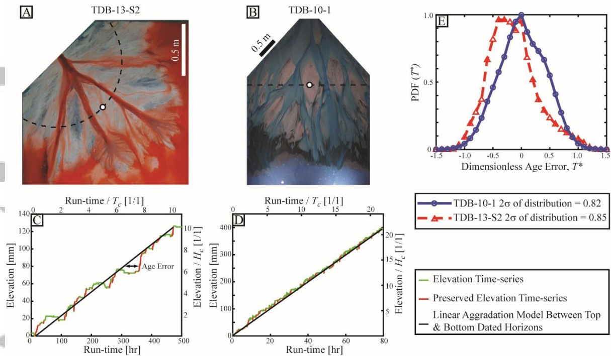
Fig. 12: Measurements of deposit age and linear-age-model-estimated ages from two experiments. (A-B) Images of TDB-13-S2 [Li and Straub, 2017] and TDB-10-1 [Wang and Straub, 2017] experimental surfaces with flow field dyed for visualization. Both experiments evolved in response to constant supplies of water and sediment and constant rates of sea-level rise. However, the magnitudes of these forcings varied in the two experiments by over an order of magnitude, while other properties such as the ratio of water to sediment supply and sediment cohesion varied between experiments. As such, the rates and styles of surface processes varied. Dashed lines indicate location of transects extracted for analysis. Open circles show location of 1-D time series of surface elevation and stratigraphically preserved elevations in the two experiments shown in panels C-D, as well as an age model for experimental stratigraphy constructed with knowledge of the basal and topmost deposit age and assuming linear aggradation between. (E) Distributions defining dimensionless age-error between measured and estimated ages in two experiments from all 1-D transects that comprise cross-sections extracted for analysis. Dimensionless age-error is generated by normalizing measured age-error by compensation timescale.
