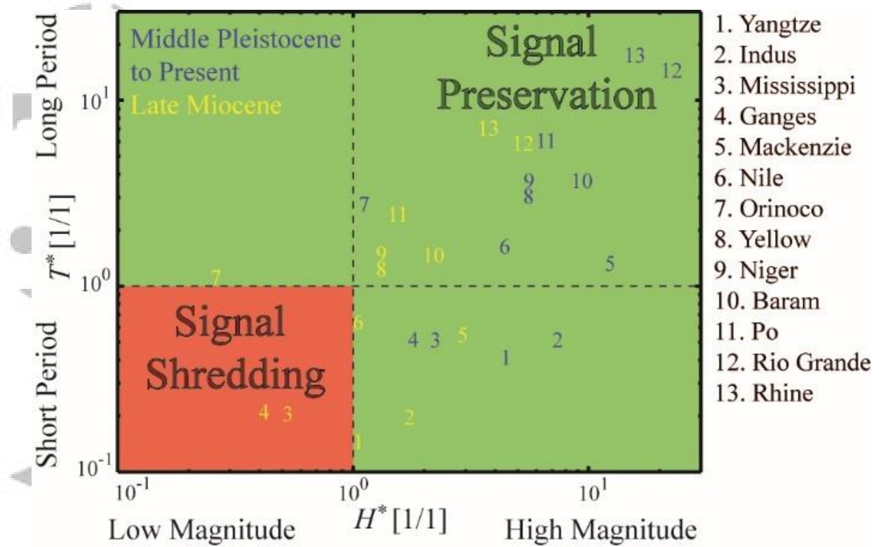
Fig. 16: Predictions of magnitude and period of RSL cycles and their stratigraphic storage potential when normalized by autogenic length and timescales for 13 major river systems. Data originally published by Li et al. [2016]. Predictions are for two time periods, the middle Pleistocene to the present (blue) and the late Miocene (yellow) and are based on modern channel depths and long term (time window of measurement > 100 ky) sedimentation rates.
