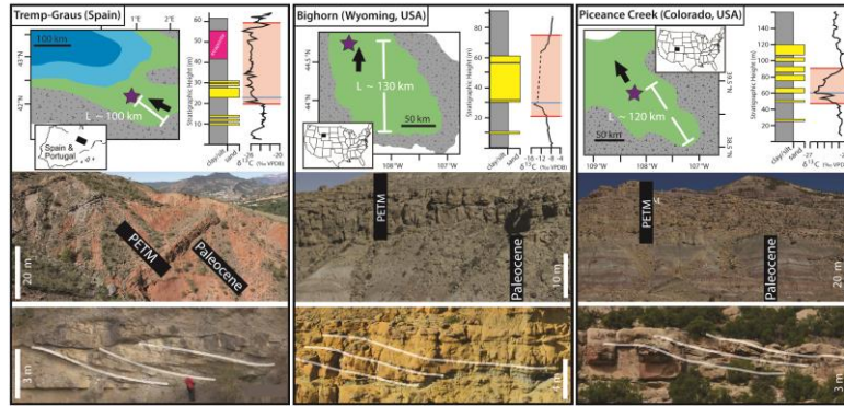
Fig. 19: Example field localities of fluvial deposits spanning the Paleocene-Eocene Thermal Maximum (PETM) in the Tremp-Graus, Bighorn, and Piceance Creek basins. In each panel appears a basin map (top left), stratigraphic sections (top right), a field photo showing large-scale stratigraphic architecture (upper photo) and a close-up photo showing a channel-belt sandstone body (lower photo). Basin maps: Context for constraining key scales associated with signal preservation, for example, depositional system length ( L ), can be estimated from basin dimensions, shown here as the distance from uplifted basement source to the study locality (star) along the path of paleoflow direction (black arrows). Maps and section data after Duller et al., 2019 (Tremp-Graus Basin, Claret Conglomerate section near Tremp, Spain), Foreman 2014 (Bighorn Basin, Willwood Formation near Powell, Wyoming), and Foreman et al., 2012 (Piceance Creek Basin, Wasatch Formation near De Beque, Colorado); paleogeography shown as uplifted source areas in gray, fluvial environments in green, shallow and deep marine in light blue and dark blue. Stratigraphic logs show architecture through PETM intervals in each basin; onset of coarse-grained deposition noted with blue line. Carbon-isotope sections show moving averages of sampled data through the intervals represented by the stratigraphic logs; onset and termination of the PETM-defining carbon-isotope excursion indicated by red lines. This comparison shows the apparent lag between the onset of the PETM and the stratigraphic response. This lag time was quantified by Duller et al. [2019] and provides insight into landscape-response times. Overview photos: Each basin shows a marked coarsening of overall stratigraphic architecture in the vicinity of the PETM [Baisden, 2014; Greenberg, 2016]. Close-up photos: Example channel-belt sandstone bodies from each basin with preserved bar-clinoform deposits (highlighted with white lines) that can be used to approximate paleo-flow depths.
