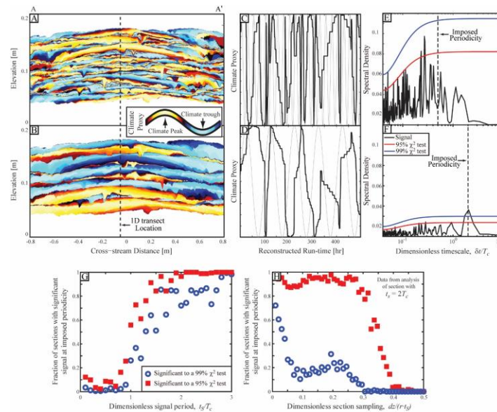
Fig. 13: Results illustrating stratigraphic storage thresholds of environmental proxies in stratigraphy. Analysis utilizes synthetic stratigraphic panel shown in figure 8C. Each 1-D topographic sample location along strike section samples an environmental signal, which for simplicity follows a sinusoidal cycle. The amplitude of this cycle is held constant, but the period is altered systematically. Stasis, erosional and depositional events of varying duration and magnitude convert continuous environmental signal into a proxy record discretized into stratigraphic beds. Strike sections of stratigraphy colored by magnitude of proxy for environmental signals with periods equal to 0.5T_c (A) and 2T_c (B). Movie documenting evolution of strata in time and sampling of proxy can be found at: https://www.youtube.com/watch?v=-I94NTIZT8A . 1-D Preserved climate proxy records (C&D) show mismatch between reconstructed time series of proxy (solid black line) and imposed environmental signal (light gray line). Reconstructed time is generated with age of basal and top-most deposits and linear age-model between. Power spectra of reconstructed proxy time series and \chi^2 confidence bands show storage of 2T_c signal (E), but no significant signal in 0.5T_c stratigraphy (F). Analysis of environmental signals with a range of periodicities (G) demonstrate reliable storage of environmental signals in proxy records when period of signal is greater than or equal to 2T_c . For strata that reliably house environmental signals in proxies, vertical sample spacing must be less than a dimensionless sample spacing of 0.25 to recover signal (H). Sample spacing is made dimensionless by dividing by the product of the long term aggradation rate and the period of the signal to be recovered.
