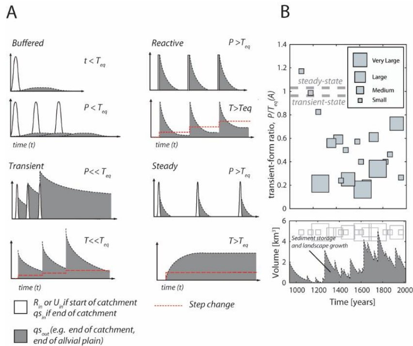
Fig. 3: Terminology for defining landscape response to changes in boundary conditions.
