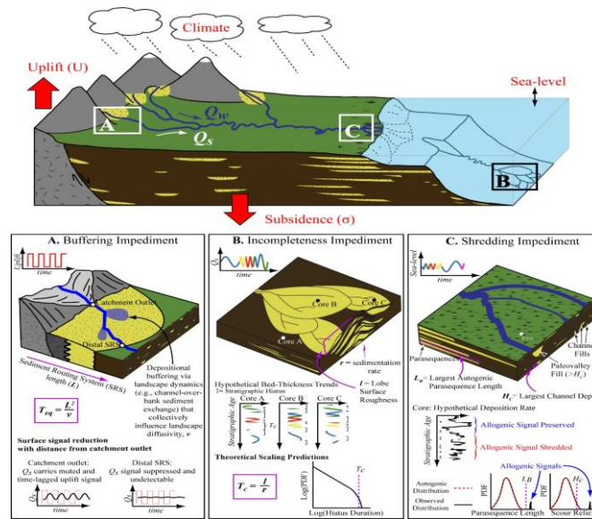
Fig. 1: Conceptual diagram of a sediment routing system (SRS) and the major impediments to stratigraphic storage of environmental signals. SRSs transport sediment from erosional sources to depositional sinks and are sensitive to environmental forcings (climate, tectonics, sea-level). Propagation of signals of these forcings across the Earth-surface and into the stratigraphic record are influenced by three primary impediments shown in schematic form in sub-panels. Each impediment can affect any section of a SRS, but for simplicity we highlight just one impediment per transport-system segment. (A) The propagation of environmental signals is buffered via the interaction of channels with landscapes. For example, step changes in tectonic uplift experienced in catchments produce muted sediment flux signals with time-lags at catchment outlets. These sediment flux signals become more muted with additional transport through fluvial SRSs. The amount of buffering can be predicted by comparing the duration or period of an environmental forcing with a system's equilibrium timescale ( T_{eq} ). (B) The stochastic relocation of SRSs, for example through depositional lobe avulsions in deep-water systems, can convert a continuous input sediment supply signal into a discrete and discontinuous record with time preserved in sedimentary beds separated by gaps or hiatuses of nondeposition. The duration of these hiatuses is limited by the system's compensation timescale ( T_c ). (C) Cut-and-fill processes in net depositional settings can shred environmental signals prior to stratigraphic storage by smearing input signals through space and time. When environmental forcings, for example changing sea-level, have magnitudes and periods less than autogenic timescales they are prone to shredding. As such, stratigraphic scales, for example deposition rates, parasequences or scours associated with the forcing, might be indistinguishable from autogenic stratigraphic scales.
