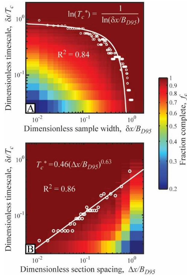
Fig. 14: Results illustrating how stratigraphic completeness is a function of both timescale of discretization and lateral field of view. (A) Phase space defining how stratigraphic completeness changes as a function of dimensionless timescale of discretization and dimensionless sample width. Open circles reflect timescale necessary to reach 100% completeness for a given width of observation. Solid white line is theoretical trend which is defined by Eq. 9, while R^2 value characterizes fit of Eq. 9 to the data. (B) Phase space defining how stratigraphic completeness changes as a function of dimensionless timescale of discretization and dimensionless 1-D section spacing. Open circles reflect timescale necessary to reach 100% completeness for a given section density. Solid white line is empirical fit to data, which is defined by Eq. 10, while R^2 value characterizes quality of regression. Both phase spaces are generated with data set shown in figure 8C.
