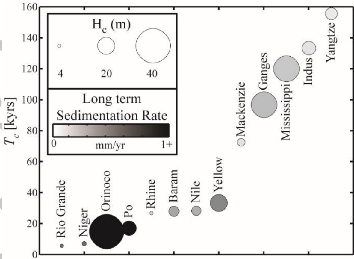
Fig. 11: Compensation timescale estimates for compilation of 13 modern delta systems. Estimates calculated with published data on channel depth and long-term deposition rate (measurement interval in excess of 100 kyr). Size of circle scales with the depth of a system's channels while grayscale value of filled circles scales with the long-term sedimentation rate of a basin. Modified from Straub and Wang [2013].
