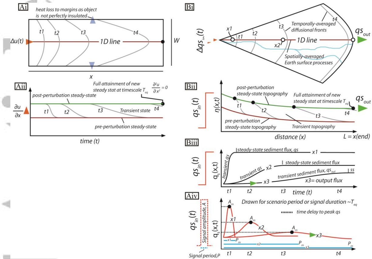
Fig. 2: Schematic of processes and timescales important in diffusion of signals. A) i, 2D view of a homogenous and isotropic solid medium illustrating the diffusion of heat following a step change increase in the rate of heat input. ii, the time-dependent response of the system from the initial or pre-perturbation steady-state condition (red line) to the post perturbation steady-state condition (green line). Note that the system is still in transient response or transient-state until the new steady state has been achieved. The time taken to reach this new steady state, or the response time T_{eq} , is related to the material properties, amplitude of perturbation and the dimensions of the solid medium. B) i, ii, 2D Map view of a spatially and temporally averaged (so homogenous and isotropic) diffusional fluvial landscape showing the position of diffusional fronts and time-dependent response of the system following a step change in sediment flux, q_{sin} . iii, time dependent response, to this step-change in terms of q_s , at 3 positions ( x_1 , x_2 & x_3 see Bi) as a function of time. iv, time dependent response of the system, in terms of q_s , shown at 3 positions ( x_1 , x_2 & x_3 see Bi) to a single spiked perturbation of q_{sin} of duration \sim T_{eq} . Note the reduction in magnitude of the signal and the increase in duration of the signal as it travels down-system. A_m , modified amplitude, P_m , modified period.
