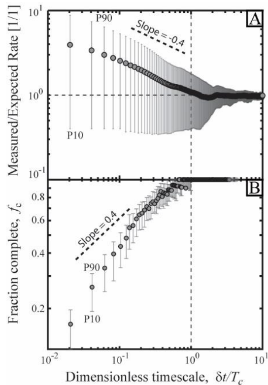
Fig. 10: Data defining the Sadler effect and stratigraphic (in)completeness measured from experimental stratigraphy. (A) Rate of deposition as a function of duration of observation measured from synthetic stratigraphic data set shown in figure 8C. Measured rates are normalized by an expected rate which equals the rate of accommodation production facilitated by long term base level rise. Duration of observation is normalized by the compensation timescale, T_c . Symbols represent mean value of all positive rates measured at a given timescale, while vertical bars represent \pm one standard deviation of distribution that defines the variability in the rate at that timescale. (B) Completeness of stratigraphic data as a function of discretization timescale. Symbols represent mean completeness value at a given timescale from all 1-D sections in data set, while vertical bars represent \pm one standard deviation of distribution that defines the variability in completeness from all 1-D sections. A movie that documents the generation of strata along the strike section shown in figure 8C colored by deposit age, and corresponding Wheeler diagram that denotes when and where time is stored in the section can be found at: https://www.youtube.com/watch?v=4uaVo_EdaB0&t=6s .
