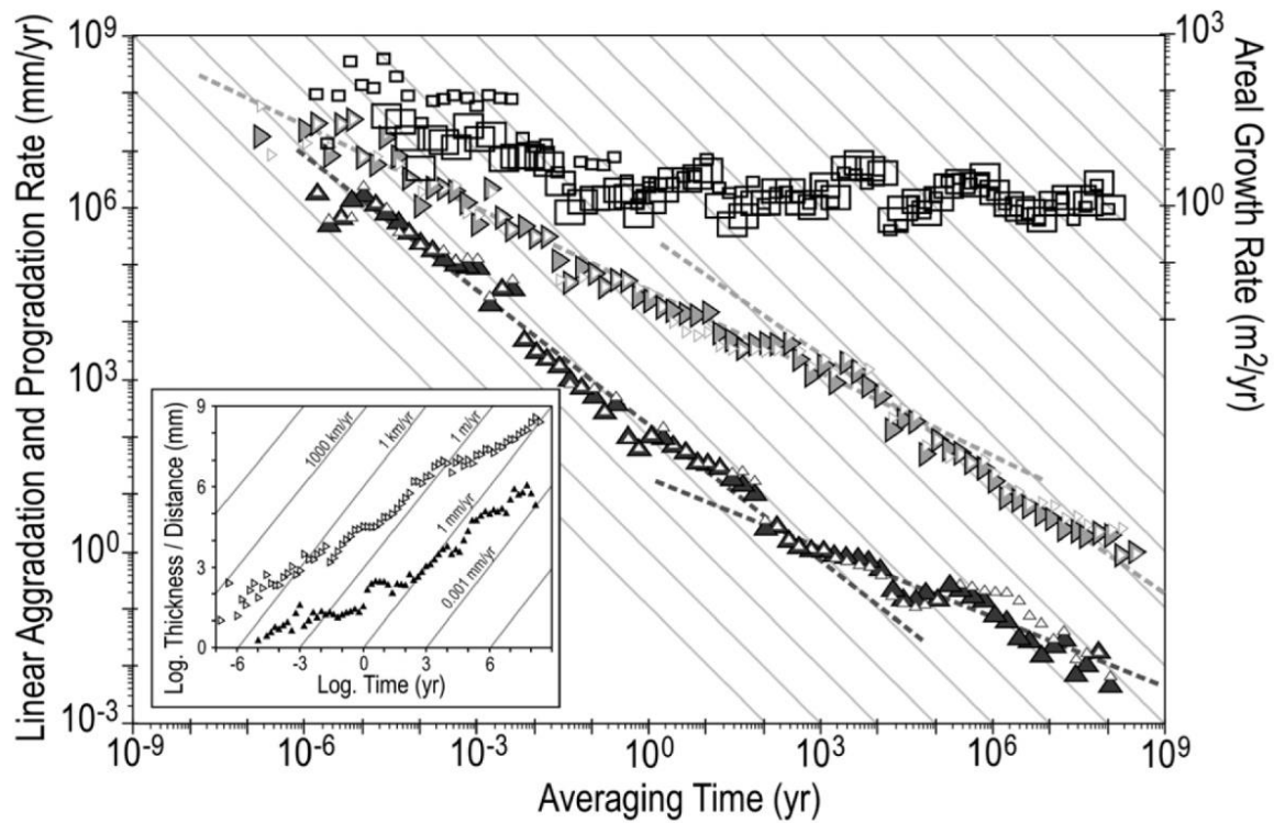
Fig. 7: Compilation of 1-D aggradation and progradation rates and expected sediment flux as a function of measurement duration. Reproduced from Sadler and Jerolmack [2015] with permission of authors. Upward-pointing triangles plot aggradation rates while forward-point triangles plot progradation rates. Expected sediment flux, plotted as squares, expressed as volume discharge per unit width of the transport system does not vary systematically from timescales of months to one hundred million years. These growth rates are not empirical field estimates; they are products of expected aggradation and progradation components determined separately from mean empirical values. Inset: Unsteady increase of expected progradation distance and aggradation thickness as a function of time span.
