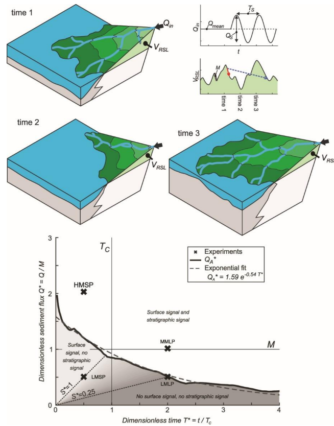
Fig. 17: Processes responsible for stratigraphic shredding of sediment-flux signals and their quantification. Set of schematic diagrams illustrate aggradational delta at three different time steps. Even under constant sediment supply rate ( Q_{in} ), the volume stored above sea level ( V_{RSL} ) continually adjusts in response to autogenic sediment storage bypass and release (SSBR). Schematic graphs show a cyclic sediment supply signal and expected autogenic changes in V_{RSL} . The rate of V_{RSL} change generally decreases with the time window measured over (e.g., red vs. dashed blue arrow) and approaches zero over long timescales. The magnitude and period of these autogenic SSBR events set a signal storage threshold which is dependent on the timescale of a signal. Plot at base defines the stratigraphic storage threshold of sediment flux signals for an experimental system and is based off measurement of autogenic change in a delta that evolved in the absence of sediment flux signals. Crosses mark combinations of periodicity and peak-to-peak amplitude for cyclic experimental stages. Analysis of stratigraphy supports the signal threshold theory, with experiments plotting above the threshold storing signals in their stratigraphy and experiments that plotted below the threshold lacking any stratigraphic signals of periodic supply signals. Modified from Toby et al. [2019].
