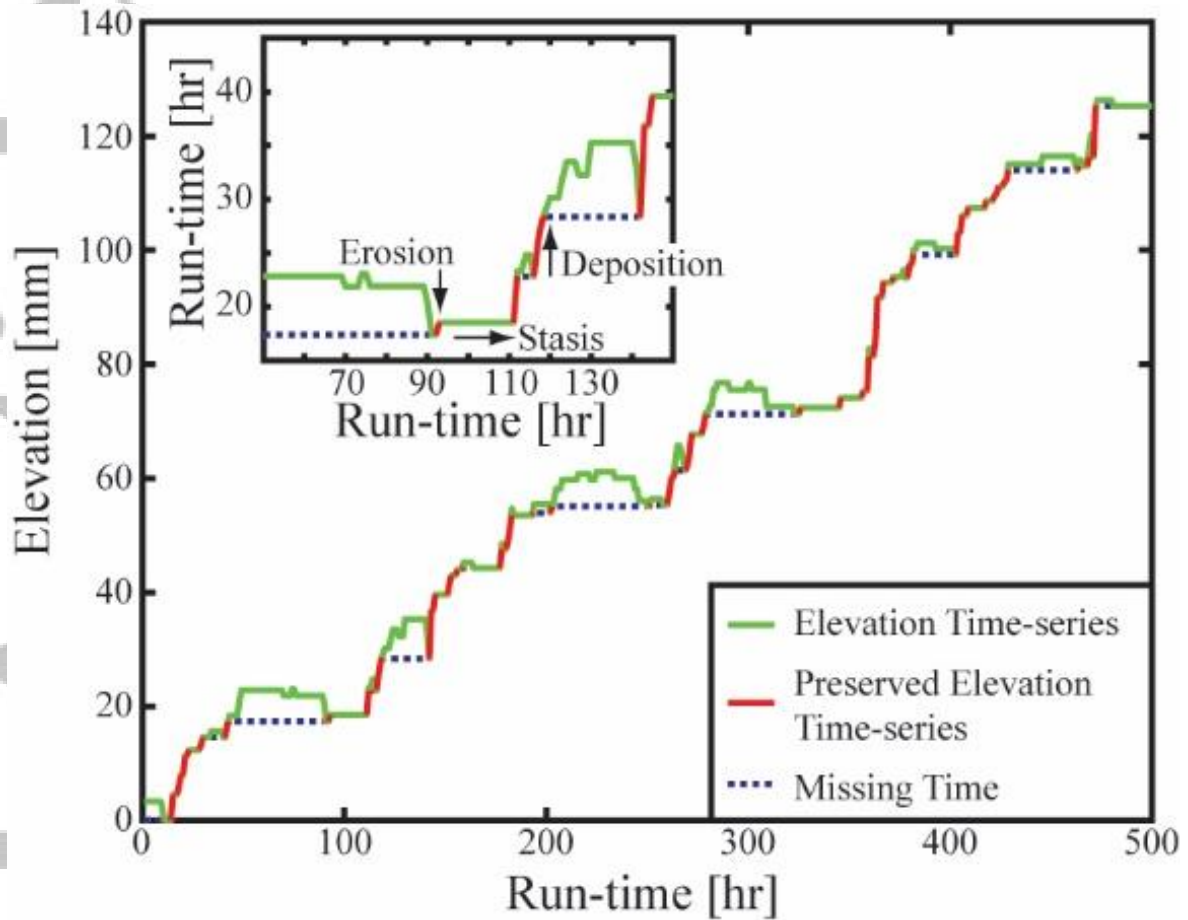
Fig. 9: Data defining the 1-D evolution of topography and resulting stratigraphy for a system that exhibits long-term net deposition, but over shorter periods experiences discrete episodes of deposition, erosion and stasis. 1-D transect is extracted from mid-point of topographic data set presented in figure 8C.
