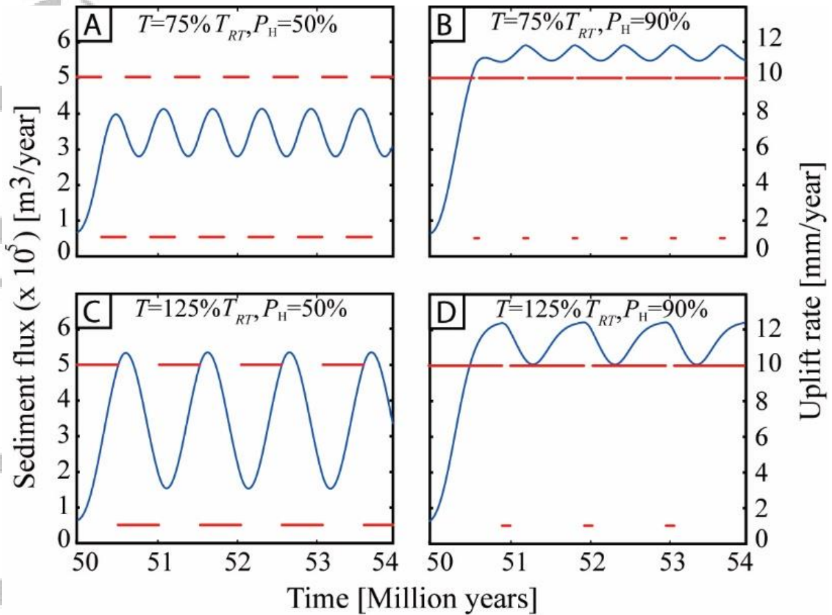
Fig. 6: The advective response of catchments, in terms of a time series of sediment flux to oscillations in uplift, scaled to a catchment response time, T_{RT} . Red lines represents the time series of uplift, and blue lines represent sediment flux at the catchment outlet; the catchment response proxy. P_H , percentage of the period during which uplift rate is high. After Li et al. [2018].
