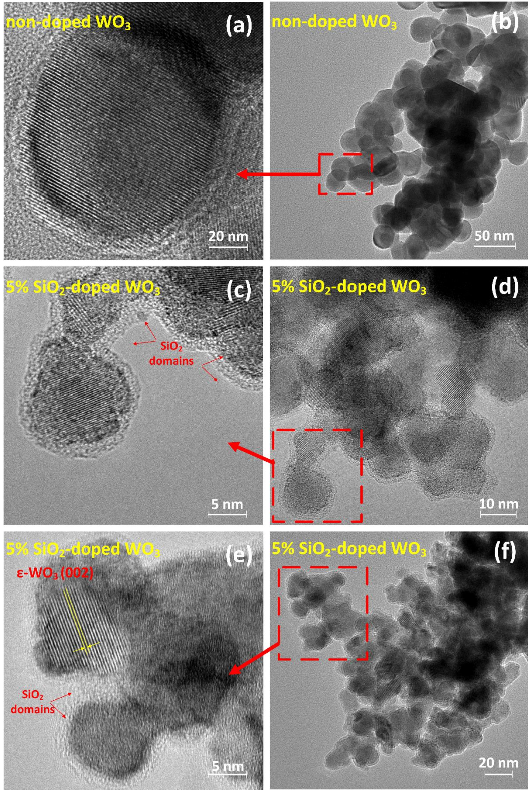
Fig. 8.9: High resolution transmission electron microscopy of the post annealed \text{WO}_3 film. (a)-(b) non-doped \text{WO}_3 , (c)-(f) 5 wt% \text{SiO}_2 doped \text{WO}_3 .
