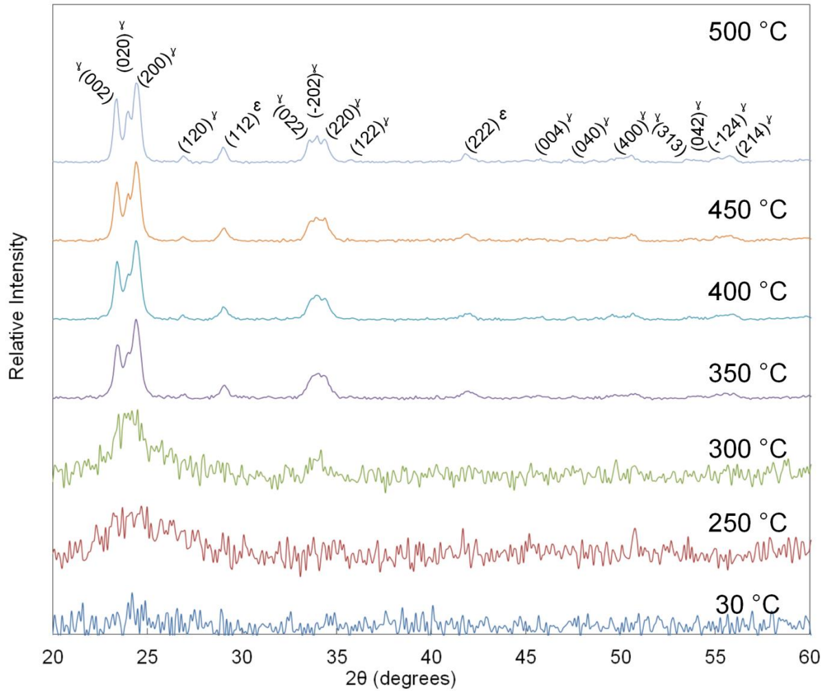
Fig. 7.7: XRD spectra of sample C during annealing from 30–500°C.
