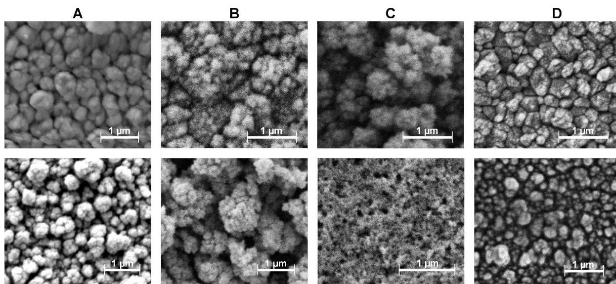
Fig. 7.3: Scanning Electron Microscopy micrographs of WO 3 films deposited by RSDT under condition A, B, C and D. (Top: as deposited, Bottom: after annealing at 500°C).
