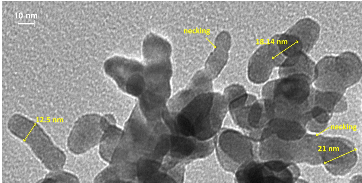
Fig. 10.7: TEM micrographs of the \text{WO}_3 crystallites showing necking and a crystallite size ( d_{\text{TEM}} ) distribution ranging between 12–25 nm.
