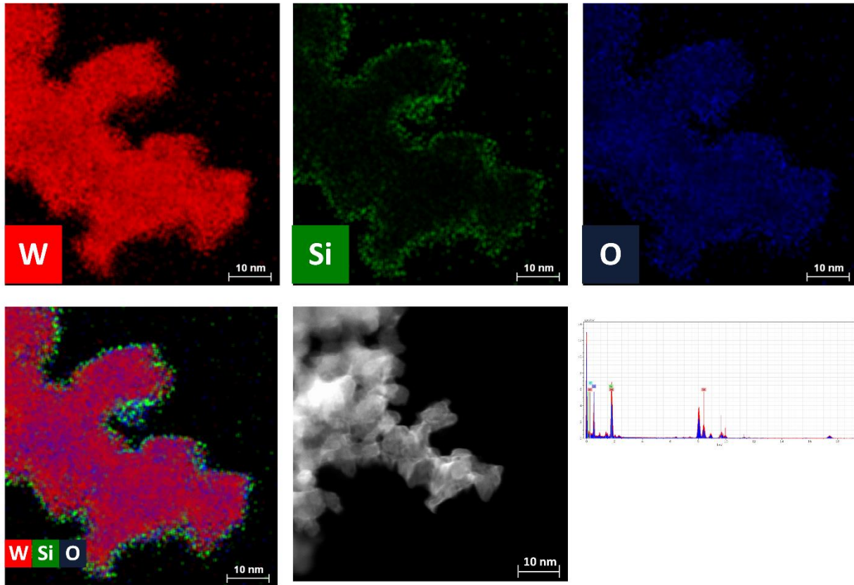
Fig. 8.10: X-ray energy dispersive spectroscopy (XEDS) elemental maps for 5 wt% SiO 2 doped WO 3 along with the scanning transmission electron microscopy (STEM) image.
