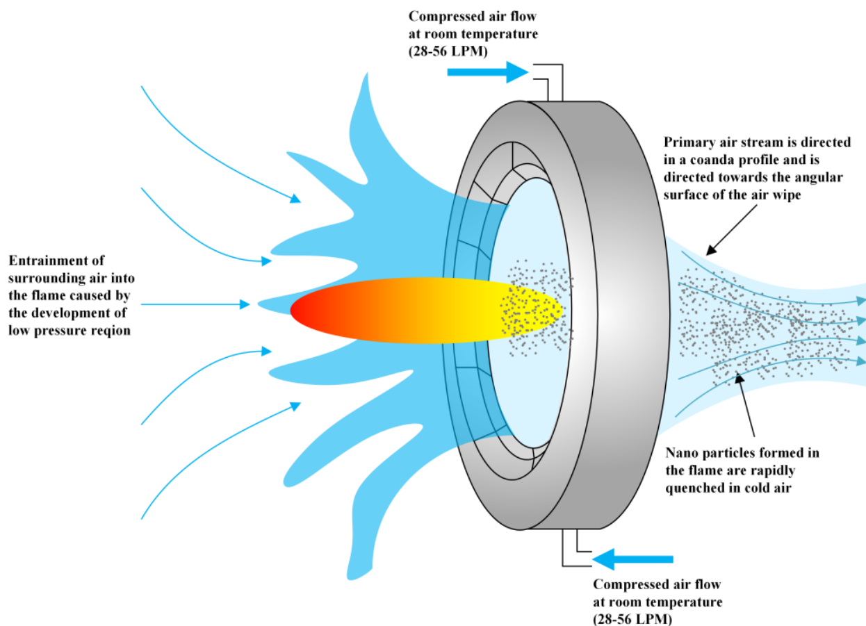
Fig. 1.3: Schematic of air quenching mechanism and the coanda profile in RSdT.
