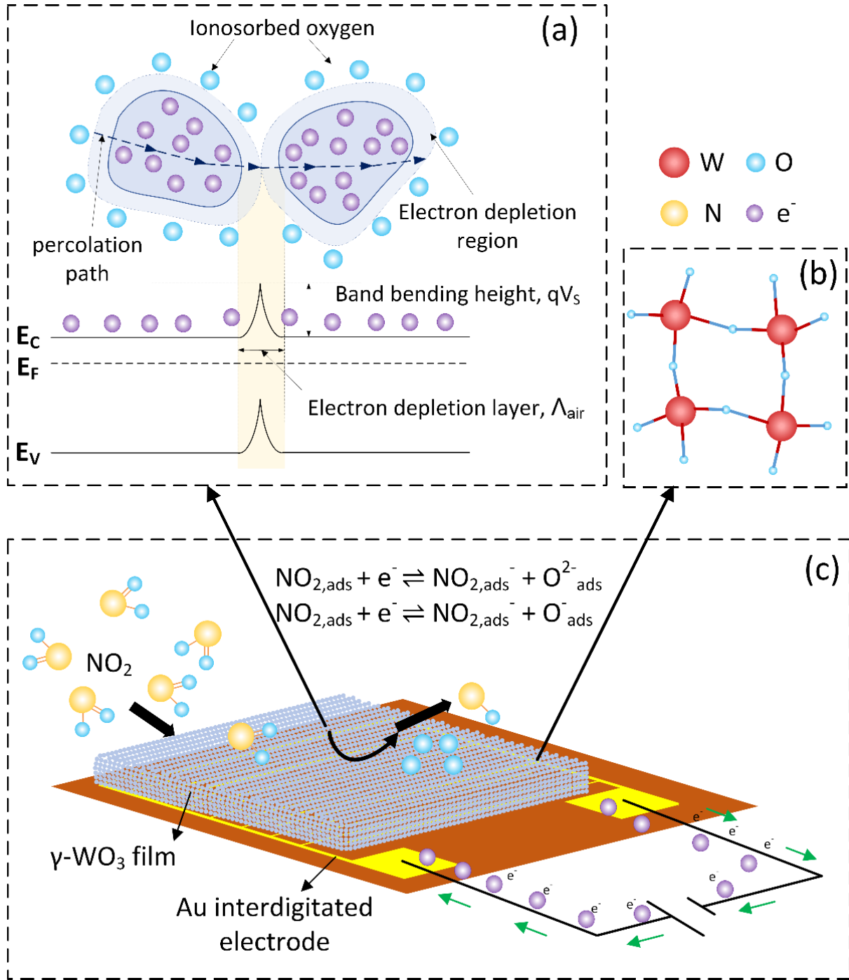
Fig. 4.2: Simplified model explaining the NO_2 sensing phenomenon by monoclinic \gamma - WO_3 . (a) Band bending after ionosorption of oxygen. E_C , E_F and E_V denotes the energy of conduction band, Fermi level and valence band respectively. qV_s and 2\Lambda_{gas} denotes the band bending height and thickness respectively. (b) Structure of \gamma - WO_3 . (c) \gamma - WO_3 thin film deposited on a gold interdigitated electrode.
