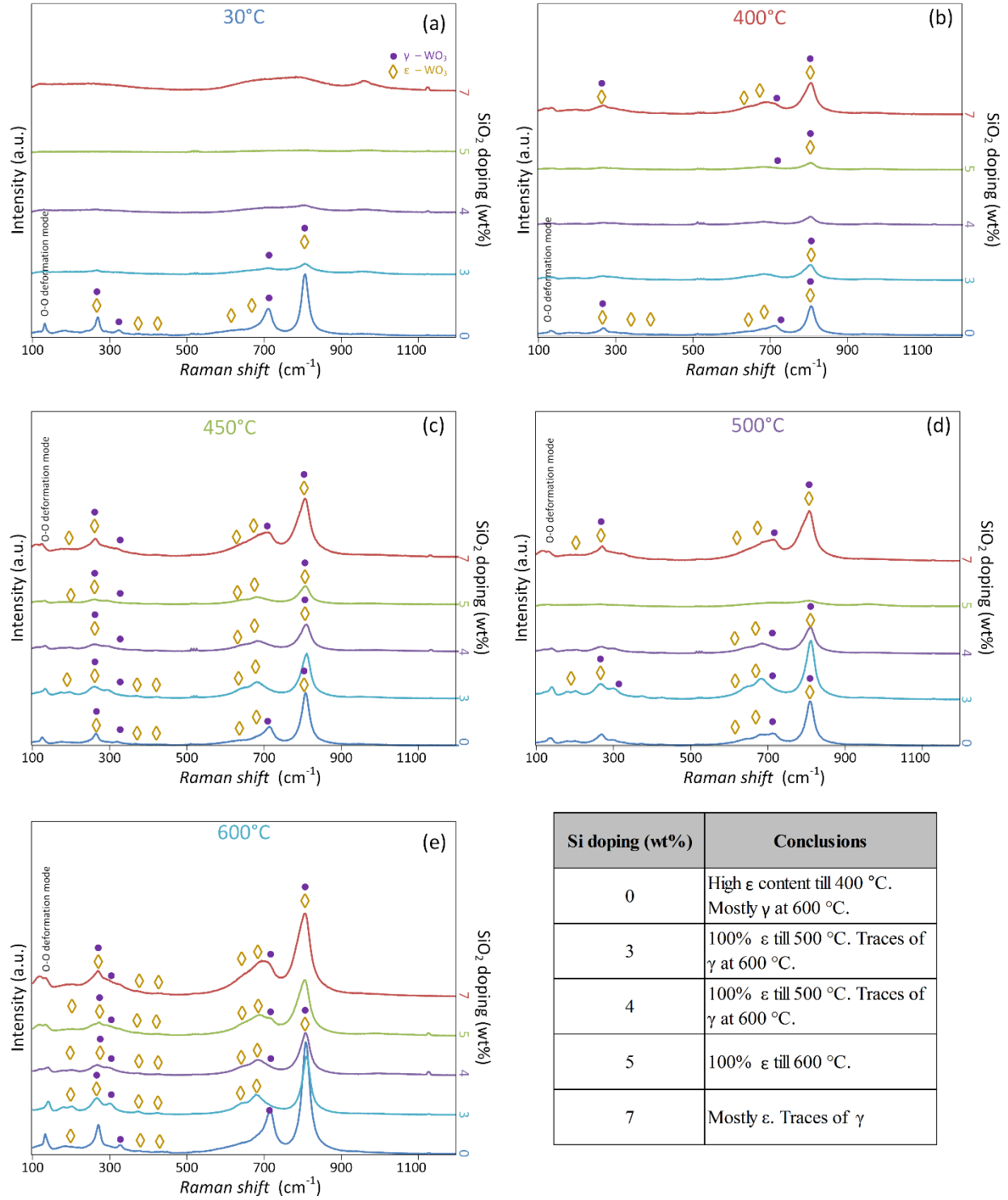
Fig. 8.7: (a)-(e) The Raman spectroscopy of the post annealed WO 3 film arranged according to the post annealing temperature.
