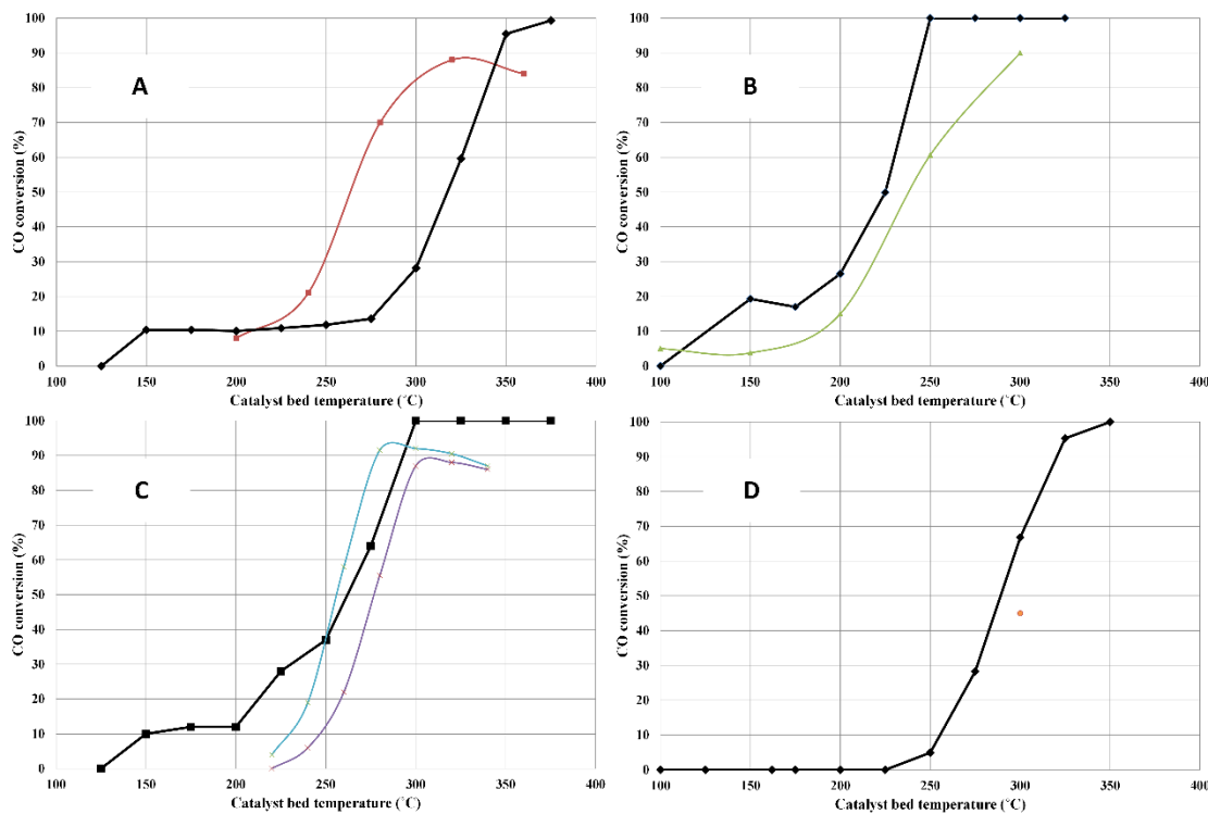
Fig. 5.7: Water-gas shift reaction activity of RSDT made catalysts as compared with literature (conventional wet chemistry based catalysts). A, B, C and D: WGS reaction activity tested with similar conditions as references [9], [6], [7] and [8] respectively.
