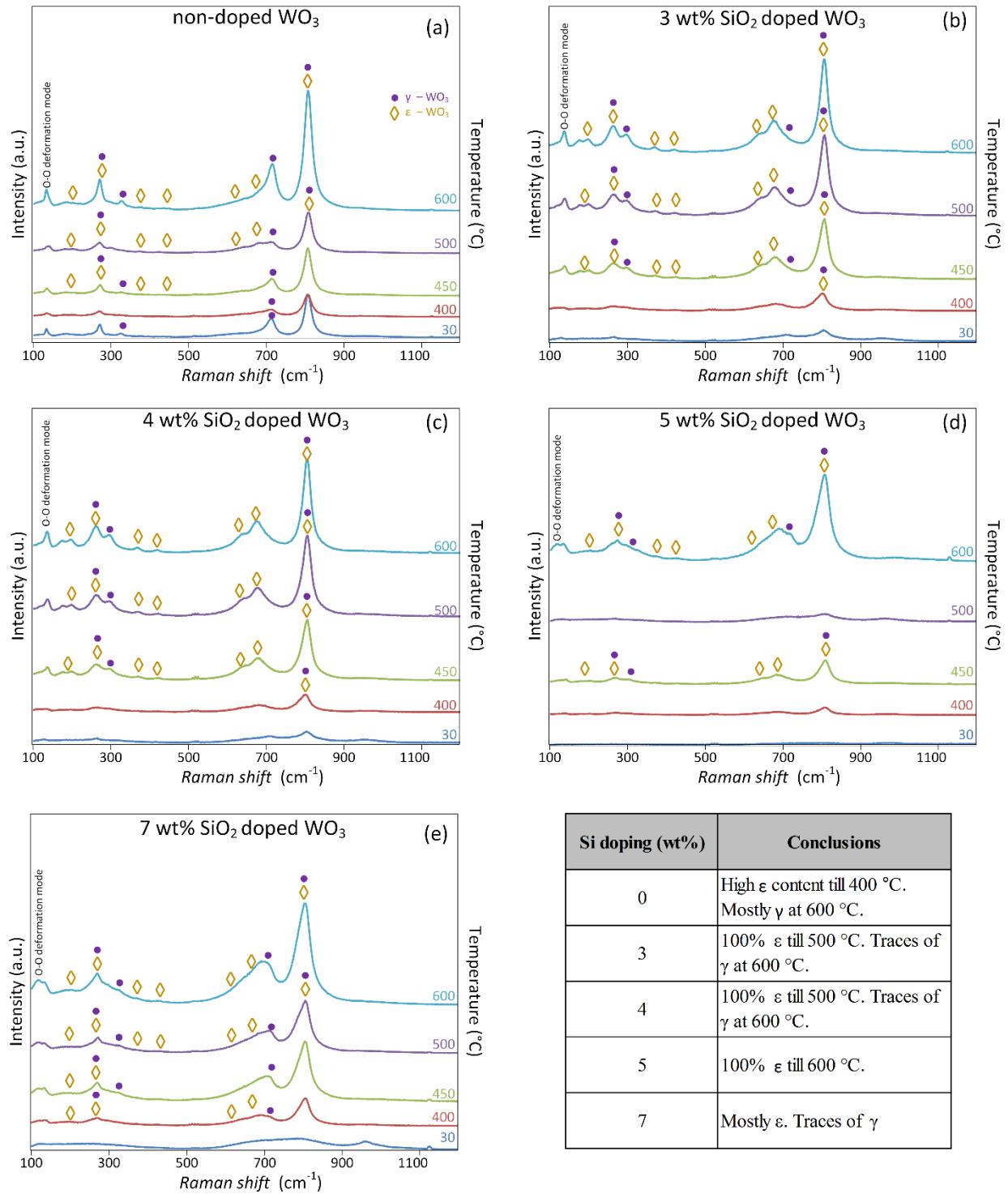
Fig. 8.6: (a)-(e) The Raman spectroscopy of the post annealed WO 3 film with 0%, 3%, 4%, 5%, and 7% SiO 2 respectively.
