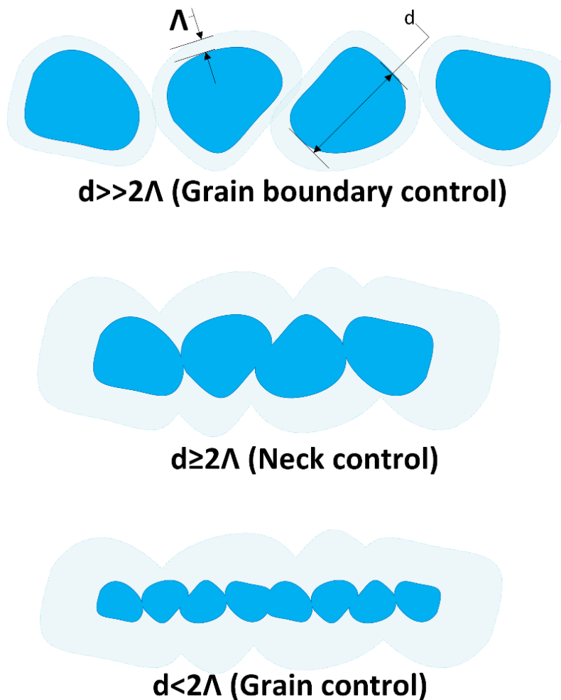
Fig. 3.4: Effect of grain size and necking in the electron depletion layer.
