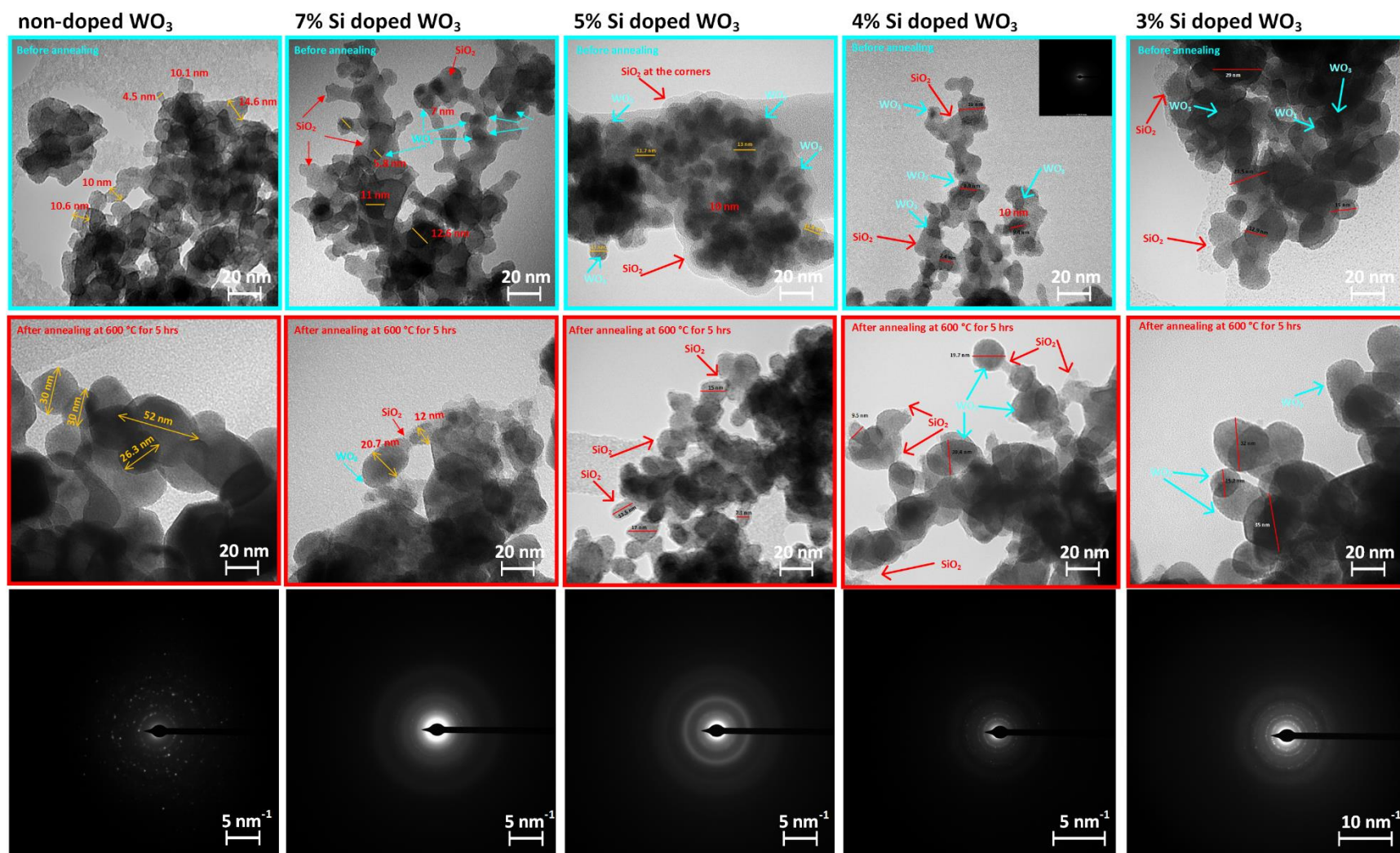
Fig. 8.8: (a)-(e) Transmission electron microscopy of the pre annealed and post annealed WO 3 film and the corresponding selected area diffraction pattern (SADP).
