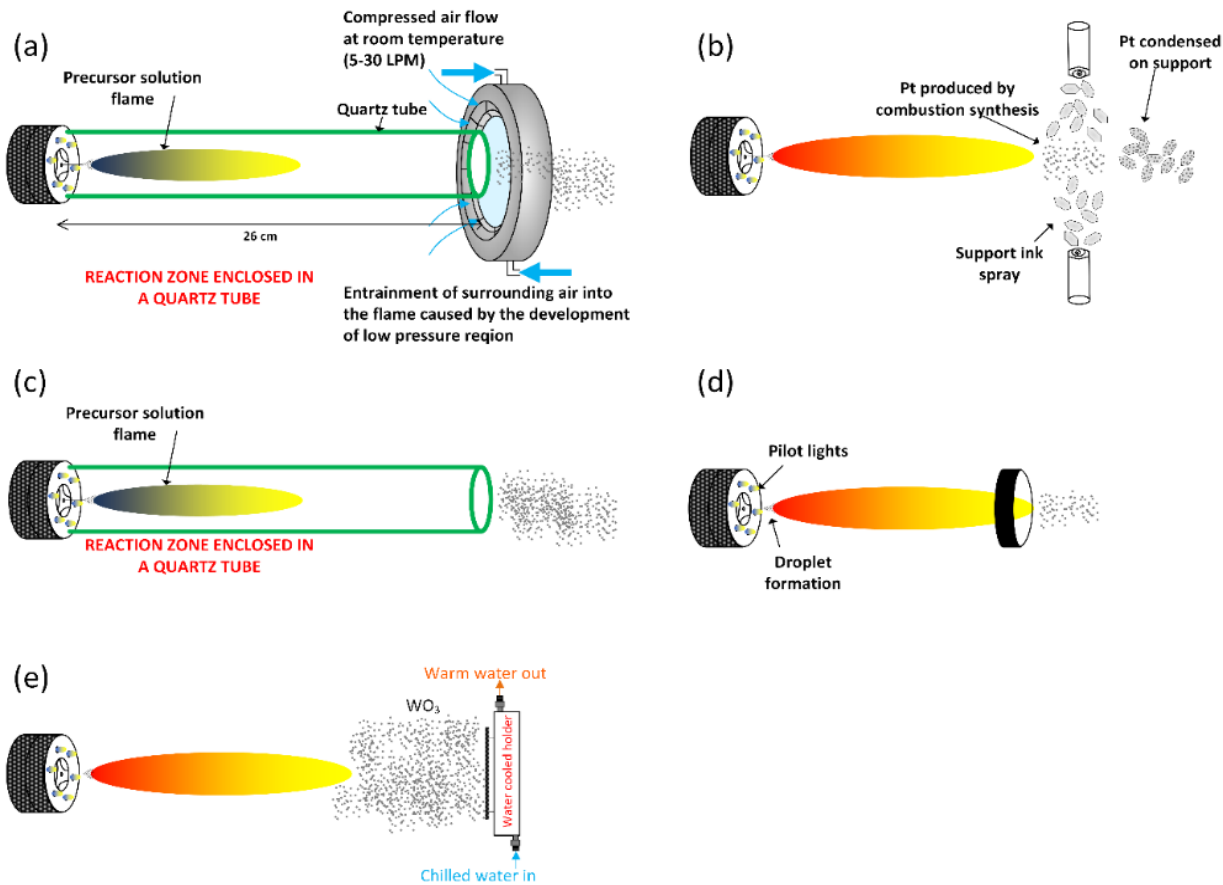
Fig. 1.5: Different configurations of RSDT: (a) for porous but micron size particles film, (b) use of secondary spray to deposited nanoparticles on support, (c) for dense film, (d) option to change the length of the reaction zone (distance between combustion nozzle and air quench), (e) deposition on a chilled substrate to enable the collection of nanopowder.
