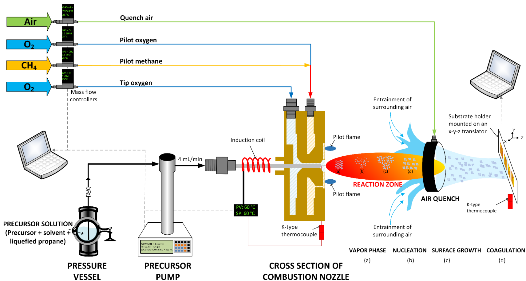
Fig. 9.1: Arrangement of the Reactive Spray Deposition Technology for direct deposition of \text{WO}_3 on gold interdigitated electrodes.
