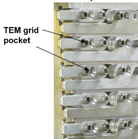
TEM grid holder for direct deposition
