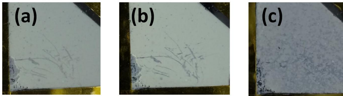
Fig. 8.12: 4 wt% SiO 2 doped WO 3 on a silicon substrate after annealing at 600°C. (a) initial film-(b) after impinging xylene based particle free frame for 60 s in RSDT, (c) after N 2 gas jet impingement test.
