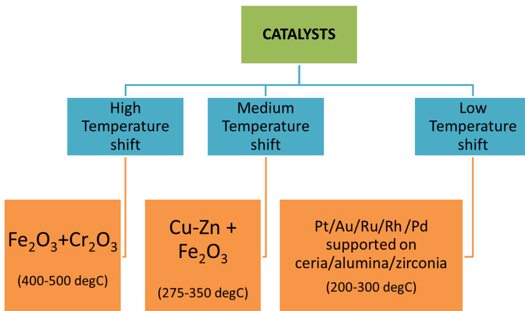
Fig. 2.2: Different types of water-gas shift catalysts and their temperature of operation.
