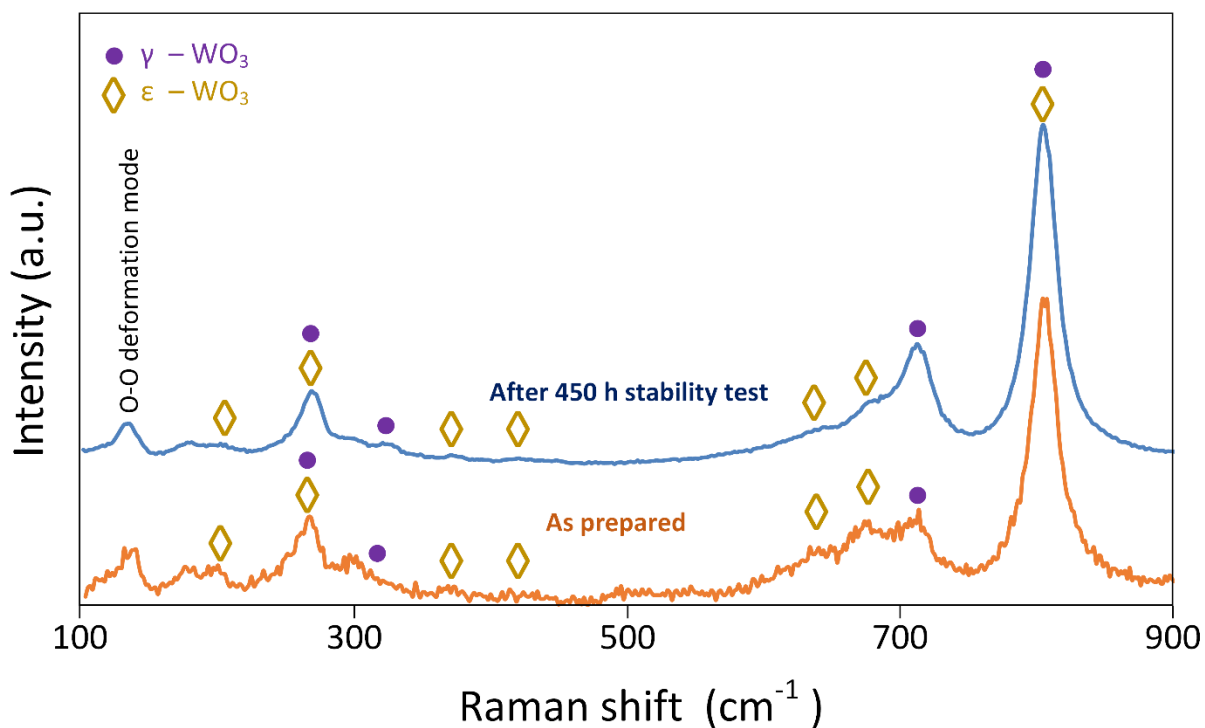
Fig. 10.5: Raman spectroscopy of the WO 3 film before and after the acetone sensing stability test.
