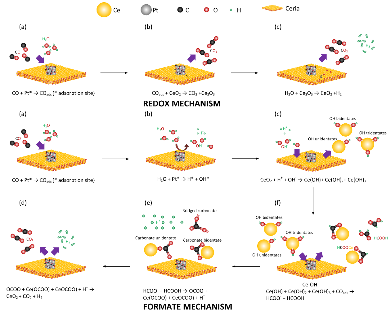
Fig. 2.4: Representation of the water-gas shift reaction redox mechanism on ceria/Pt catalysts shown in atomic scale.
