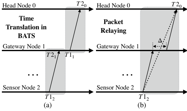
Fig. 1. Multi-hop extension based on (a) time translation proposed in BATS and (b) packet-relaying gateways.
