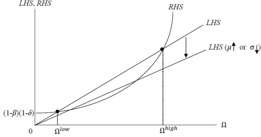
Figure 3b: Multiple equilibria under \alpha < 1/2 and a large \sigma
