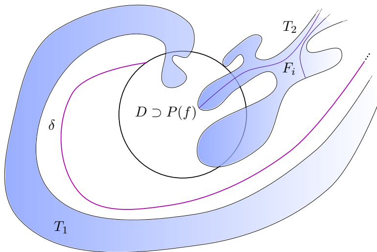
FIGURE 1. The dynamical plane for a function with two tracts. Some of the fundamental domains obtained by taking preimages of \delta are shown in one of the two tracts.
