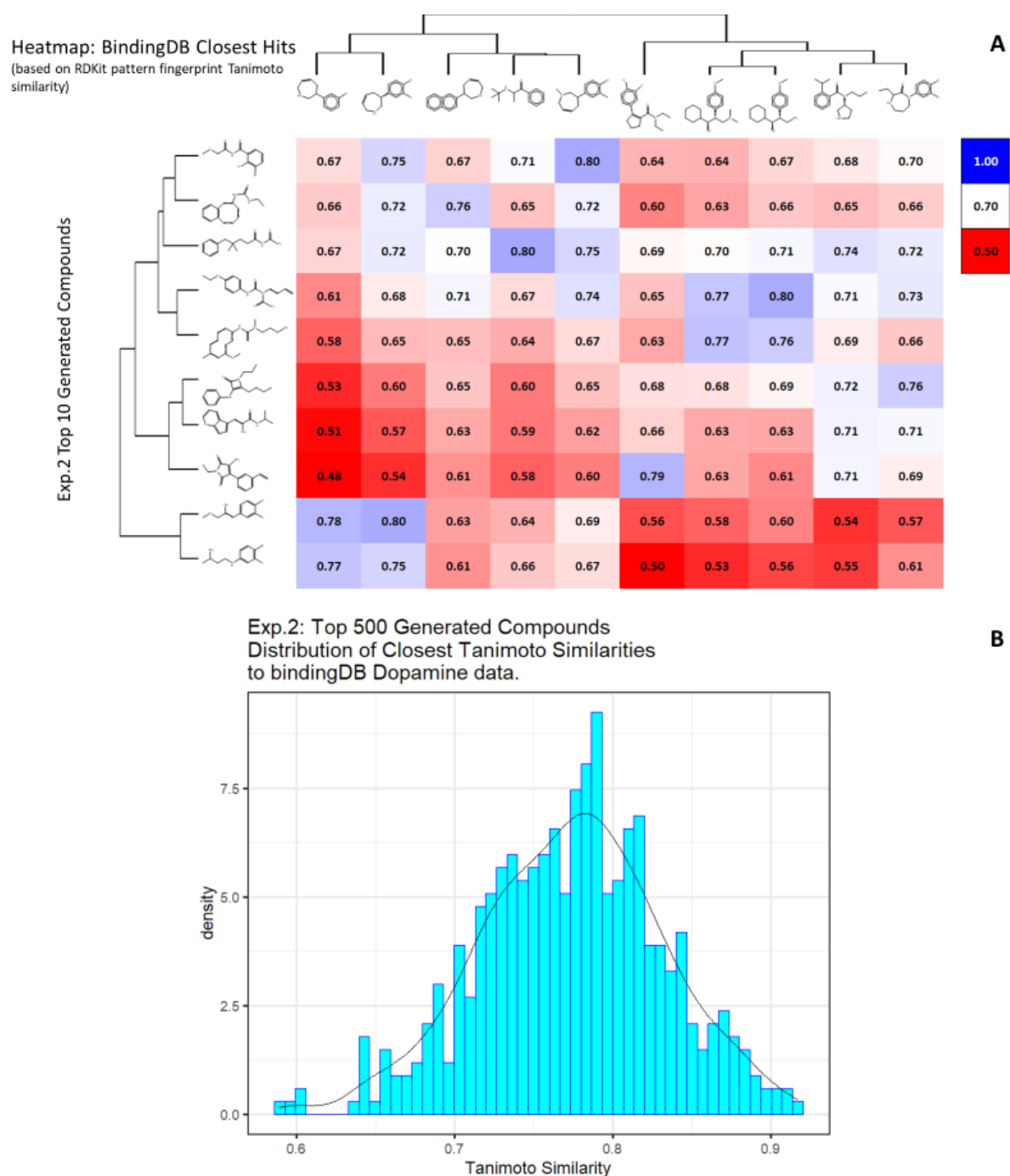
Figure 6. In silico generation by DeepGraphMolGen of novel molecules with predicted binding capacity to the dopamine transporter. Molecules were generated as described in the text. A. Top 10 molecules as predicted by DeepGraphMolGen versus the closest molecule in the BindingdB dataset and the Tanimoto similarity thereto (encoded using the RDKit patterned fingerprint). B. Distribution of Tanimoto similarities to a molecule in BindingdB dataset of the top 500 molecules.
