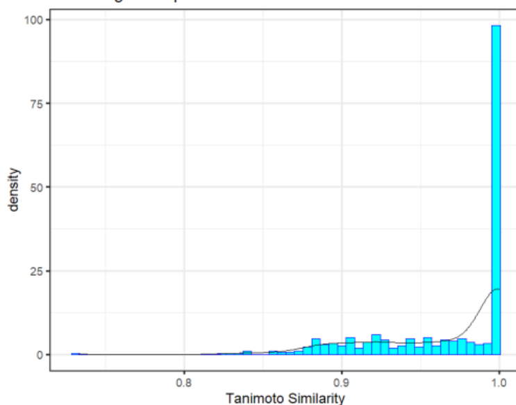
Exp.3: Top 500 Generated Compounds Distribution of Closest Tanimoto Similarities to bindingDB Dopamine data. B
