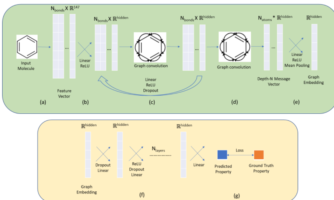
Figure 2. The property prediction pipeline for our method. The steps in green represent the feature extraction using Graph Convolution and the steps in orange represent regression of property scores. (a) The molecule is represented as a feature vector with features described as in section 2.1. (b) The feature vector is passed through a linear layer to get Depth-0 message. (c) Through repeated graph convolution (message passing) followed by Linear Layer, we get Depth N-1 message. (d) Each atom's final message is calculated by summing up the messages (also Graph Convolution) of the neighbouring atoms. (e) The resultant message is passed through a Linear Layer and the mean of all the atoms is taken to get the final embedding. (f) The property score is regressed from the graph embedding by a Feed Forward Neural Network. (g) The loss between predicted property and ground truth property is then backpropagated to change the weights.
