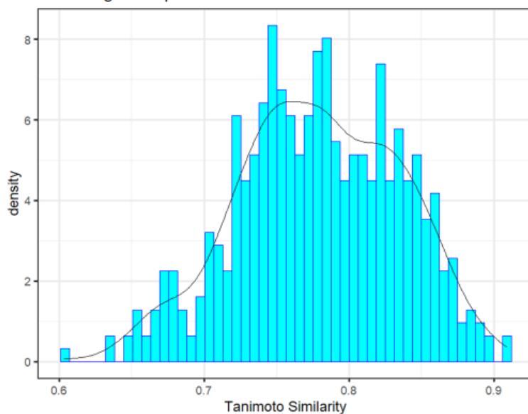
Exp.1: Top 500 Generated Compounds Distribution of Closest Tanimoto Similarities to bindingDB Dopamine data.
