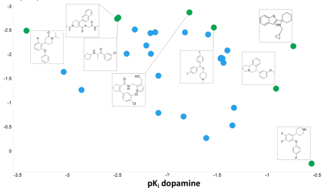
pK_i norepinephrine
