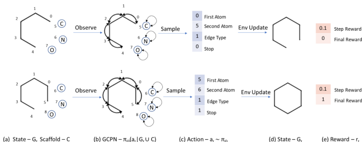
Figure 3. The reinforcement learning pathway for systemic generation of molecules (Redrawn from You et al. [34]). (a) The state is defined as the current graph G_t and the possible atom types C . (b) The GCPN conducts message passing to encode the state as node embeddings and estimates the policy function. (c) The action to be performed ( a_t ) is sampled from the policy function. The environment performs a chemical valency check on the intermediate state and returns (d) the next state G_t and (e) the associated reward ( r_t )
