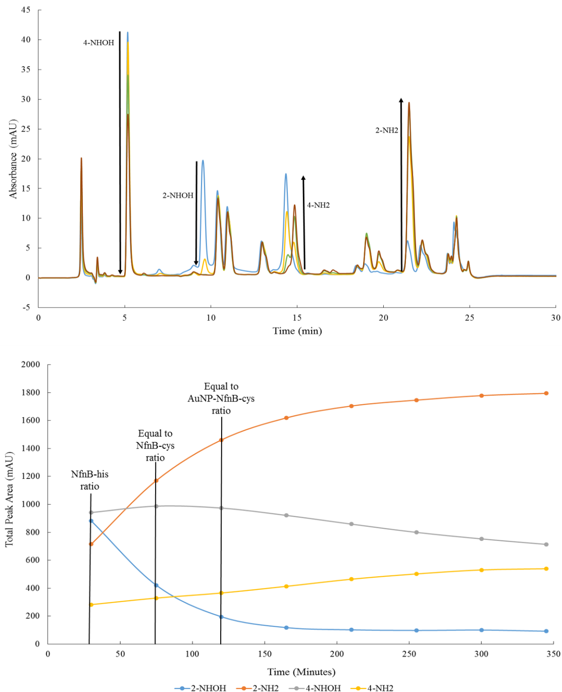
Figure 3. (Top) HPLC chromatogram of a reaction mixture in the presence of NfnB-his, measuring absorbance at 420 nm. The 4-hydroxylamine was detected at 5-6 minutes and the corresponding amine was detected at 14.5-15.5 minutes. The 2-hydroxylamine was detected at 9-10 minutes with the corresponding amine being detected at 21-22 minutes. (Bottom) A graph showing how each of the peak areas corresponding to the hydroxylamine and amine products changes over time as the reaction proceeds including labels of where the hydroxylamine ratio for NfnB-his matches those obtained for NfnB-cys and AuNP-NfnB-cys.
