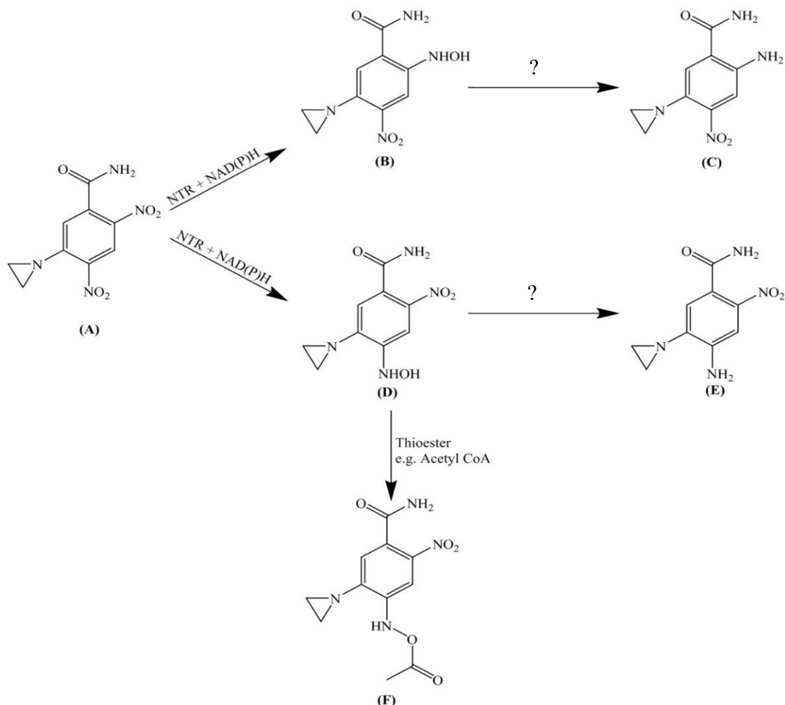
Figure 1. Figure adapted from the work done by P. Race et al. [21] showing the structure and reactions of CB1954 (A) with a nitroreductase enzyme and an NAD(P)H cofactor showing formation of the hydroxylamine derivatives (B) and (D) and the further reduction to the subsequent amine products over time (C) and (E) as well as the formation of the DNA cross-linking species (F) formed when the 4-hydroxylamine derivative is reacted with an intracellular thioester.
