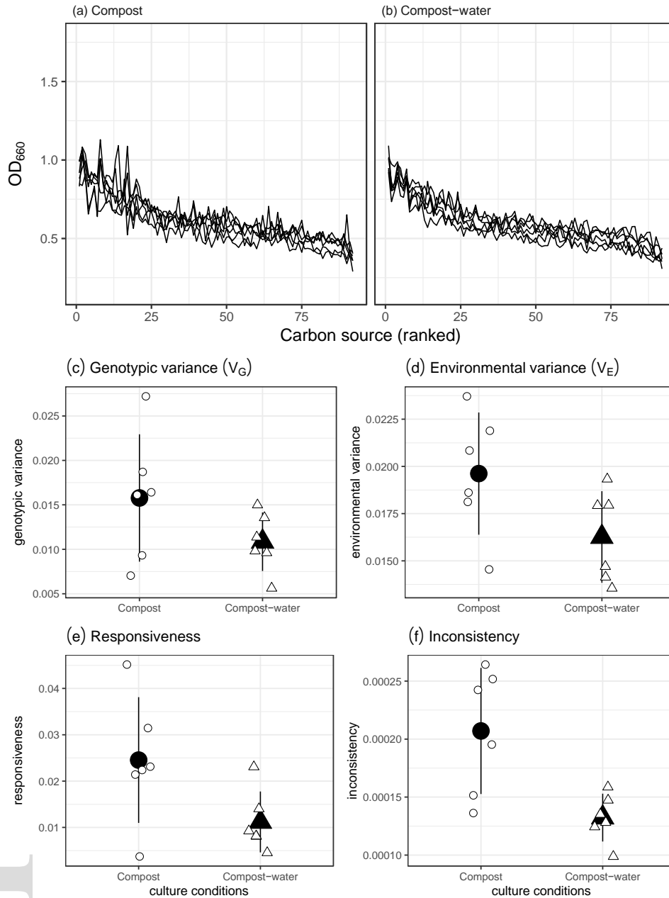
Figure 2. Catabolic profiles of populations evolved in either compost or compost-water. Performance of each clone evolved in either (a) compost or (b) compost-water on a variety of substrates. Total phenotypic variance was split into (c) genotypic variance (d) environmental variance and genotype x environmental components: (e) responsiveness and (f) inconsistency. Bacterial populations evolved in compost had higher inconsistency, indicating they had evolved to specialize on different resources. In (a,b), black lines represent the mean OD_{660} of each population (10 clones) and grey lines represent the performance of individual clones. In (c-f) Large black points are treatment means and error bars are the \pm of the standard deviation. Small white points are individual population values.
