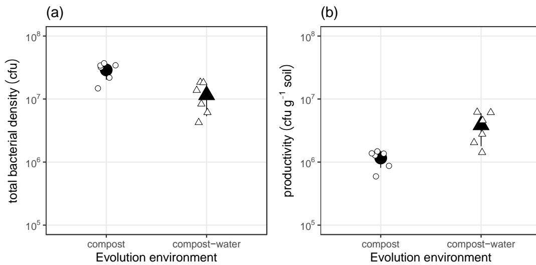
Figure 1. Bacterial densities of populations evolved in either compost or compost-water. (a) Total bacterial density was higher in the compost populations, but (b) density per unit compost (productivity) was higher in the compost-water populations. Points represent densities of each population (CFUs per gram of soil). Large black points are treatment means and error bars are the \pm of the standard deviation. Small white points are individual population values.
