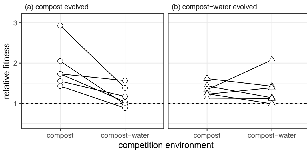
Figure 3. Relative fitness of populations evolved in either compost or compost-water. Points represent the relative fitness of each population. Lines show the links between each evolved population in each of its competition environments.
