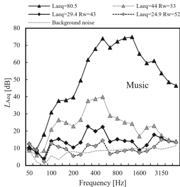
Figure 1 - Frequency characteristics of noise stimuli.
