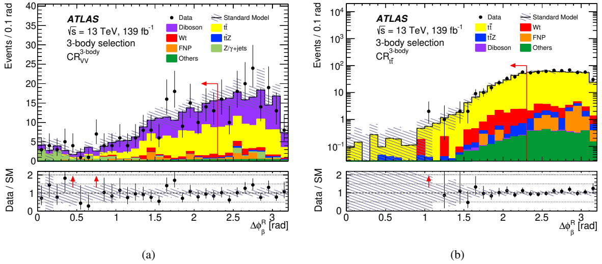
Figure 4: Three-body selection. Distributions of (a) \Delta\phi_\beta^R in the CR_{VV}^{3\text{-body}} selection, and (b) in the CR_{t\bar{t}}^{3\text{-body}} selection, after the background fit. The contributions from all SM backgrounds are shown as a histogram stack. “Others” includes contributions from VVV , t\bar{t}t , t\bar{t}t\bar{t} , t\bar{t}W , t\bar{t}WW , t\bar{t}WZ , t\bar{t}H , and tZ processes. The hatched bands represent the total statistical and detector-related systematic uncertainty. In the upper panels, red arrows indicate the control region selection criteria. The bottom panels show the ratio of the observed data to the total SM background prediction, with hatched bands representing the total uncertainty in the background prediction; red arrows show data outside the vertical-axis range.
