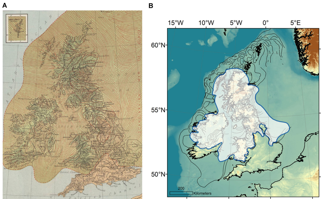
Figure 1. Three depictions of the extent of the British–Irish Ice Sheet. (A) Geikie (1894) used a small amount of evidence along with some large conjecture to reconstruct the ice sheet reaching the edge of the continental shelf and being confluent with Scandinavian ice over the North Sea. (B) By the 1980s, accumulation of substantial amounts of evidence from glaciogenic sediments and landforms, and less use of conjecture, led to a much smaller ice sheet being reconstructed, summarised here (blue line) by Bowen et al. , (1986). In the 21st century, data collected by ship-borne geophysics allowed widespread observations of seafloor moraines and grounding lines and that overturned the small-ice model (black lines show ice extent and retreat, modified from Clark et al. , 2012). Reconstructions returned to the large-ice model and confluence with the Scandinavian Ice Sheet. This retreat pattern, however, had much uncertainty about timing, which glacial stage was represented and rates of retreat; these uncertainties provided the motivation for BRITICE-CHRONO and this special issue. [Color figure can be viewed at wileyonlinelibrary.com ]
