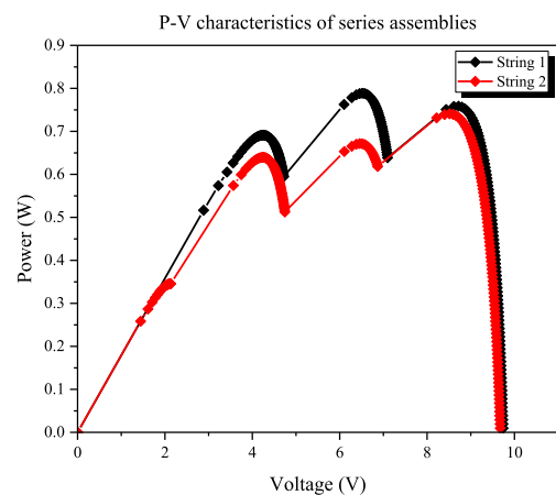
FIGURE 11. The 2 × 4 PV modules output characteristics of I-V and P-V before reconfiguration.
