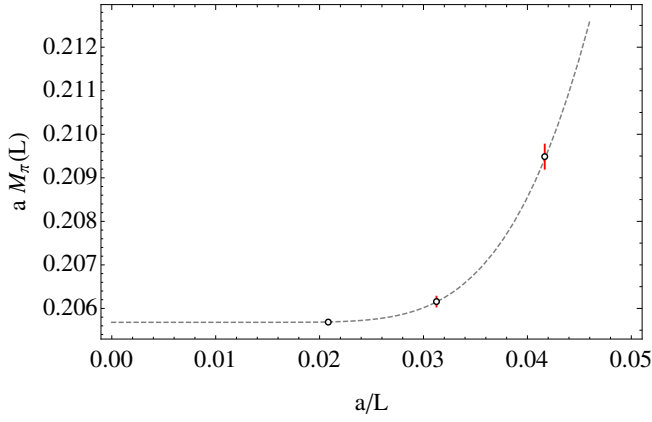
FIG. 2. Dependence of the PGNB mass aM_\pi on the inverse of the spatial extent of the lattice L for the fermion mass am = 0.0075 . The gray line shows the L -dependence predicted by the model in Eq. (14), using the best fit values for the parameters \alpha and \beta indicated in Eq. (16). For the range of lattice volumes for which we have data, the finite-volume correction to aM_\pi is clearly significant.
