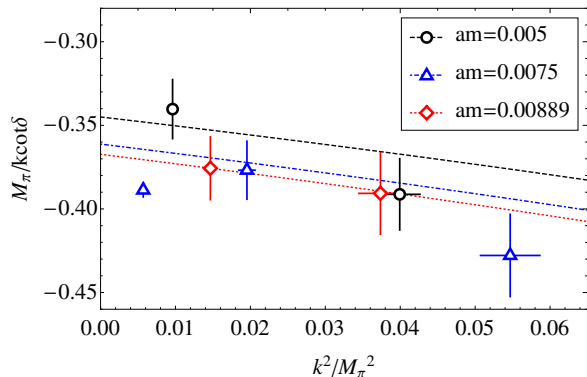
FIG. 1. Plot showing the variation of the scattering phase shift with scattering momentum for the three largest fermion masses. The points indicate the lattice data, given in Table II, whereas the lines represent tree level dilaton EFT predictions, as explained in Section III.
