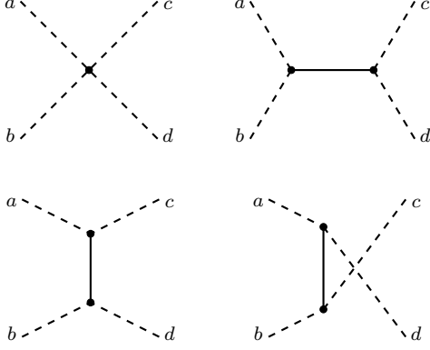
FIG. 4. Feynman diagrams in dilaton EFT which appear in the \pi - \pi scattering amplitude at tree level. The dashed lines represent PNGBs and the solid lines represent the dilaton.
