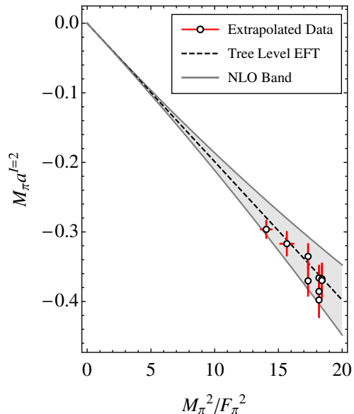
FIG. 5. Points representing the scattering lengths determined from lattice data are plotted against the finite-volume extrapolated quantity M_\pi^2/F_\pi^2 . They are compared with the tree level dilaton EFT prediction given in Eq. (32), and shown here as the straight black dashed line. The central values from the global fit are inputted to obtain this dependence. The gray band plotted around the dashed line represents the plausible range of corrections to the EFT prediction which could occur at NLO, and is given by Eq. (34).
