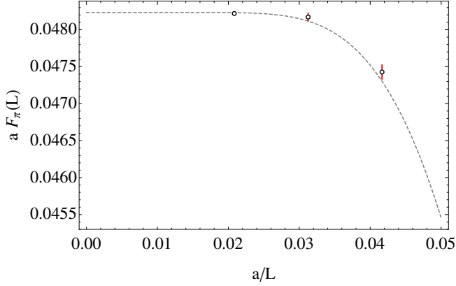
FIG. 3. Dependence of the PGNB mass aF_\pi on the inverse of the spatial extent of the lattice L for the fermion mass am = 0.0075 . The gray line shows the L -dependence predicted by the model in Eq. (15).
