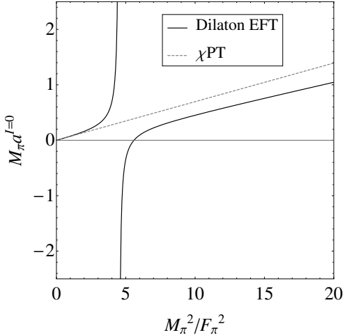
FIG. 6. The prediction for the scattering length in the I = 0 channel, obtained using tree level dilaton EFT from Eq. (35), and the global fit central values is shown here as the black solid line. The gray dashed line representing the prediction from tree level chiral perturbation theory is shown for comparison.
