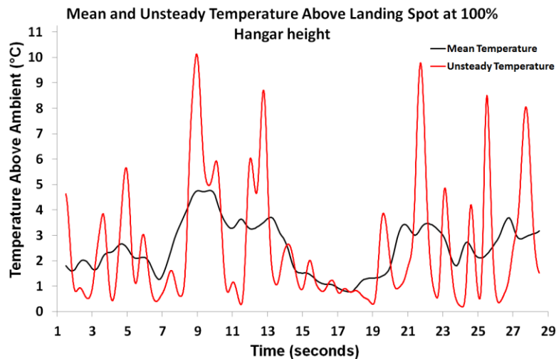
Figure 25 CFD-predicted air temperatures above landing deck – Instantaneous and 3-second average
