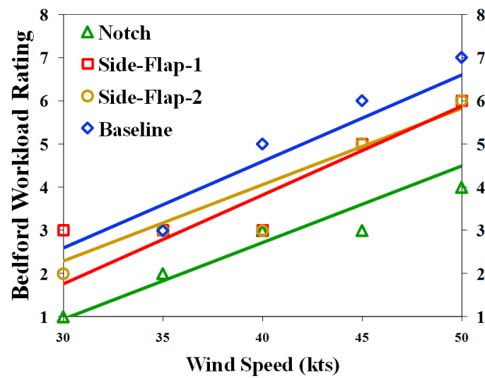
Figure 17 Pilot workload ratings for 30 second hover over landing spot in Green 45° winds
