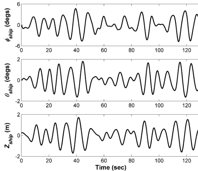
Figure 9 Example of simulated ship motion in sea state six conditions measured at the ship's centre of gravity
