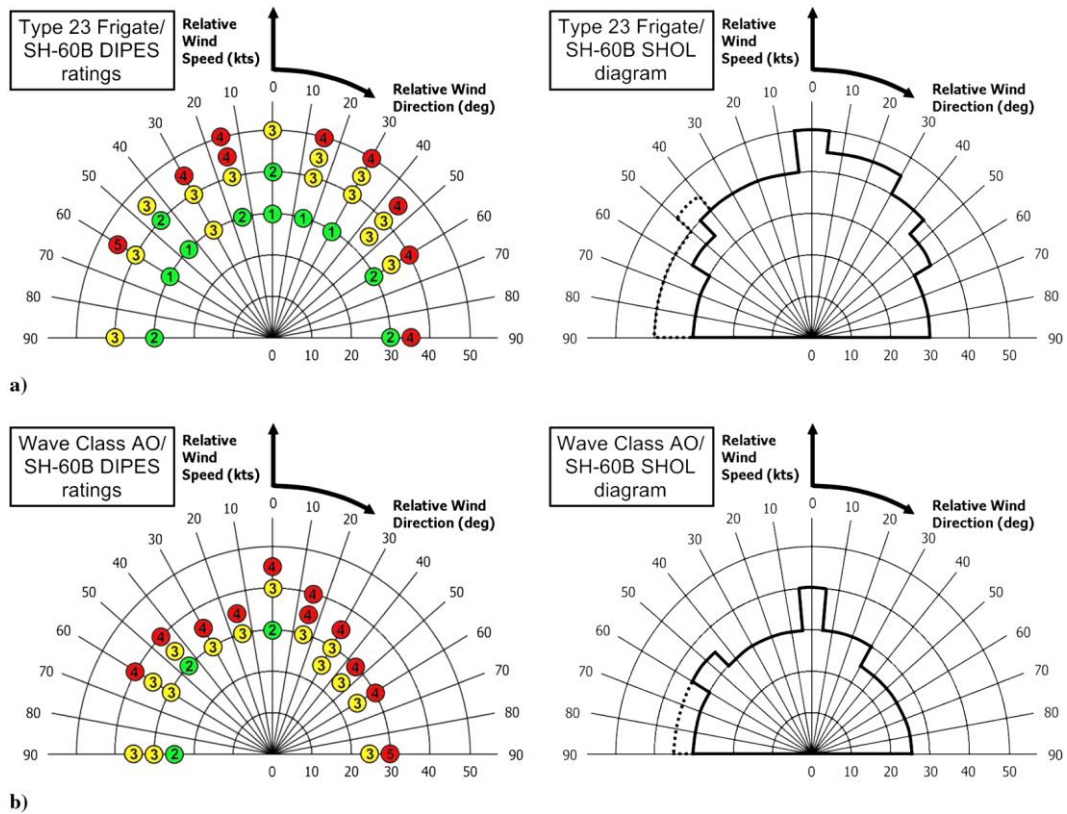
Figure 13 DIPES Ratings and SHOL Diagrams for a Type 23 Frigate and Wave Class tanker.
