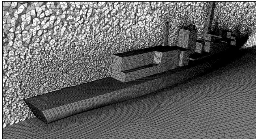
Figure 7 Unstructured CFD mesh for Type 23 frigate
