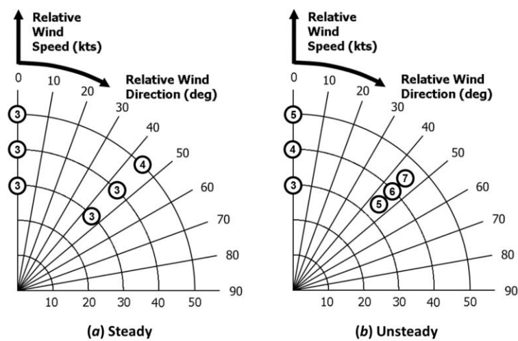
Figure 11 Bedford workload ratings for a station-keeping task in steady and unsteady airwakes.
