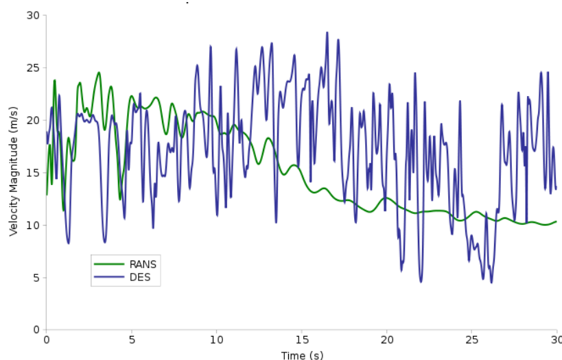
Figure 6 Time history of velocity at a point in the flow above the flight deck using URANS and DES
