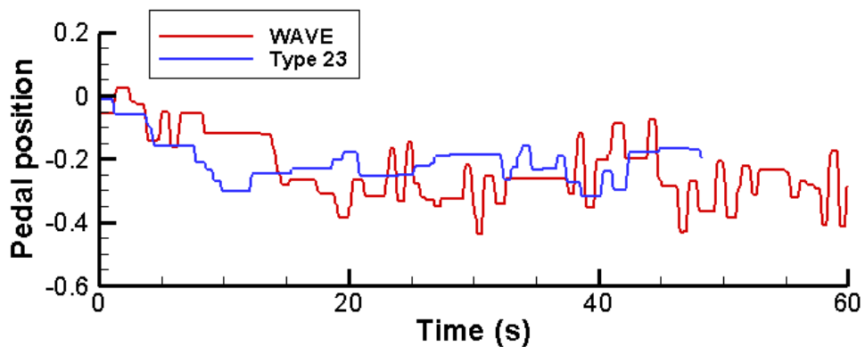
Figure 14 Pilot pedal activity (+1 to -1) in the simulator while station-keeping above the landing spot of a Wave Class Tanker and a Type 23 frigate in a Green 45 wind
