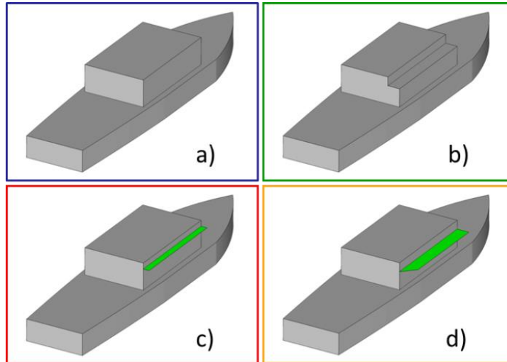
Figure 16 Simplified ship; a) Baseline; b) Notch; c) Side-Flap1; d) Side-Flap 2
