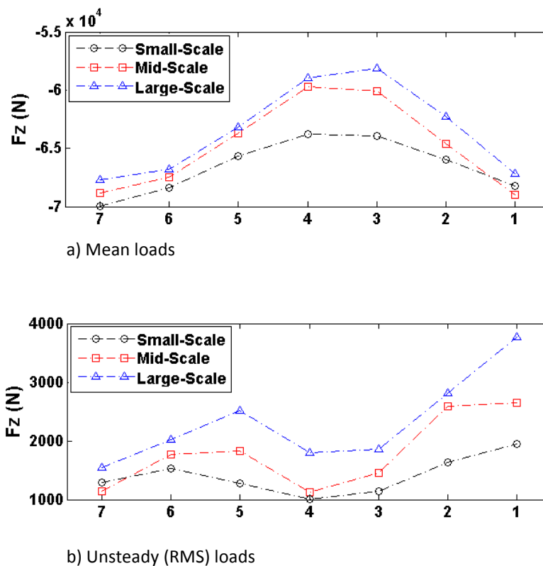
Figure 19 Mean and RMS helicopter loads in ship airwakes measured by the Virtual AirDyn
