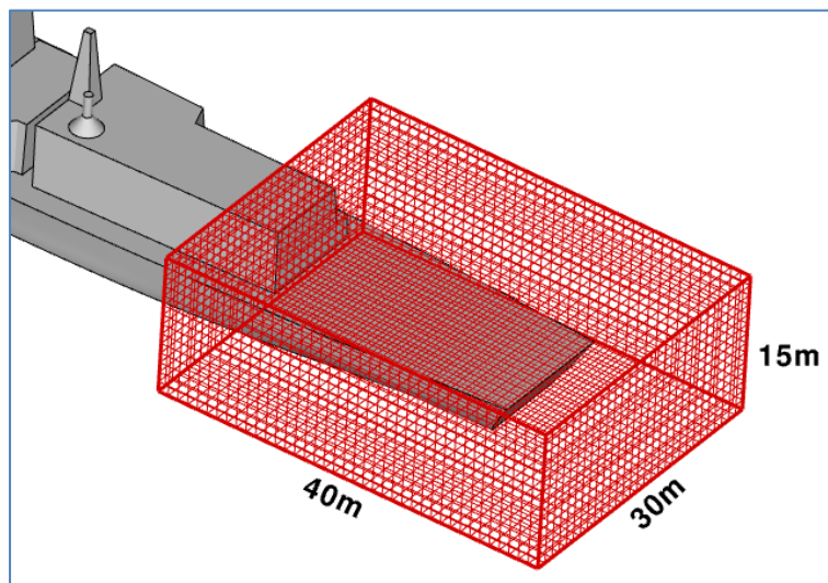
Figure 8 Structured grid for airwake lookup table
