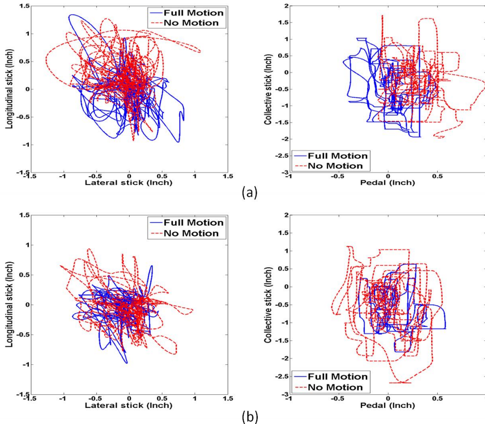
Figure 12 Pilot control activity in (a) daylight and (b) fog, with and without motion.
