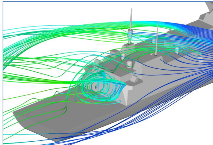
Figure 20 Virtual AirDyn assessment of future frigate superstructure aerodynamics
