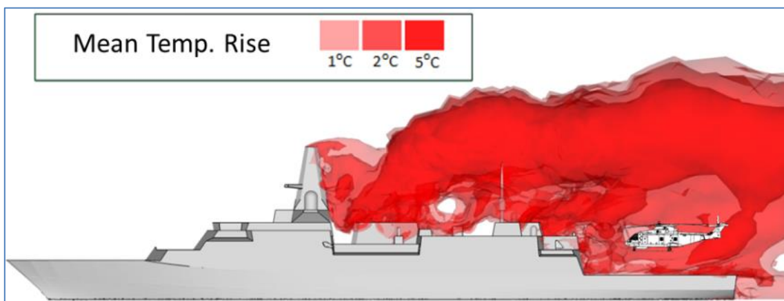
Figure 24 Instantaneous iso-surfaces of unsteady ship exhaust plume temperatures
