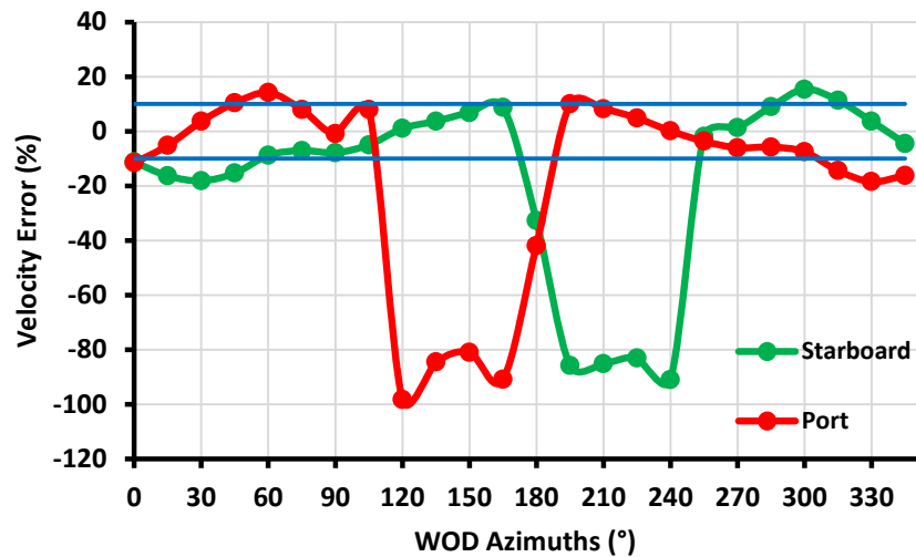
Figure 22 Predicted percentage deviation of wind speed at anemometer locations
