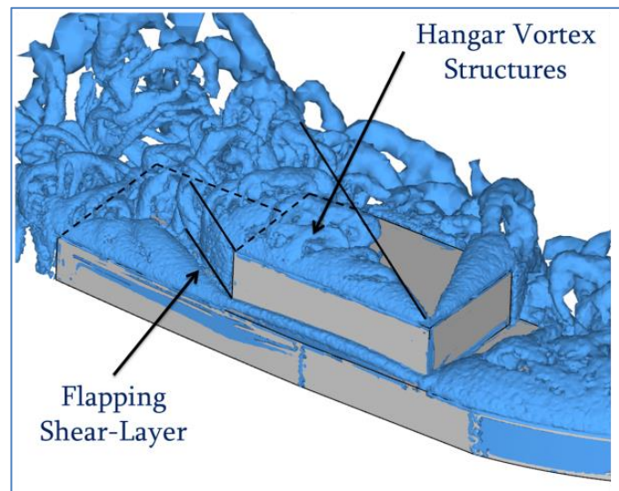
Figure 15 Visualisation of air flow over a simplified ship in oblique 45^\circ winds by surfaces of iso-vorticity
