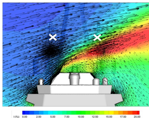
Figure 21 Contours of turbulence intensity with velocity magnitude vectors in a 40 kt 90° beam wind
