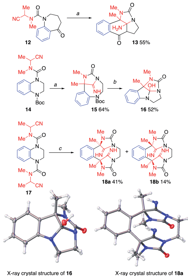
Scheme 5 Ring-expansion of substituted tetrahydroquinolines. Conditions: a (1) KHMDS (2 equiv.), THF, 0 °C, 1–1.5 h; (2) MeOH; b 2 M HCl : MeOH (1 : 1), reflux, 44 h. c (1) KHMDS (4 equiv.), THF, 0 °C, 5 h. (2) MeOH. CCDC deposition numbers for X-ray data: 16 1993733; 18a 1993734.†
