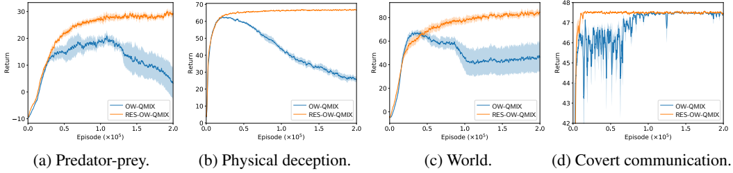
Figure 21: Performance comparison of Weighted QMIX and RES-Weighted QMIX.
