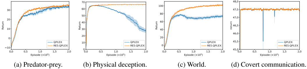
Figure 22: Performance comparison of QPLEX and RES-QPLEX.
