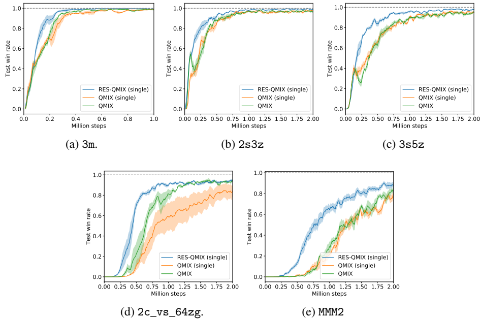
Figure 25: Performance comparison of RES-QMIX (single), QMIX (single), and QMIX.
