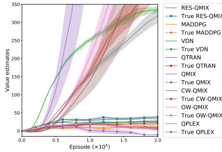
Figure 18: Comparison of true values and estimated values of different algorithms in predator-prey.
