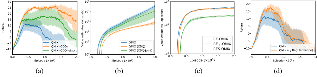
Figure 10: (a) and (b) Comparison of performance and value estimates of QMIX (CDQ) and QMIX (CDQ-joint). (c) Value estimates (in log scale) of RE-QMIX, RE + -QMIX, and RES-QMIX. (d) Performance comparison of QMIX and QMIX ( L_2 Regularization).
