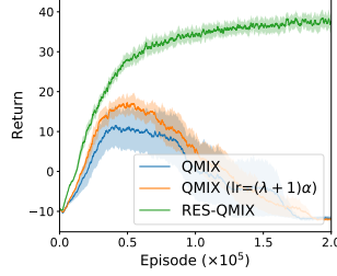
Figure 13: Comparison results of QMIX, QMIX (lr=( \lambda + 1 ) \alpha ), and RES-QMIX.
