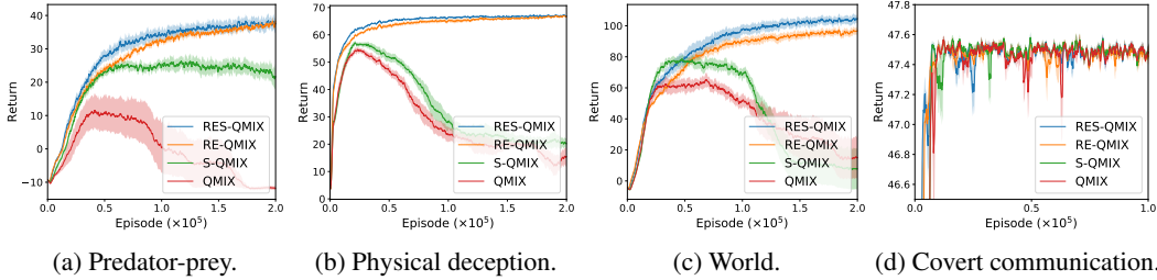
Figure 19: Ablation study of the effect of each component.
