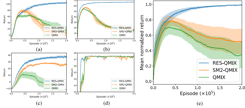
Figure 23: Performance comparison of RES-QMIX, SM2-QMIX and QMIX. (a) Predator-prey. (b) Physical deception. (c) World. (d) Covert communication. (e) Mean normalized return.
