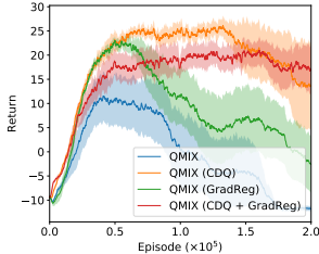
Figure 2: Return of QMIX and its variants in the predator-prey environment.
